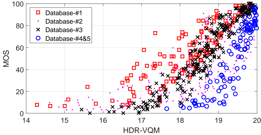
Figure 4.2 – MOS vs HDR-VQM scores before INLSA alignment.
