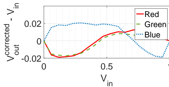
(c) Deviation for each color channel
