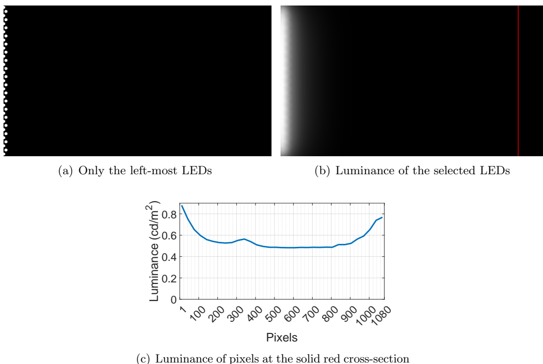
Figure A.5 – Figures of a measurement test where (a) only the left-most LEDs are selected. The (b) luminance of the selected LEDs were measured following the solid-red line. (c) The measured luminance values for the solid-red cross-section show that the edges of the display has more light compared to the center part.
