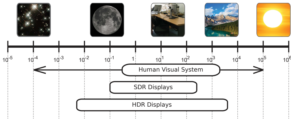
Figure 1.1 – Comparison of SDR and HDR display systems with respect to the real world luminance values and to the capabilities of human visual system. (Values of the scale are in \text{cd/m}^2 .)
