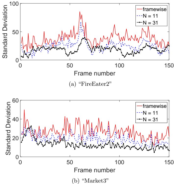
Figure 2.8 – Standard deviation change with respect to frame number for (a) “FireEater2” and (b) “Market3” sequences
