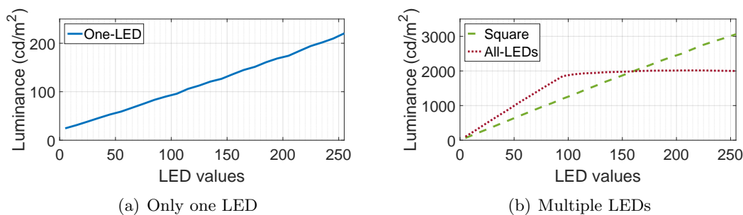
Figure A.2 – Plots of the measured luminance with respect to the LED value for the case of (a) only one LED and (b) multiple LEDs. The plots show a linear (or close to piecewise linear in the case of all LEDs) relationship between the LED values and the emitted luminance. Since the scale of luminance values are not comparable in the case of only one LED and multiple LEDs, they are presented in different sub-figures.
