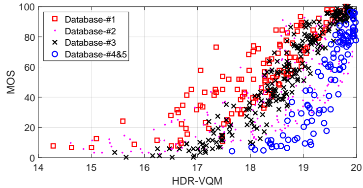
(a) HDR-VQM - Before INLSA (RMSE = 44.10)
