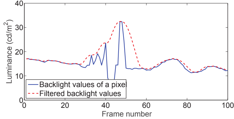
Figure 2.4 – Example of temporal smoothing of backlight pixel trajectories for the “ChristmassTree” video sequence.
