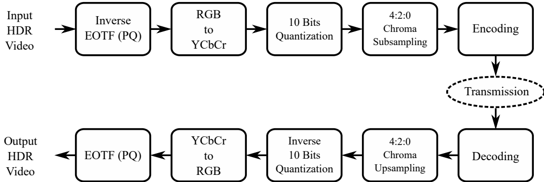
Figure 1.2 – HDR video compression pipeline as described in MPEG CFe [LFH15], and standardized in ITU-R BT.2100 [ITU17b]
