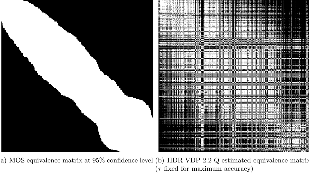
Figure 4.7 – Equivalence maps for the (sorted) combined database. White entries correspond to S(I_i) \cong S(I_j) , black to S(I_i) \not\cong S(I_j) .
