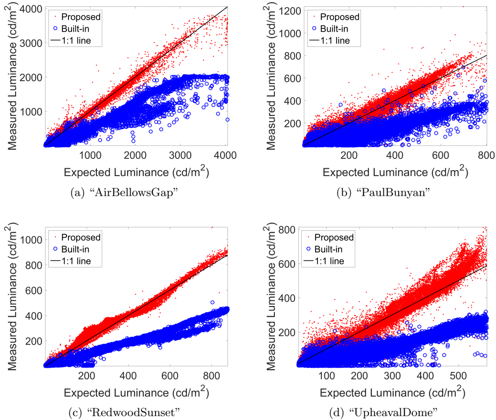
Figure 2.6 – Plots of measured luminance vs. expected luminance
