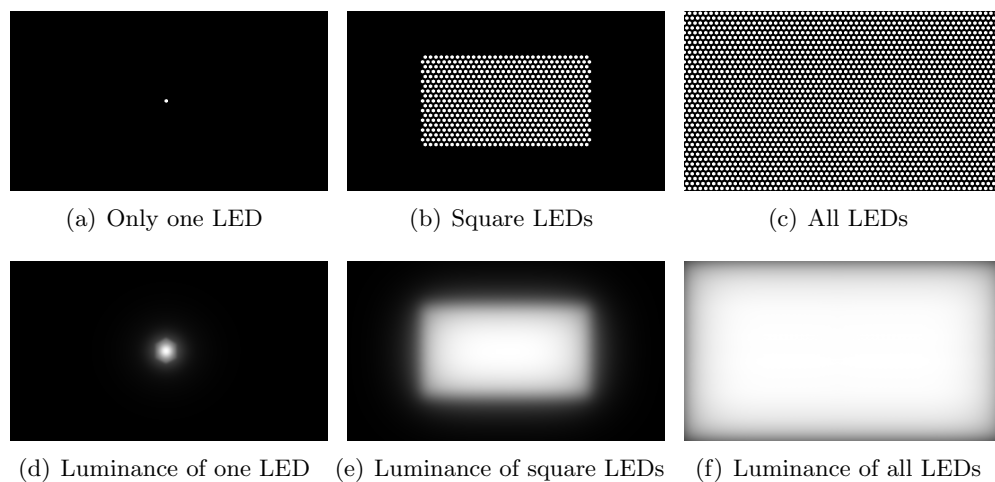
Figure A.1 – Test patterns created for LED measurements for three different cases using (a) only one LED, (b) a collection of LEDs that covers 30% of the display area, and (c) all the LEDs of the backlight layer. LCD values for these test patterns were set to 255 in order to ensure that all of the backlight passes the LCD layer. Estimated luminance values (presented in (d)-(f)) were normalized for representation. The emitted luminance values were measured at the center of the display for each case.
