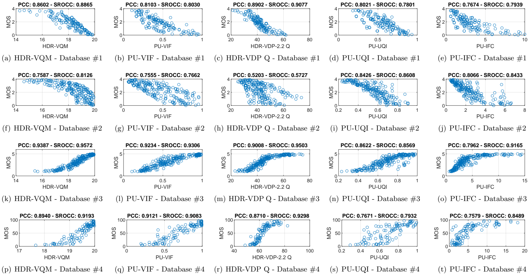
Figure 4.3 – Plots of MOS vs objective quality scores for the selected objective metrics selected showing the linearity of the metric estimations
