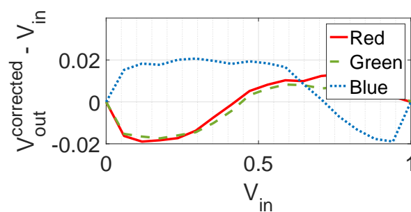
(c) Deviation for each color channel
