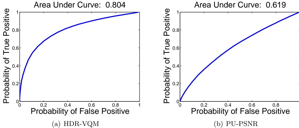
Figure 4.8 – Example of ROC curves for two objective quality metrics, with corresponding area under the curve (AUC). Metrics with higher AUC enable better discrimination between the two hypotheses \mathcal{H}_0 and \mathcal{H}_1 .
