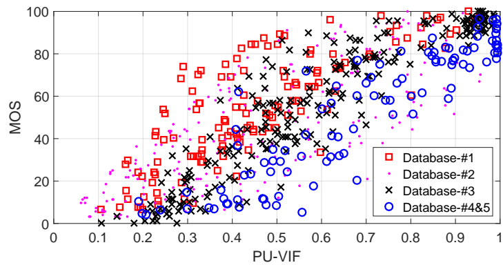
(c) PU-VIF - Before INLSA (RMSE = 59.27)
