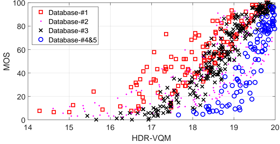
Figure 4.2 – MOS vs HDR-VQM scores before INLSA alignment.
