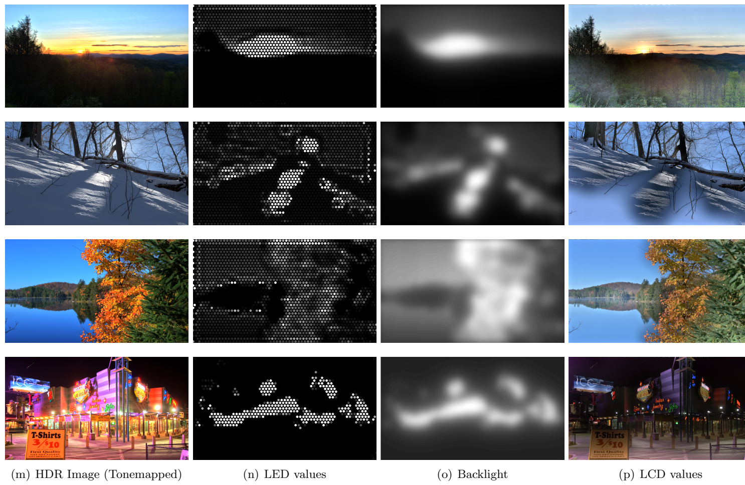
Figure 2.3 – Examples of tonemapped HDR images, LED values, backlights, and LCD values of HDR images (top to bottom) “AirBellowsGap”, “DevilsBathtub”, “MasonLake(1)”, “LasVegasStore”
