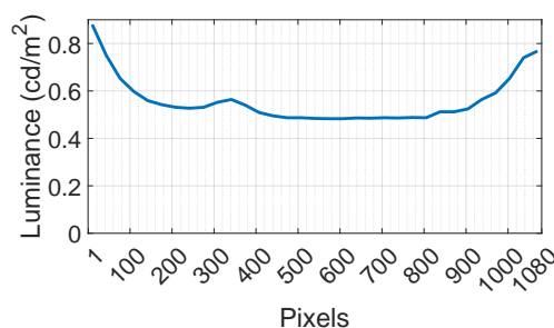
(c) Luminance of pixels at the solid red cross-section
