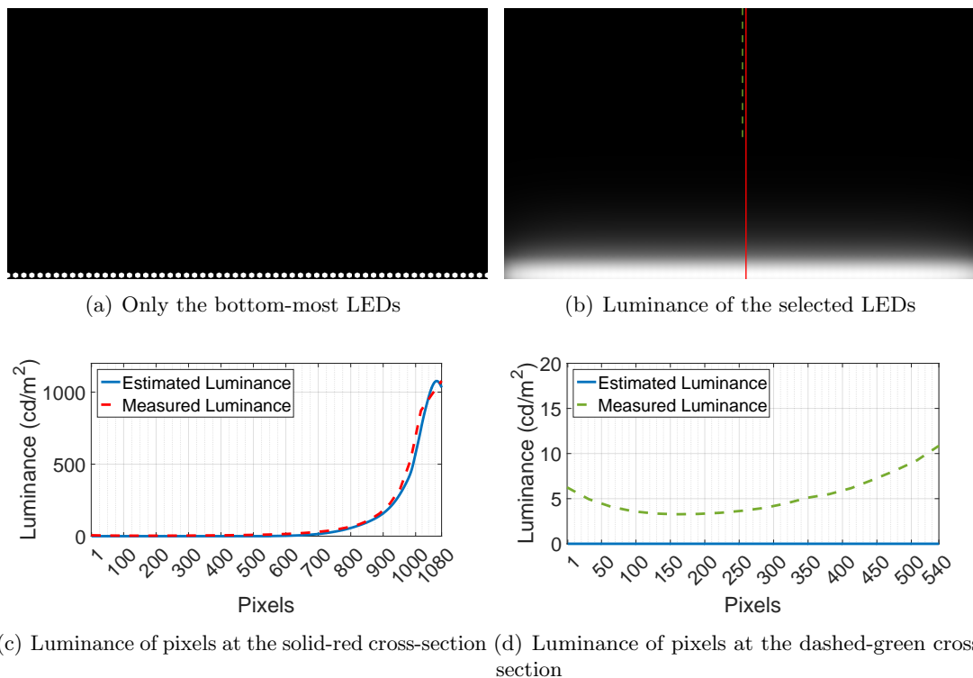
Figure A.4 – Figures of a measurement test where (a) only the bottom-most LEDs were selected. The (b) luminance of the selected LEDs were measured following the solid-red and dashed-green lines. (c) The measured luminance values for the solid-red cross-section are in agreement with the estimated luminance values, and it shows that the estimation of the developed algorithm is accurate. However, (d) the measured luminance values for the dashed-green cross-section reveals a strange phenomenon. The luminance values increase as we move away from the light source and get closer to the edge.
