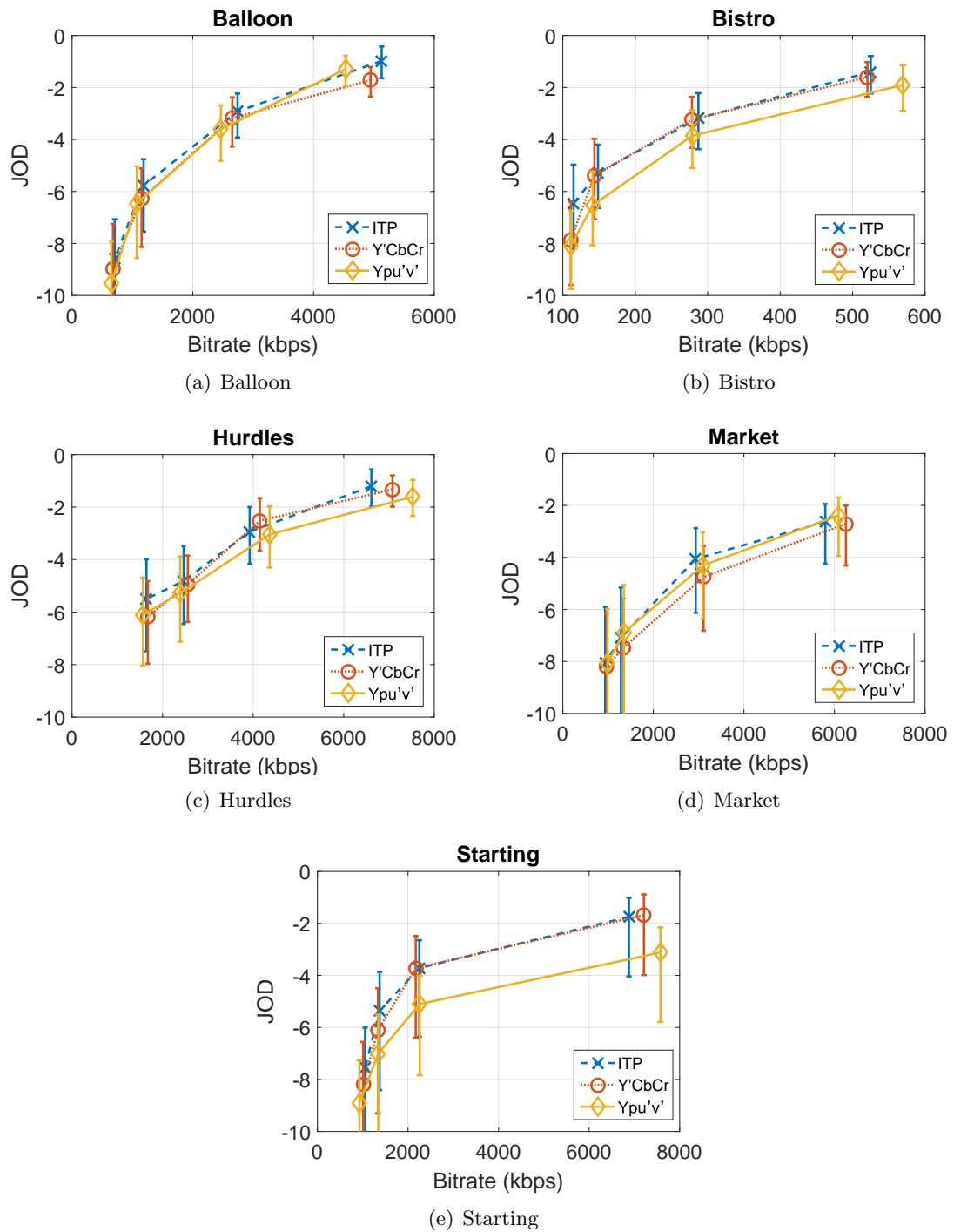
Figure 3.7 – Image scores obtained by scaling preferences to relative quality distances (in JOD units) for the three tested color spaces.
