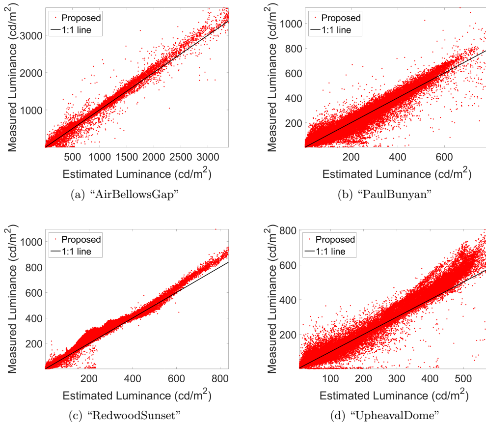
Figure 2.7 – Plots of measured luminance vs. estimated luminance. These results are presented only for the proposed rendering.
