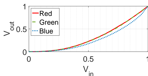
(a) The relationship between V_{in} and V_{out} for each color channel
