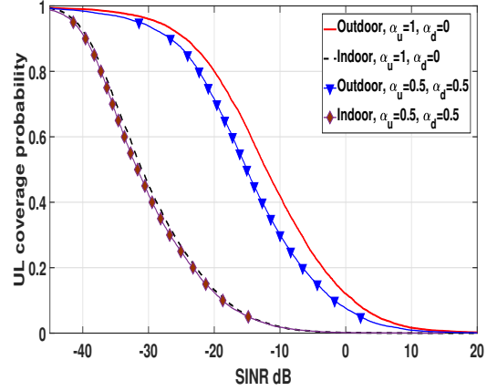
Figure 3.11 – Small-cells UL coverage probability : 2b = 3.5 , k = 0.4 and \lambda = 10 small-cell/ km^2 .
