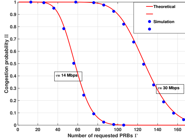
Figure 6.3 – Congestion probability theoretical vs simulation for two values of \tau
