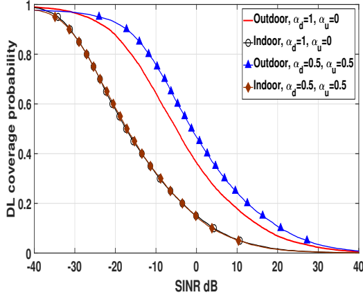
Figure 3.10 – Small-cells DL coverage probability : 2b = 3.5 , k = 0.4 and \lambda = 10 small-cell/ km^2 .
