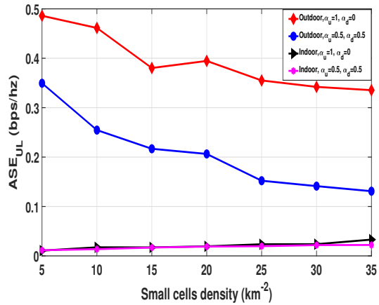
Figure 3.13 – UL average spectral efficiency : 2b = 3.5 , k = 0.4 .
