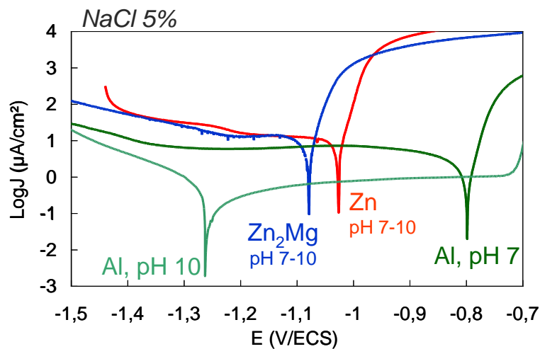
Figure 9: Polarization curves of Zn, Al and Zn_2Mg at pH ranging from 7 to 10 in NaCl 5wt. % (from [43]).
