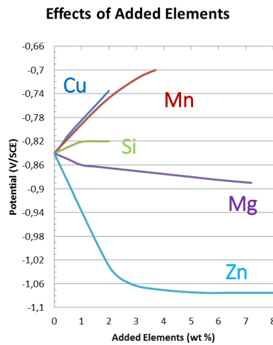
Figure 7 : Alloying elements influence on the dissolution potential of aluminum alloys in ASTM G69. (from [29])
