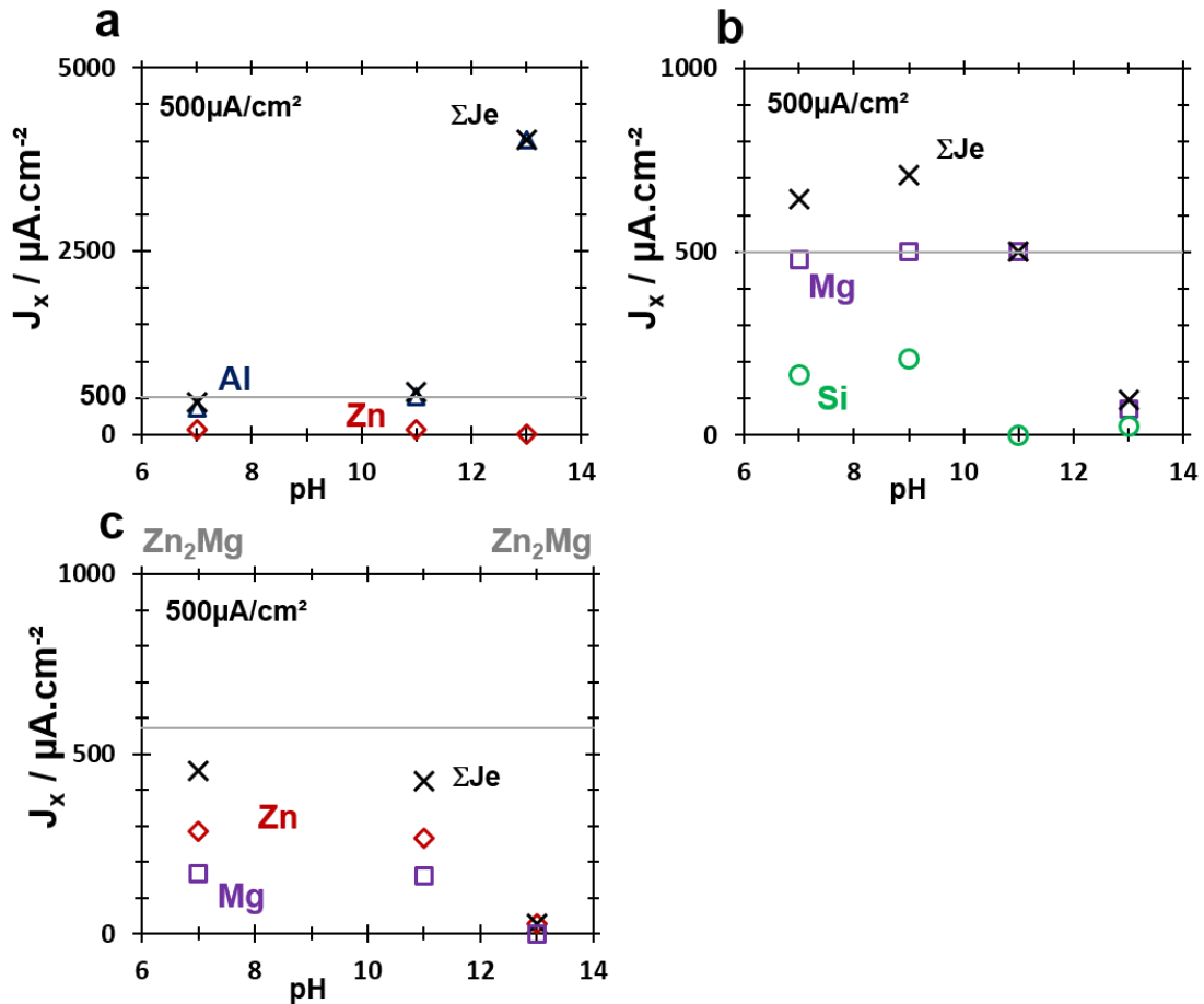
Figure 8 : Effect of pH on the elemental dissolution currents J_x ( x=Al, Zn, Mg, \text{ and } Si ) for (a) Al(Zn32), (b) Mg_2Si , (c) Zn_2Mg dissolving in 0.172 M NaCl aqueous solution with different pH under imposed anodic current of 500 \mu A.cm^{-2} .
