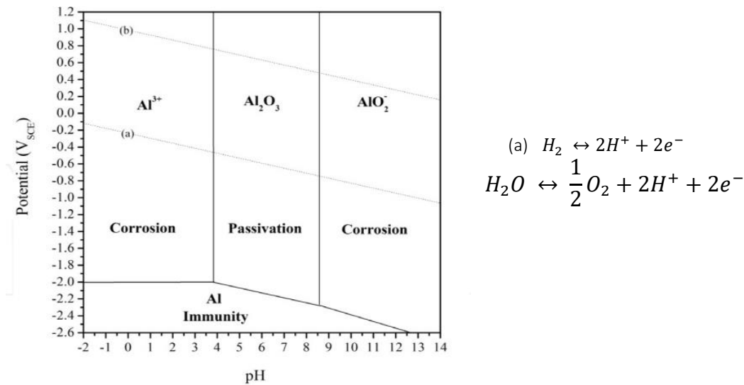
Figure 5 : E-pH diagram for pure Al at 25 °C in aqueous solution (adapted from Pourbaix 1974). The lines (a) and (b) correspond to water stability and its decomposed product. (from [27])
