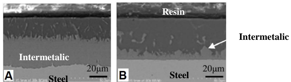
Figure 3 : Cross-sectional SEM views of aluminized steel sheets which were hot dipped in pure Al (A) and AlSi9 (B) at 800 °C. Intermetallic phase between coating and steel. (from [6])
