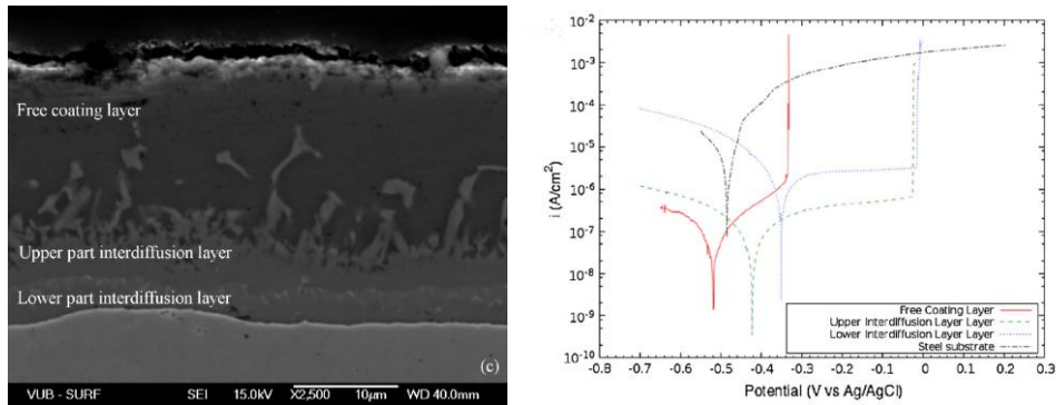
Figure 12 : SEM observation and potentiodynamic polarization curves in 0.1 M NaCl solution of Aluminum-Silicon coating different layers obtained by the electrochemical micro-cell positioned in the GDOES sputter craters (from [51]).
