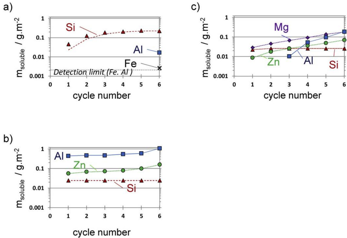
Figure 6 : Evolution of the quantity of soluble Al, Si, Zn and Mg in the solution collected with cycling in accelerated corrosion test VDA 233-102 for (a) AlSi, (b) AlSiZn and (c) AlSiZnMg coatings. For each chemical element the total dissolved mass is normalized by the sample surface area, msol / g.m^{-2} .
