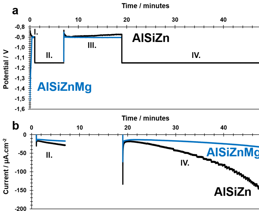
Figure 4 : (a) Potential and (b) current evolution at OCP and under cathodic polarization in 1 wt. % NaCl aqueous solution at initial pH7.
