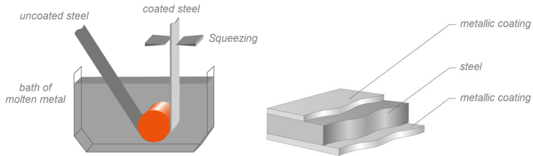
Figure 2 : Hot dip process and coating system drawing (from [3]).
