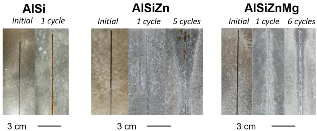
Figure 5 : Typical surface appearance of AlSi, AlSiZn and AlSiZnMg coated steels before (initial) and after several cycles of accelerated corrosion test VDA 233-102 (as indicated).
