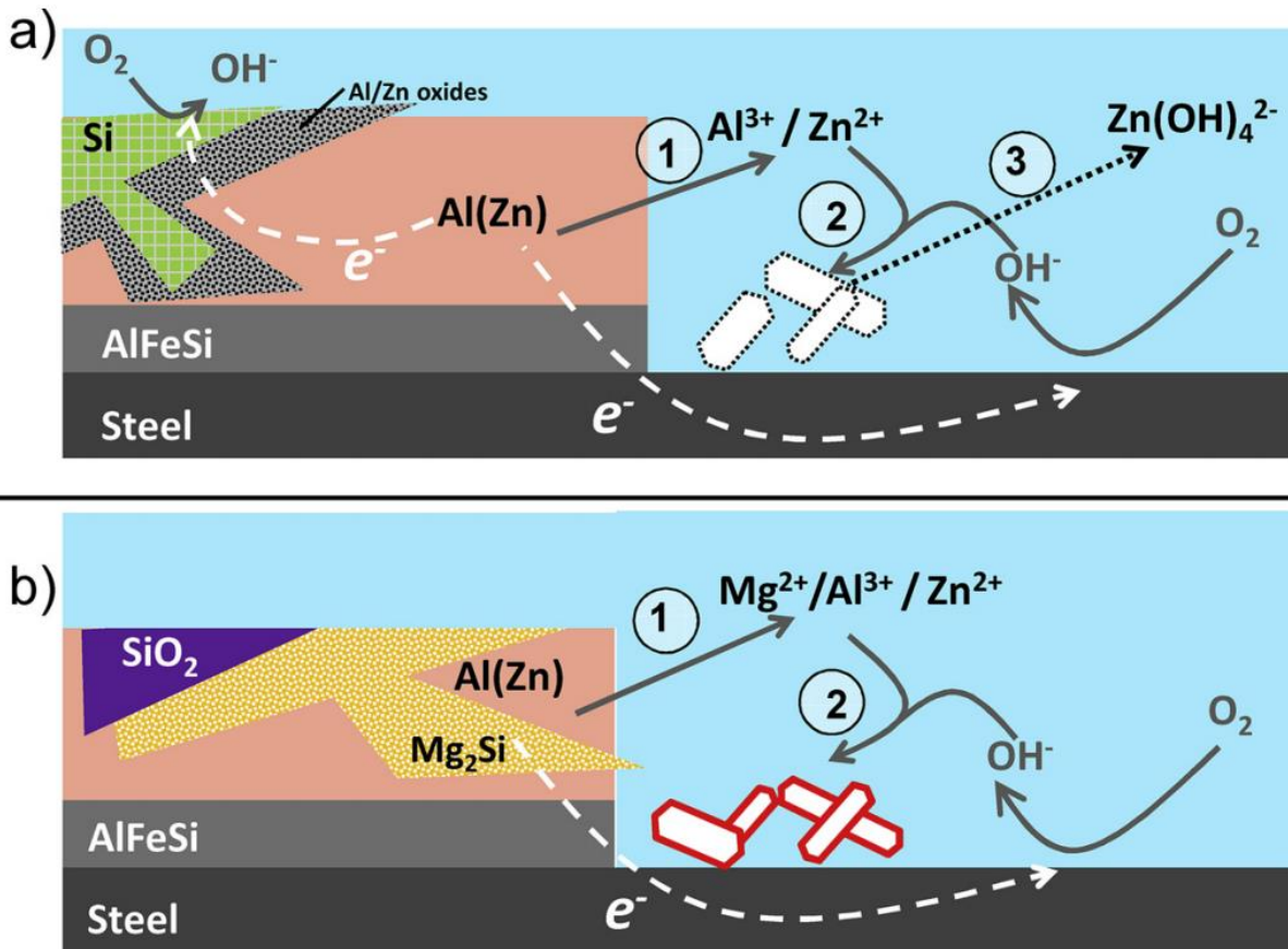
Figure 10 : Schematic representation of proposed corrosion and protection mechanisms in (a) AlSiZn and (b) AlSiZnMg coated steel in the presence of the defect going up to the steel. Step 1. Coating dissolution and sacrificial effect. For AlSiZn two types of microgalvanic coupling are proposed - "sacrificial" coupling protecting steel and "lost" current used in micro galvanic coupling with Si because Si potential (60.5 V vs. SCE) is close to potential of steel and cathodic versus AlZn. Step 2. Precipitation (and partial modification) of corrosion products due to pH increase and drying. Step 3. Dissolution of Zn and Al containing corrosion products from AlSiZn at advanced stages of corrosion because of continuous pH increase. This step is absent when corrosion products contain Mg^{2+} because of their high pH stability (for instance Mg(OH)_2 formation in place of dissolution of LDH resulting in a skin effect). As a result, Mg is expected to extend both, the coating life (and hence a sacrificial protection) and the barrier effect of corrosion products in the scratch.
