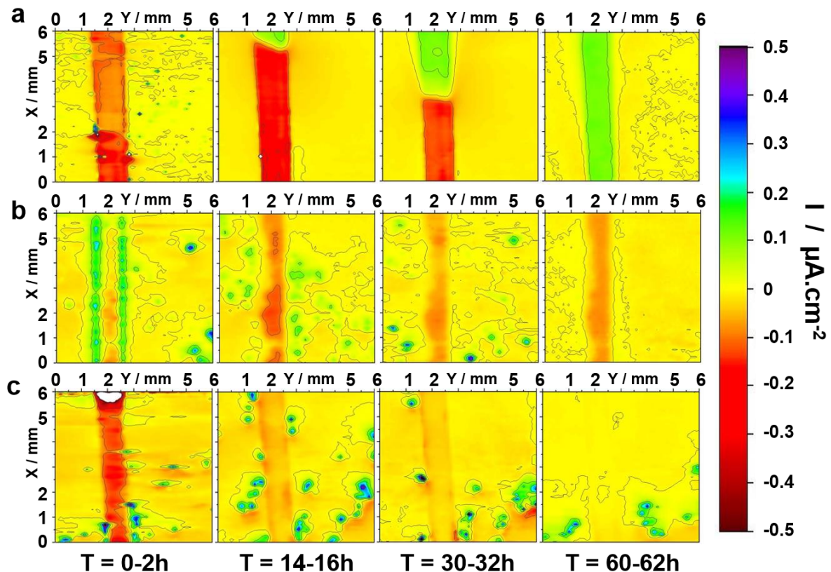
Figure 4 : SVET cartography of (a) AlSi, (b) AlSiZn and (c) AlSiZnMg scratched coating at different times of immersion in 100 \text{ mg.L}^{-1} \text{ NaCl} solution.
