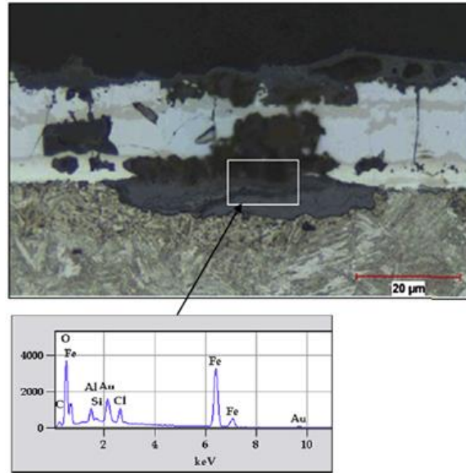
Figure 13 : SEM image and EDS spectra in the corroded zone at the interface between the coating and the substrate (the area of analysis is indicated). The sample was corroded in accelerated tests. Gold (Au) a 20 nm gold layer was sputtered on the surface before SEM observation in order to avoid the charging of the non-conductive corrosion product surface (from [12]).
