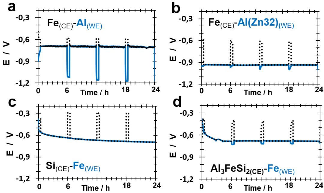
Figure 3 : Evolution of the potentials measured in coupling experiments between the substrate steel and the phases relevant for the AlSi(Zn,Mg) coating. Coupled phases: (a) Fe-Al, (b) Fe-Al(Zn32), (c) Si-Fe and (d) \text{Al}_3\text{FeSi}_2 -Fe in 0.172 M NaCl aqueous solution. Coupling tests consisted of 6 h cycles, each cycle consisted of 30 minutes of the OCP measurement on two uncoupled phases followed by 5 hours and 30 minutes of galvanic coupling).
