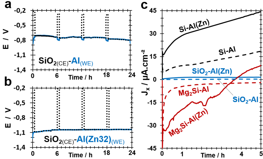
Figure 6 : Evolution of potential measured on 2 phases during coupling tests for (a) SiO 2 -Al and (b) SiO 2 -Al(Zn32) in NaCl 0.172 M aqueous solution. (c) Galvanic current of Si containing phases and Al or Al(Zn32) in NaCl 0.172 M aqueous solution.
