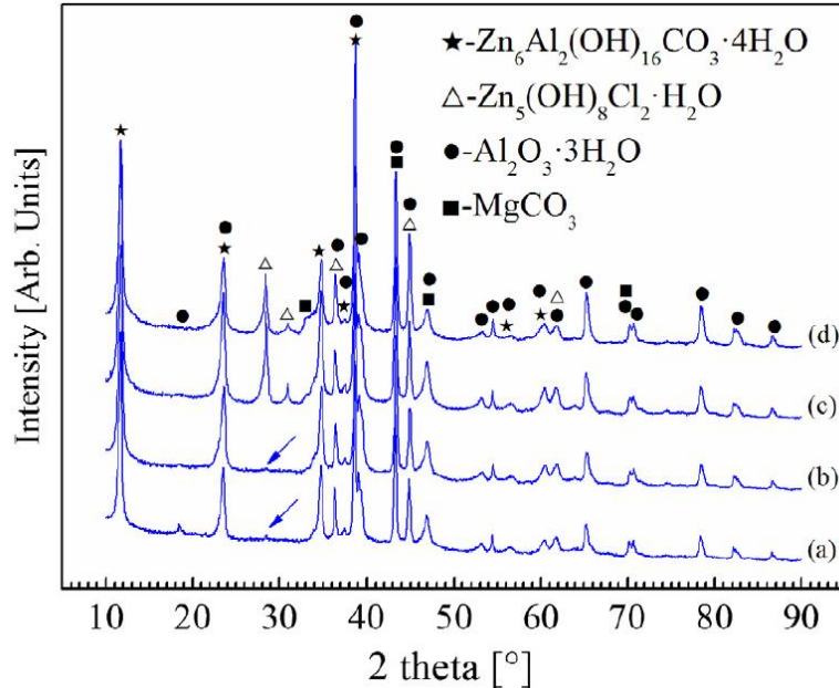
Figure 14 : XRD spectra of different corrosion products collected from the surface of the corroded coatings after 168 h exposure to NSS test according to EN ISO 9227: (a) Galvalume® coating, (b) G–0.5Mg coating, (c) G–1.5Mg coating, (d) G–2.5Mg coating (from [19]).
