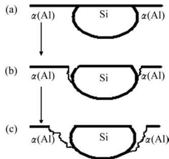
Figure 10 : Schematic mechanism of local corrosion around a Si particle (from [46]).
