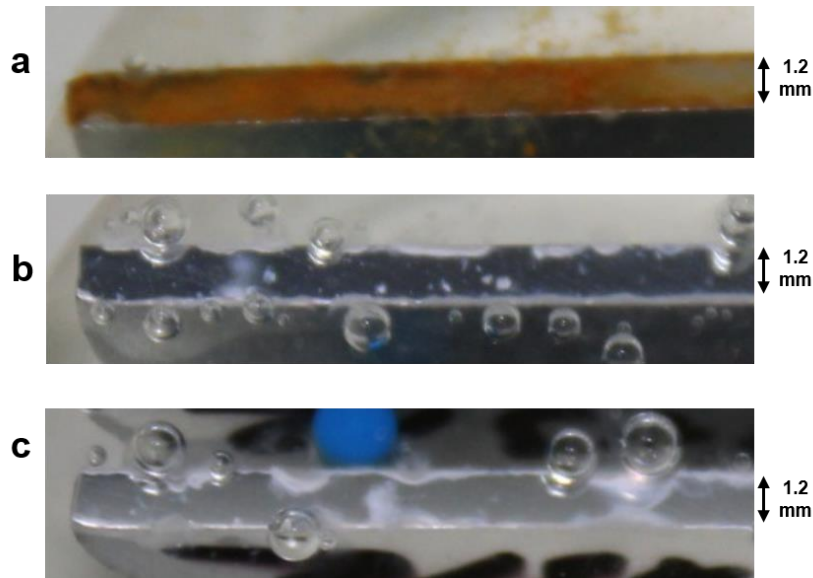
Figure 1 : Typical example of in-situ optical images of immersed cut edges of (a) AlSi, (b) AlSiZn, (c) AlSiZnMg after 48h immersion in 1 wt. % NaCl aqueous solution at initial pH 7.
