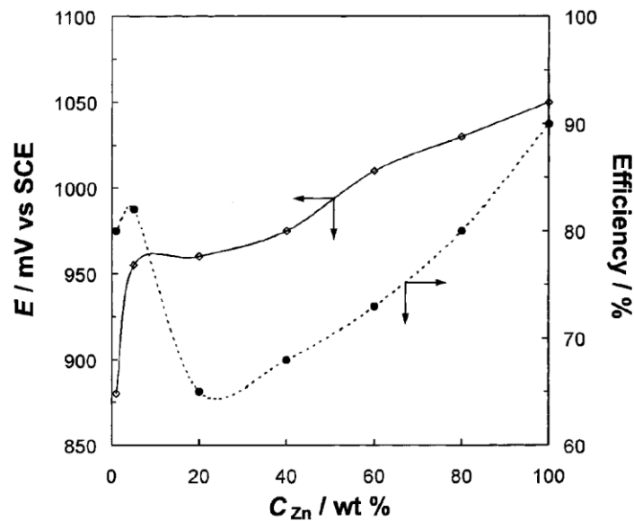
Figure 8 : Anode efficiency and operating potentials of the Al-Zn alloys with different Zn content. (from [16])
