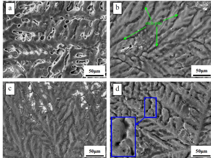
Figure 15 : Morphologies of different corroded coating surfaces after dissolving corrosion products with 10wt. % ammonium persulphate solution: (a) Galvalume coating, (b) G– 0.5Mg coating, (c) G–1.5Mg coating and (d) G–2.5Mg coating (from [19]). etc.
