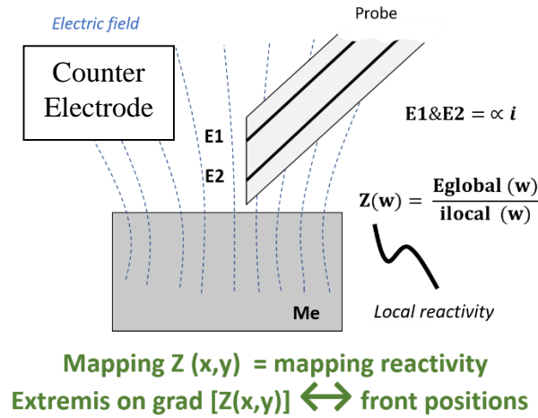
Figure 2 : Local Electrochemical Impedance Spectroscopy (LEIS) explanatory diagram.
