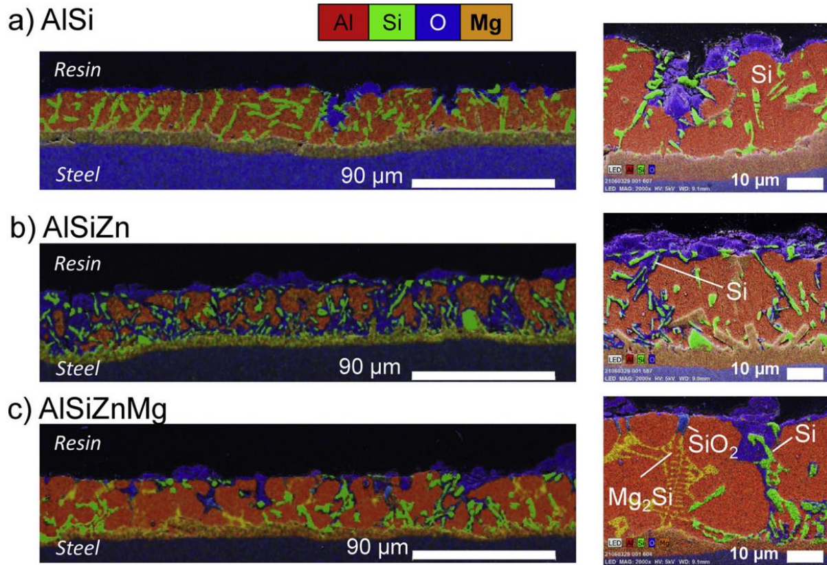
Figure 8 : EDS maps showing corrosion products distribution after 12 cycles of the VDA 233-102 test in the cross sections of unscratched (a) AlSi, (b) AlSiZn and (c) AlSiZnMg coated steels with high Si content. O distribution permits to distinguish corrosion products from non-corroded areas while Al, Si and Mg distributions help to identify the phases. General view and more resolved images are shown.
