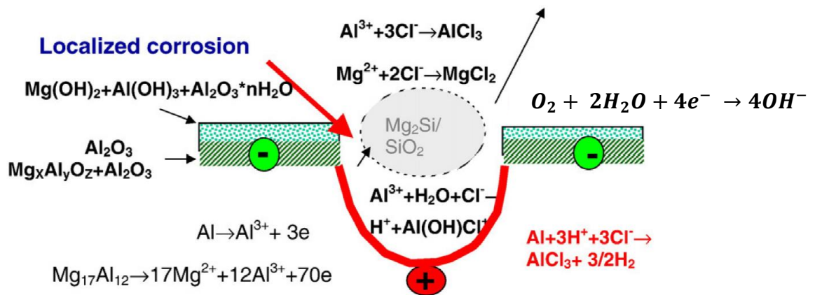
Figure 11 : Localized corrosion mechanisms of Mg 2 Si in Al and AlMg matrix (from [50]).
