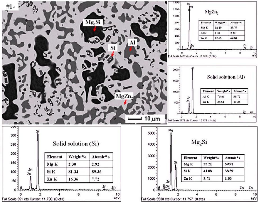
Figure 4 : SEM images and EDS analysis of present phase for an Al 15 Zn 62 Mg 17 Si 6 alloy. (from [21])
