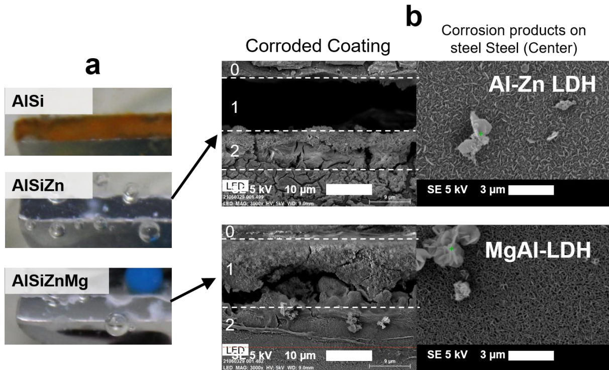
Figure 11 : (a) Typical cut edges appearance of AlSi, AlSiZn, AlSiZnMg coatings after 48h immersion in 1 wt. % NaCl aqueous solution at initial pH7. (b) Secondary Electron Images of AlSiZn and AlSiZnMg coatings cut edges after 48h immersion in 1 wt. % NaCl aqueous solution at initial pH7. 0: Resin; 1: Coating; 2: Intermetallic.
