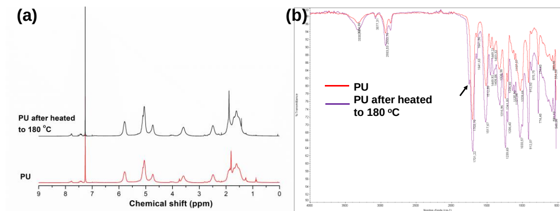
Figure 2.25. ^1\text{H} NMR (a) and ATR-IR (b) spectra of PU polymer ( M_n = 4000\text{ Da} ) and PU after heated to 180 °C and cooled to r.t. slowly under argon.
