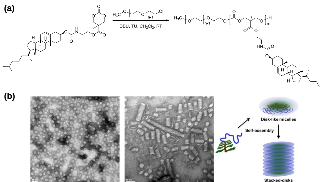
Figure 3.5. (a) Synthesis of cholesterol-functionalized amphiphilic polycarbonate diblock copolymer m\text{PEG}_{113}\text{-}b\text{-P(MTC-Chol)}_n via organocatalytic ROP. (b) TEM images and schematic illustration of disk-like micelles and stacked-disk-like aggregates formed by the self-assembly of m\text{PEG}_{113}\text{-}b\text{-P(MTC-Chol)}_n copolymers. 21
