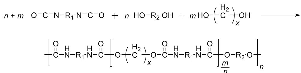
Figure 1.2. General structure of linear, single-phase ( m=0 ) and phase-separated ( m=1, 2 ) PUs on the micrometer scale. Rigid segments (urethane linkages) and flexible segments (polyols) are distributed statistically. 4
