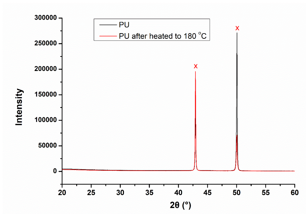
Figure 2.26. XRD spectra of PU polymer ( M_n = 4000\text{ Da} ) and PU after heated to 180 °C and cooled to r.t. slowly under argon. The two diffraction peaks (x) are from the sample support made of copper.
