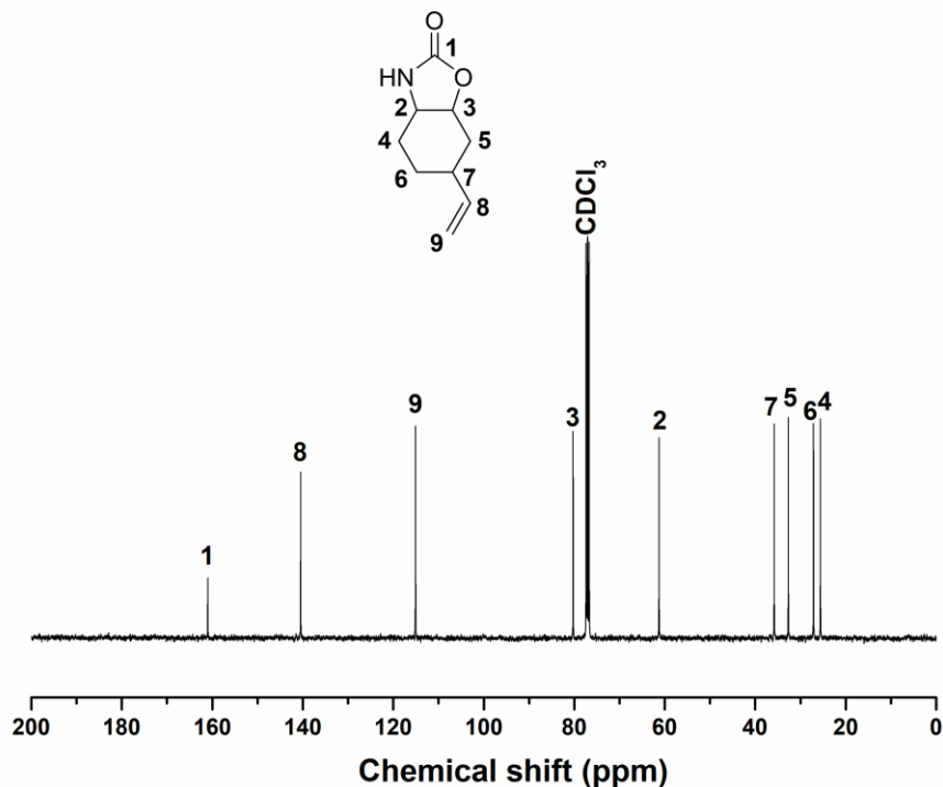
Figure 2.7. ^1\text{H} NMR (a) and ^{13}\text{C} NMR (b) spectra of CHU monomer. \text{CDCl}_3 , 300 MHz, 297 K.
