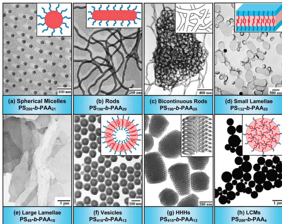
Figure 1.25. Transmission electron microscopy (TEM) photographs and corresponding schematic diagrams of various morphologies formed from amphiphilic \text{PS}_m\text{-}b\text{-PAA}_n copolymers. Note: m and n are the degrees of polymerization of PS and PAA, respectively. In the schematic diagrams, the red represents hydrophobic PS parts, while the blue denotes hydrophilic PAA segments. HHHs: hexagonally packed hollow hoops; LCMs: large compound micelles, in which inverse micelles are composed by a PAA core surrounded by PS coronal chains. Generally, the hydrophilic segments of the “crew-cut” aggregates cannot be seen in TEM images if they are not stained. 72
