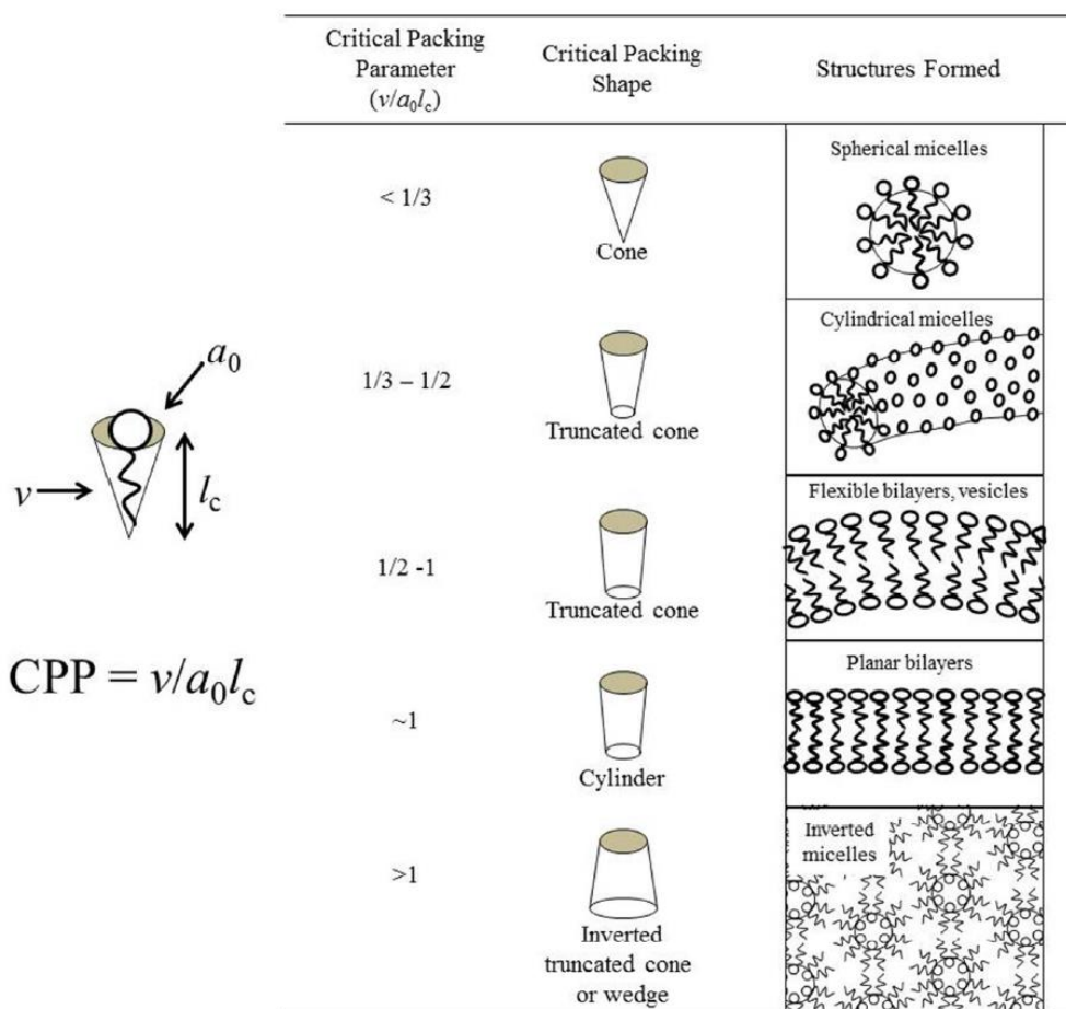
Figure 1.21. Critical packing parameter (CPP, also called packing parameter, p ) of molecules for self-assembly and the morphologies of the formed assemblies. 59
