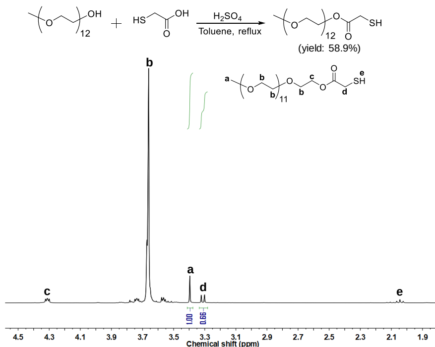
Figure 4.8. Synthetic scheme and 1 H NMR spectrum of mPEG 12 -SH.
