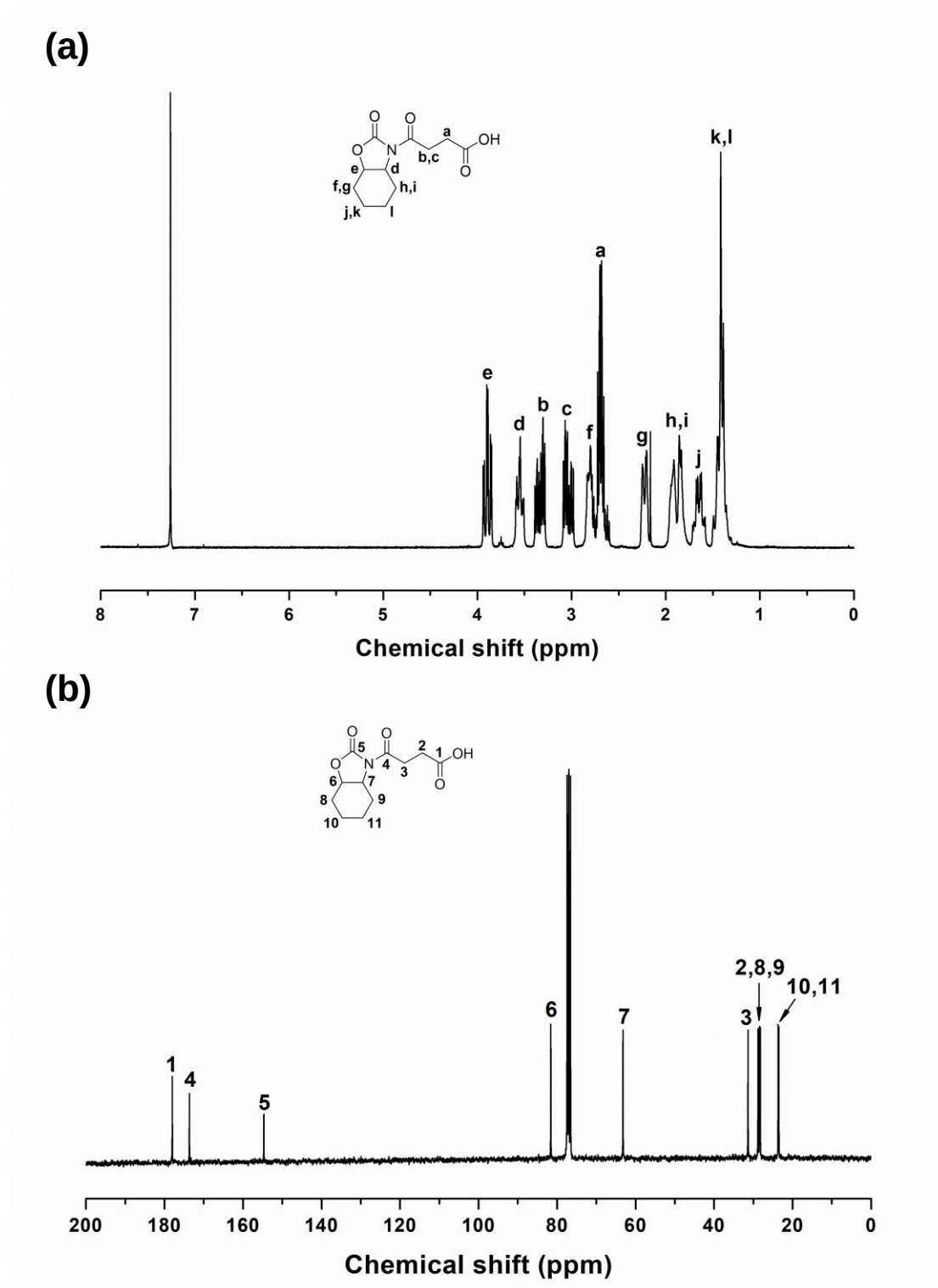
Figure 3.11. ^1\text{H} NMR (a) and ^{13}\text{C} NMR (b) spectra of CHU-COOH. \text{CDCl}_3 , 400 MHz, 297 K.
