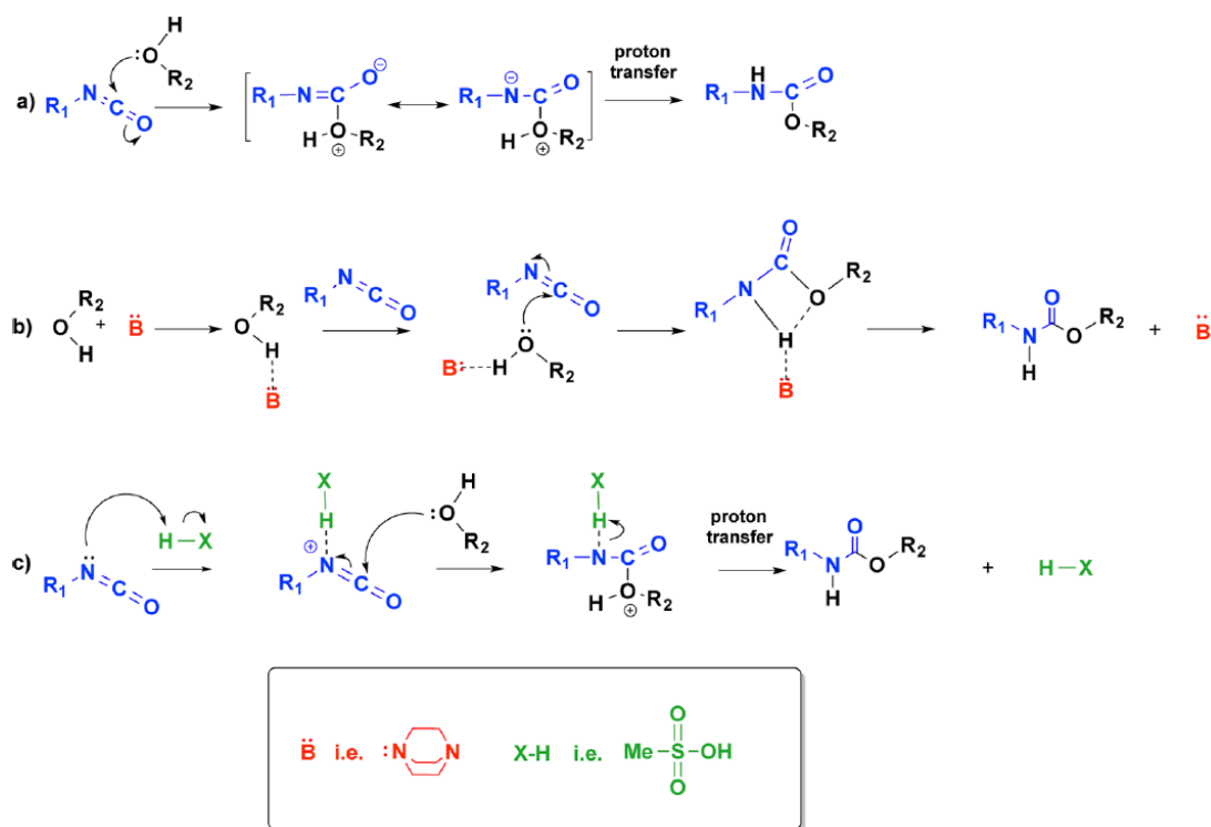
Figure 1.7. General mechanism of isocyanate/alcohol reaction (a) in the absence of catalyst, (b) in the presence of a base or nucleophilic activator, and (c) in the presence of an acid or electrophilic activator. 9
