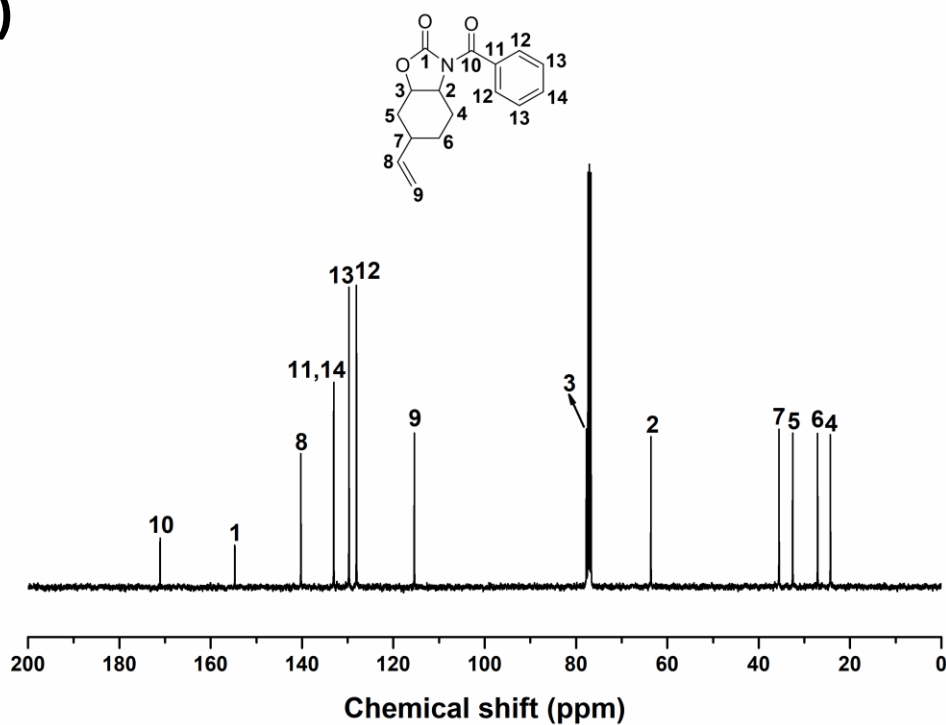
Figure 5.9. 1 H NMR (a) and 13 C NMR (b) spectra of CHU-derived imide II . CDCl 3 , 400 MHz, 297 K.
