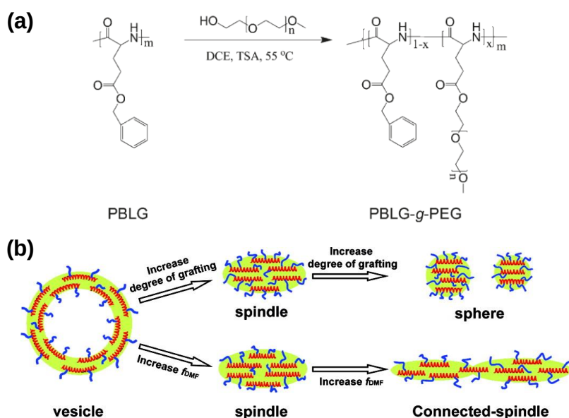
Figure 4.5. (a) Synthesis of PBLG-g-PEG graft copolymer by ester exchange reaction. DCE: 1,2-dichloroethane; TSA: p -toluenesulfuric acid. (b) Schematic representation of the morphology transition from vesicles to spindles, and then to spheres. 21
