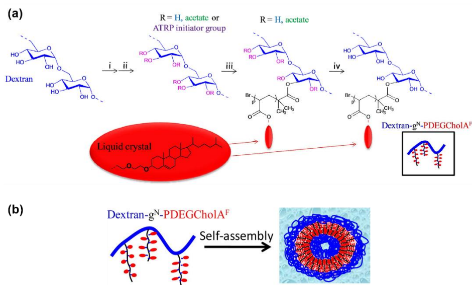
Figure 4.6. (a) Synthesis of amphiphilic Dex-g N -PDEGCholA F graft glycopolymers using a “grafting from” strategy. (b) Schematic illustration of the self-assembly of graft glycopolymers into polymersomes. 22
