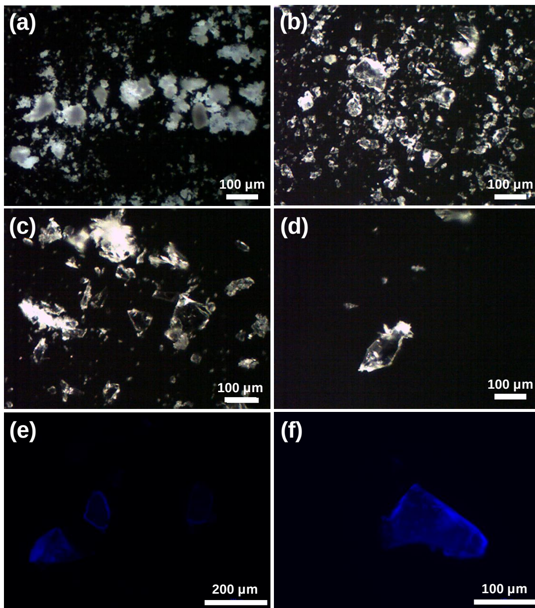
Figure 2.24. Photographs captured by POM (a-d) and Fluorescence microscopy (e,f). (a) original PU samples ( M_n = 4000 Da) without being heated; (b-f) PU samples after heated to 180 °C and cooled to r.t. slowly under argon.
