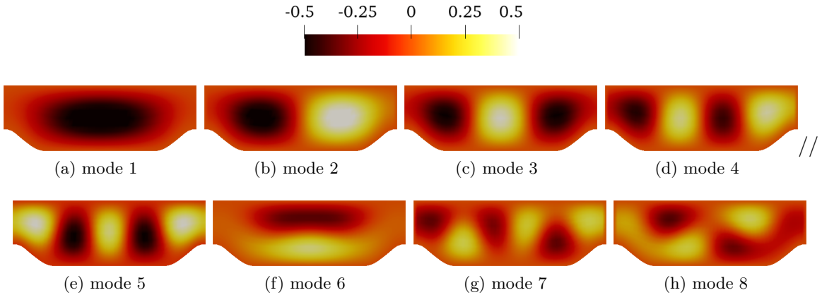
Figure 4.9: Contour plots of first 8 modes from KL decomposition for the periodic hills case. The modes are scaled by their corresponding eigenvalues.
