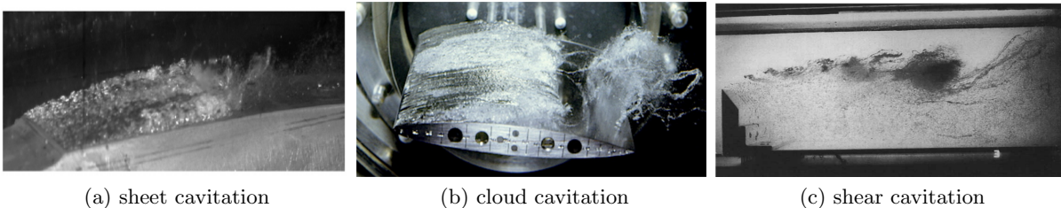
Figure 1.2: The different cavitation patterns. Adopted from [6, 17, 110]
