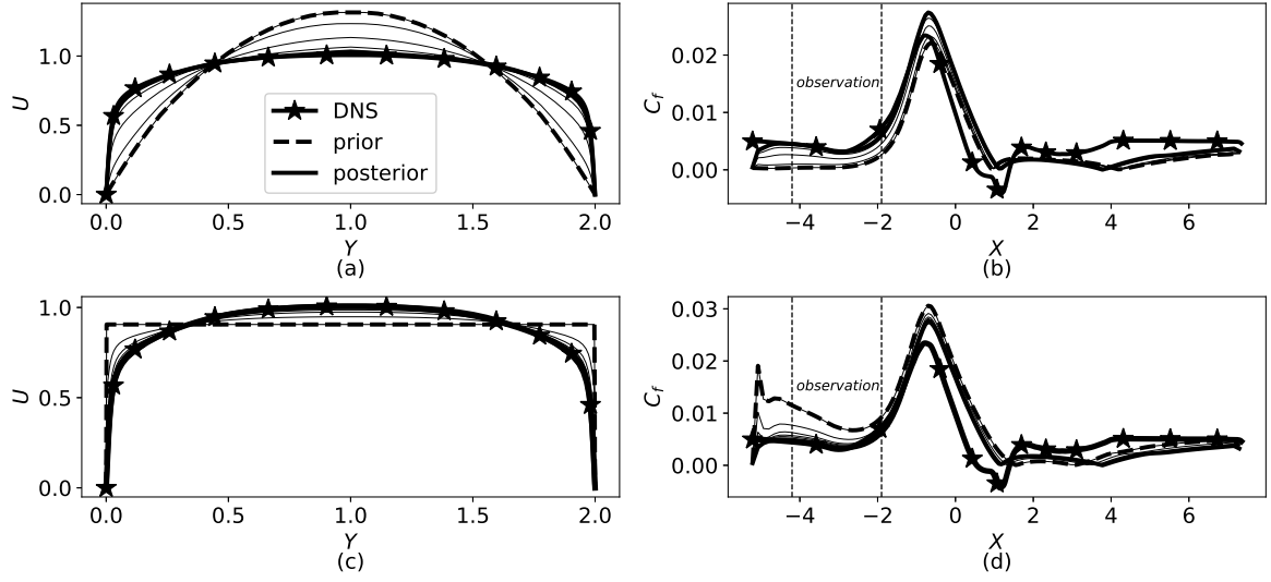
Figure 3.3: Data assimilation results about the inferred inlet velocity and the prediction in C_f : (a) (b) for the prior of parabolic velocity; (c) (d) for the prior of flat velocity
