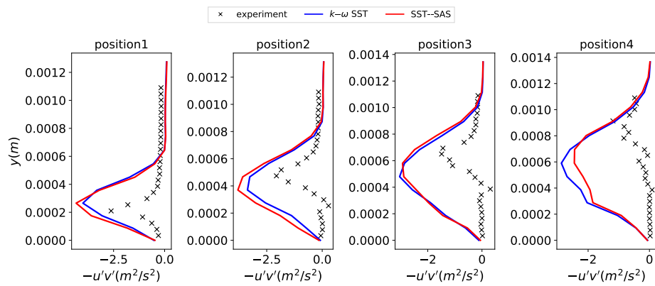
Figure 6.12: Comparison in Reynolds shear stress between the different turbulence models and experiments without Rebound correction.
