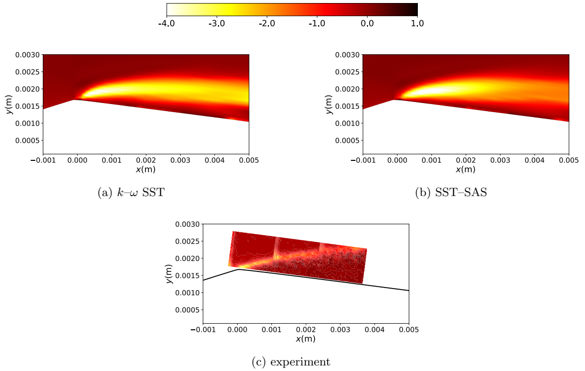
Figure 6.11: time-averaged Reynolds shear stress without Rebound correction.
