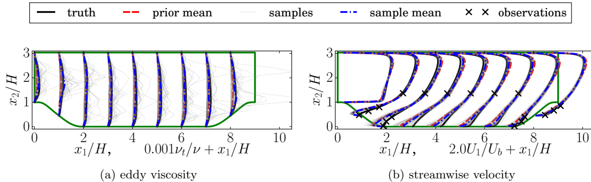
Figure 4.10: Prior realizations of eddy viscosity \nu_t and propagated streamwise velocity U_1 for the periodic hills case. The locations of the observations are indicated by crosses ( \times ).
