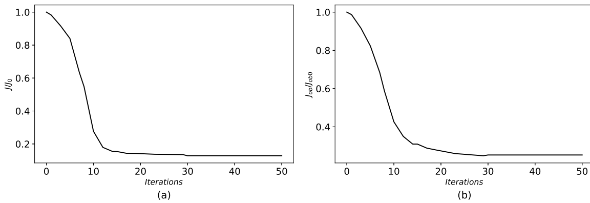
Figure 3.15: data assimilation results in cost function J (a) and J_{ob} (b)
