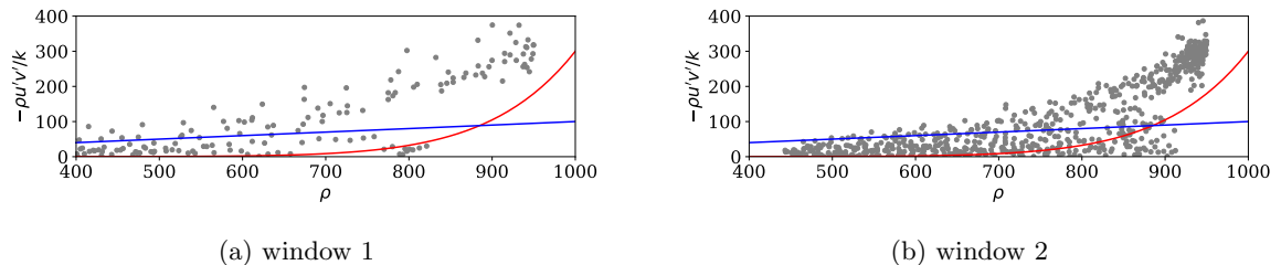
Figure 6.14: The comparison of the Reboud correction with n = 10 (red line), the Bradshaw assumption with c = 0.1 (blue line) and experimental data (grey dots)
