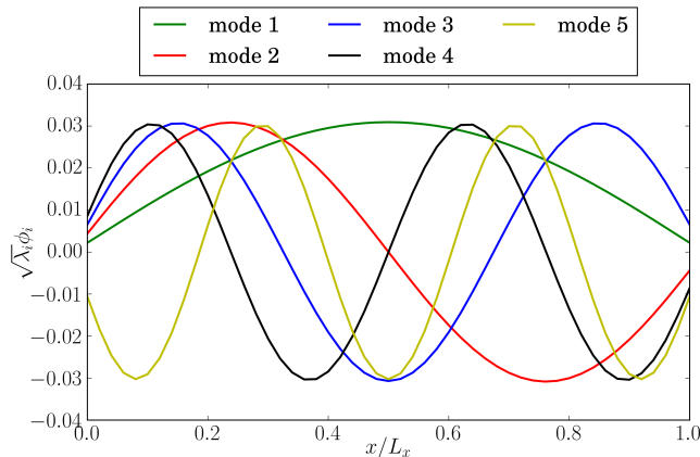
Figure 4.4: First 5 KL modes in the diffusion case scaled by their corresponding eigenvalues.
