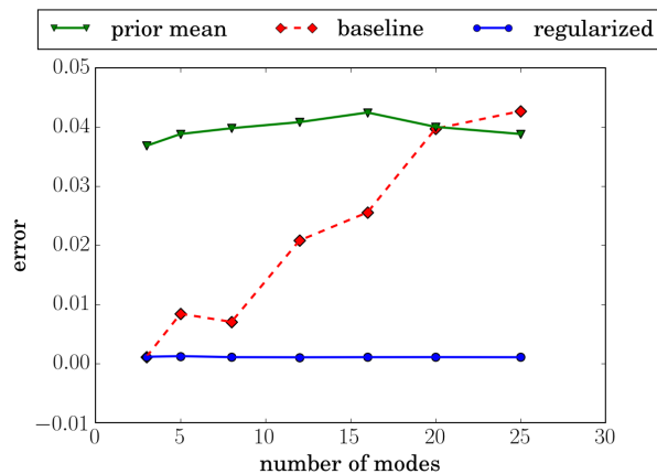
Figure 4.8: Errors in the inferred diffusivity in the diffusion case for the baseline method and the regularized methods as a function of number of modes used in the field representation.
