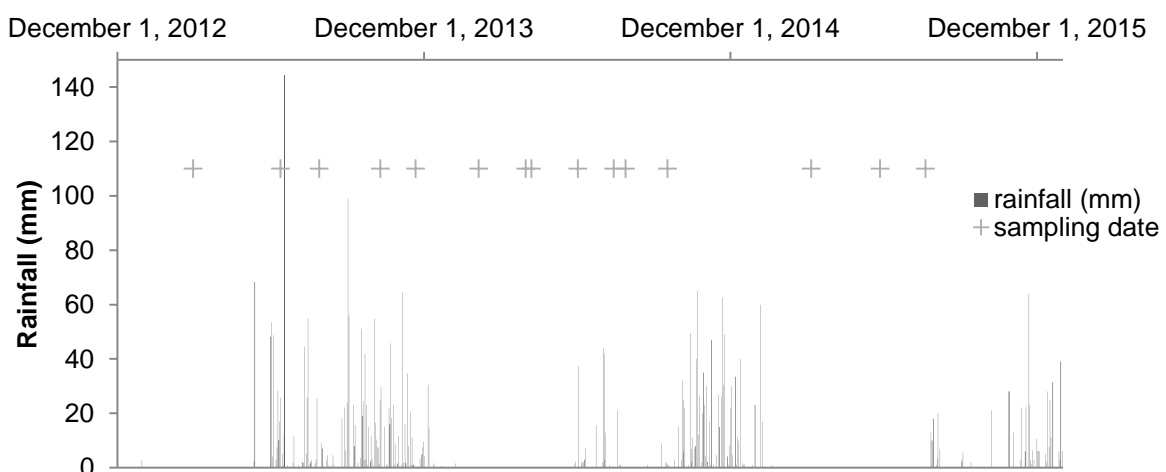
86 Fig. 1 Water sampling dates and daily rainfall from December 1 st , 2012 to December 31 st , 2016 (NOAA National 87 Data Centers 2015) 88
