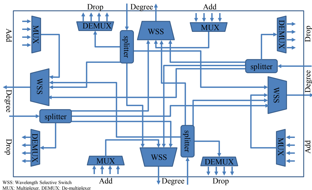
Figure 3.3: Example of colored, directed four-degree ROADMs, based on Wavelength Selective Switches and splitters. The structure uses a broadcast and select architecture. WDM mux and demux are used for Add and Drop ports.
