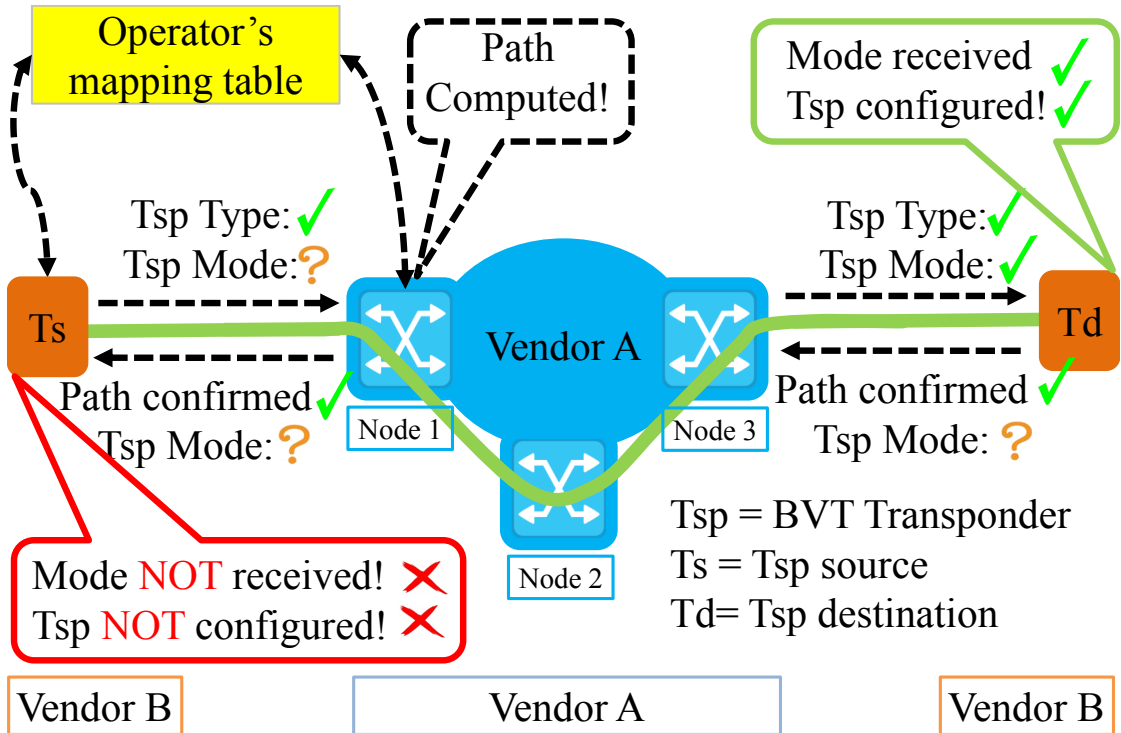
Figure 4.4: Alien wavelength lightpath setup using the RSVP-TE-based approach with BVTs; The transponder's mode is not sent upstream to Ts and the lightpath setup fails
