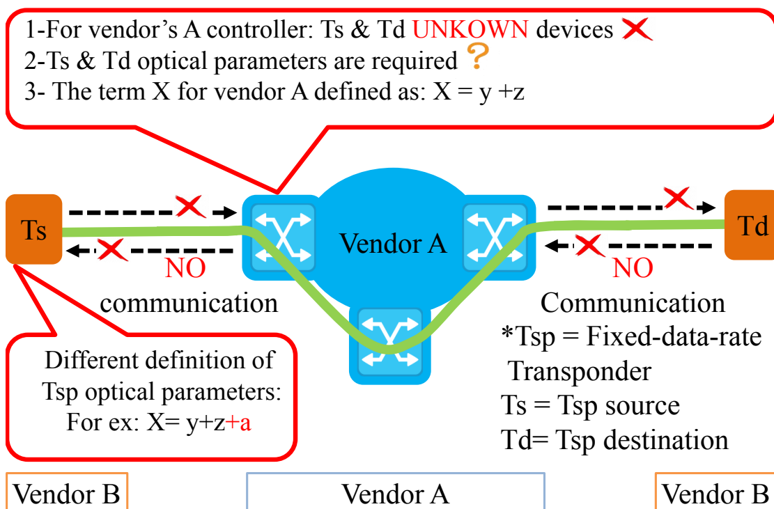
Figure 4.1: Challenges faced by automating the alien lightpath setup process from the control and management point of view
