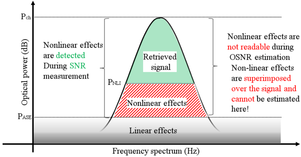
Figure 3.5: Spectrum analysis of an optical signal at the receiver side with nonlinear noise spectrally superimposed over the signal, this figure is an exploratory one since, the nonlinear effects might superimposed in a different shape over the signal and not exactly as shown here.
