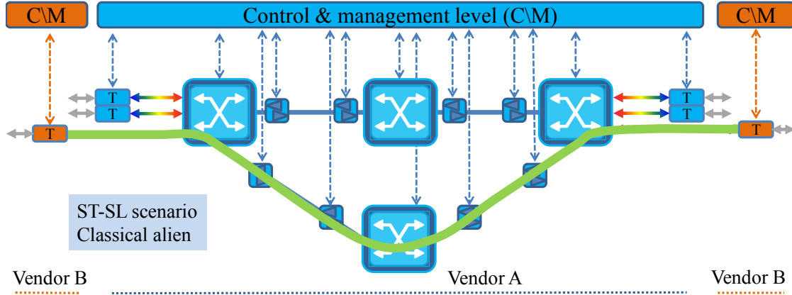
Figure 3.7: Single-vendor Transponder - Single-vendor Line (ST-SL) scenario, i.e. classical alien scenario. The color code is used to differentiate between vendors' equipment.
