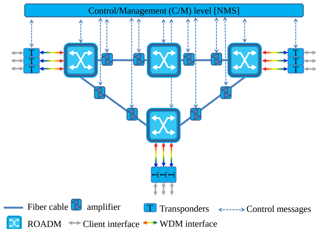
Figure 3.1: Structure of a WDM transport system, when purchased from a single vendor
