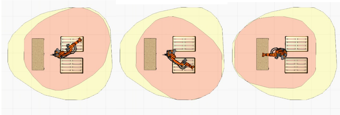
Figure 26: Screenshots from simulation of robot in application. The yellow polygon represents the minimum required separation distance over the entire programmed path. The red polygon represents the instantaneous required separation distance based on the robot's current speed at that moment along the programmed path.
