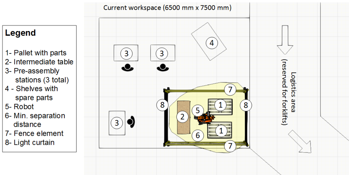
Figure 29: Final selected configuration with a KR22 robot, 2 light curtains, and 2 fences to limit access to the pallets and the table.
