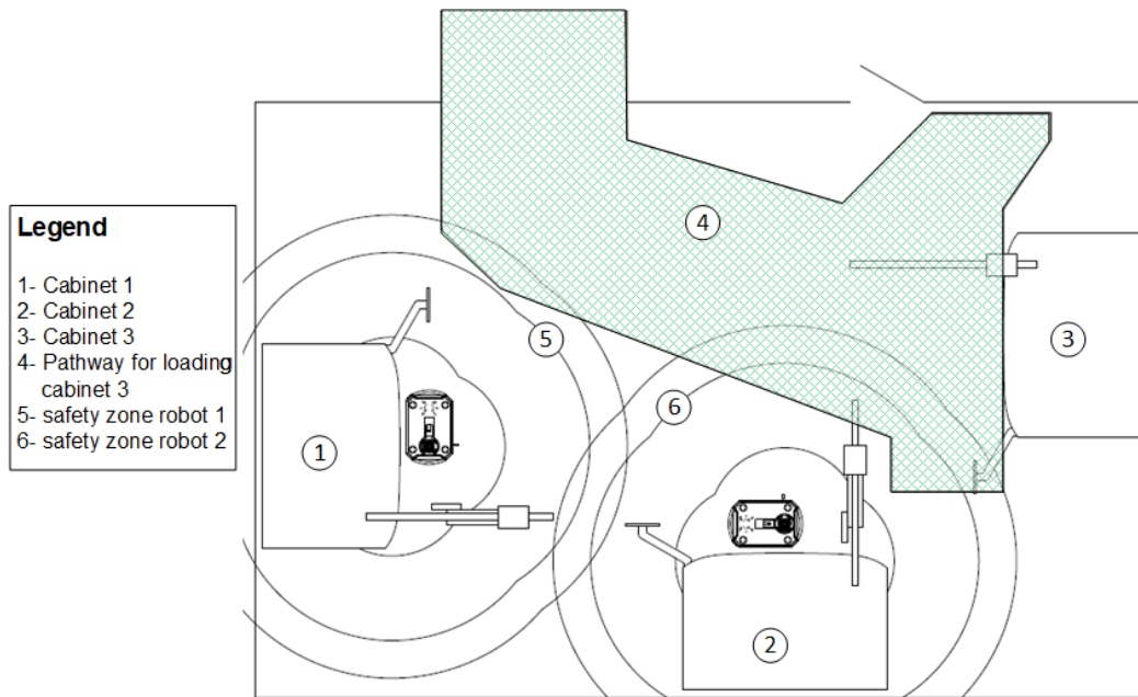
Figure 25: The calculated safety zones for robots working in cabinets 1 and 2 and the floor space needed to load / unload cabinet 3.
