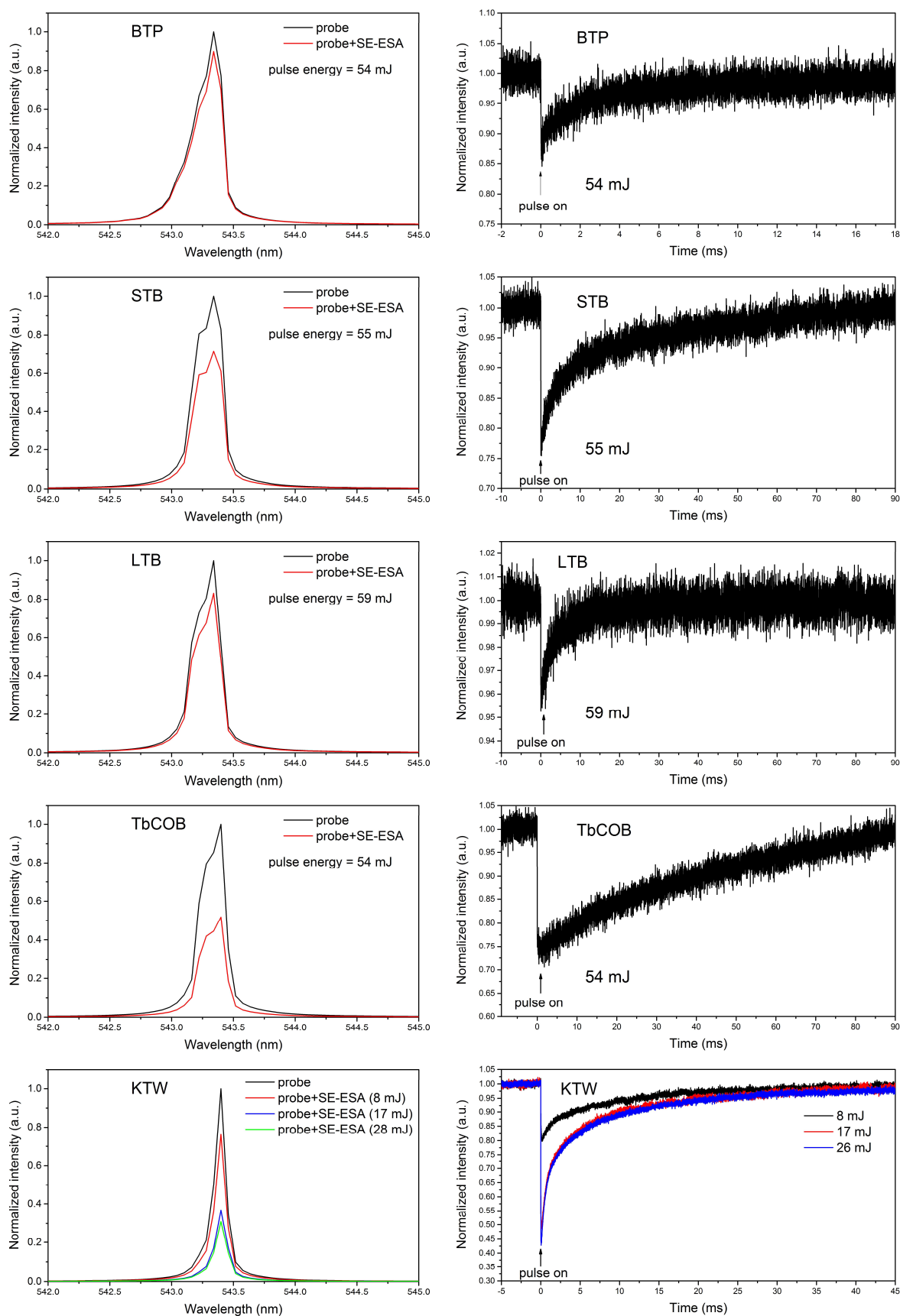
Figure 3.28 Left: emission spectra without (marked as “probe”) and with the pump (marked as “probe+SE-ESA”); Right: time-evolution curves of the photon intensity monitored at 543.4 nm.
