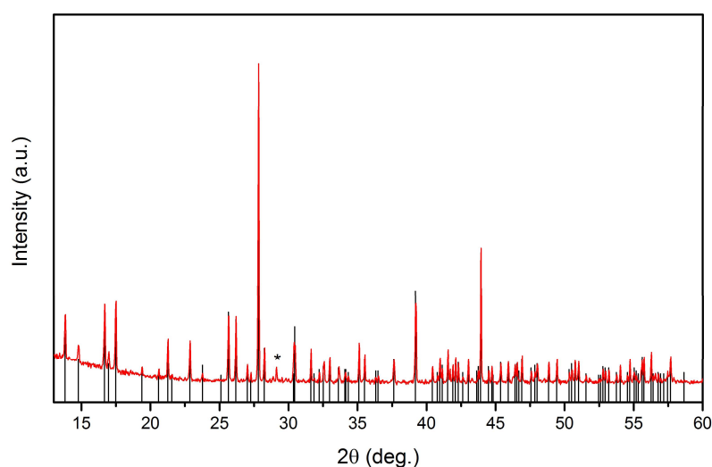
Figure 2.13 Powder X-ray diffraction pattern of the white LTB polycrystals (reference ICDD code: 00-061-0412).
