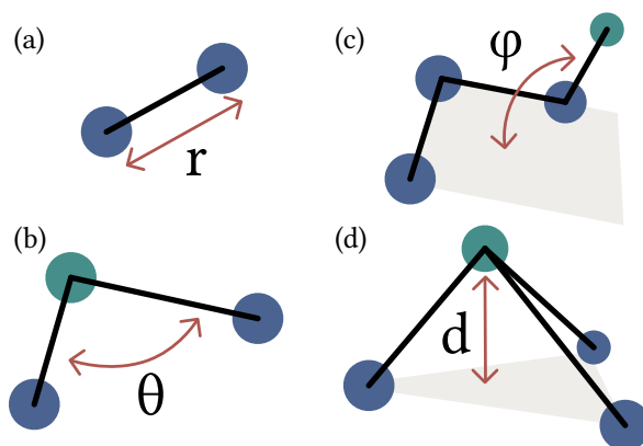
Figure 3.1 – Definition of the parameters used to compute the energy of a molecular system with classical force field. (a) bonds; (b) angles; (c) dihedral angles; (d) improper dihedrals/out of plane distance.
