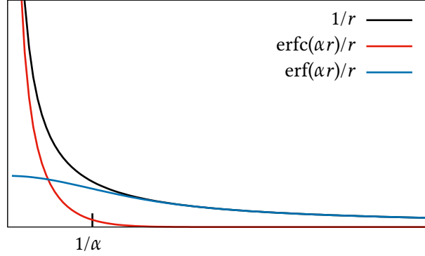
Figure 6.5 – Shape of the functions involved in Ewald summation: 1/r , \text{erfc}(\alpha r)/r , and \text{erf}(\alpha r)/r .
