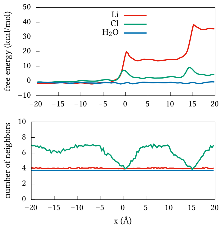
Figure 5.11 – Free energy profile (top) of a single molecule entering ZIF-8 and corresponding number of neighbors (bottom) in the first solvation shell as function of the position of the molecule along the (111) crystallographic axis. The first ZIF-8 window is at x = 0 ; the x < 0 area corresponds to bulk water, and the x > 0 area to water-filled ZIF-8. We evaluated the uncertainty on the free energy profile using Monte Carlo bootstrapping [183] , and found it to be at most 0.08 kcal/mol for H 2 O, and 0.3 kcal/mol for Cl − and Li + .
