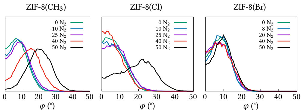
Figure 4.4 – Distribution of linker swing angle (Zn – Zn – Zn – X dihedral angle, where X stands for CH 3 , Cl or Br for ZIF-8(CH 3 ), ZIF-8(Cl) or ZIF-8(Br), respectively) at various values of nitrogen loading.
