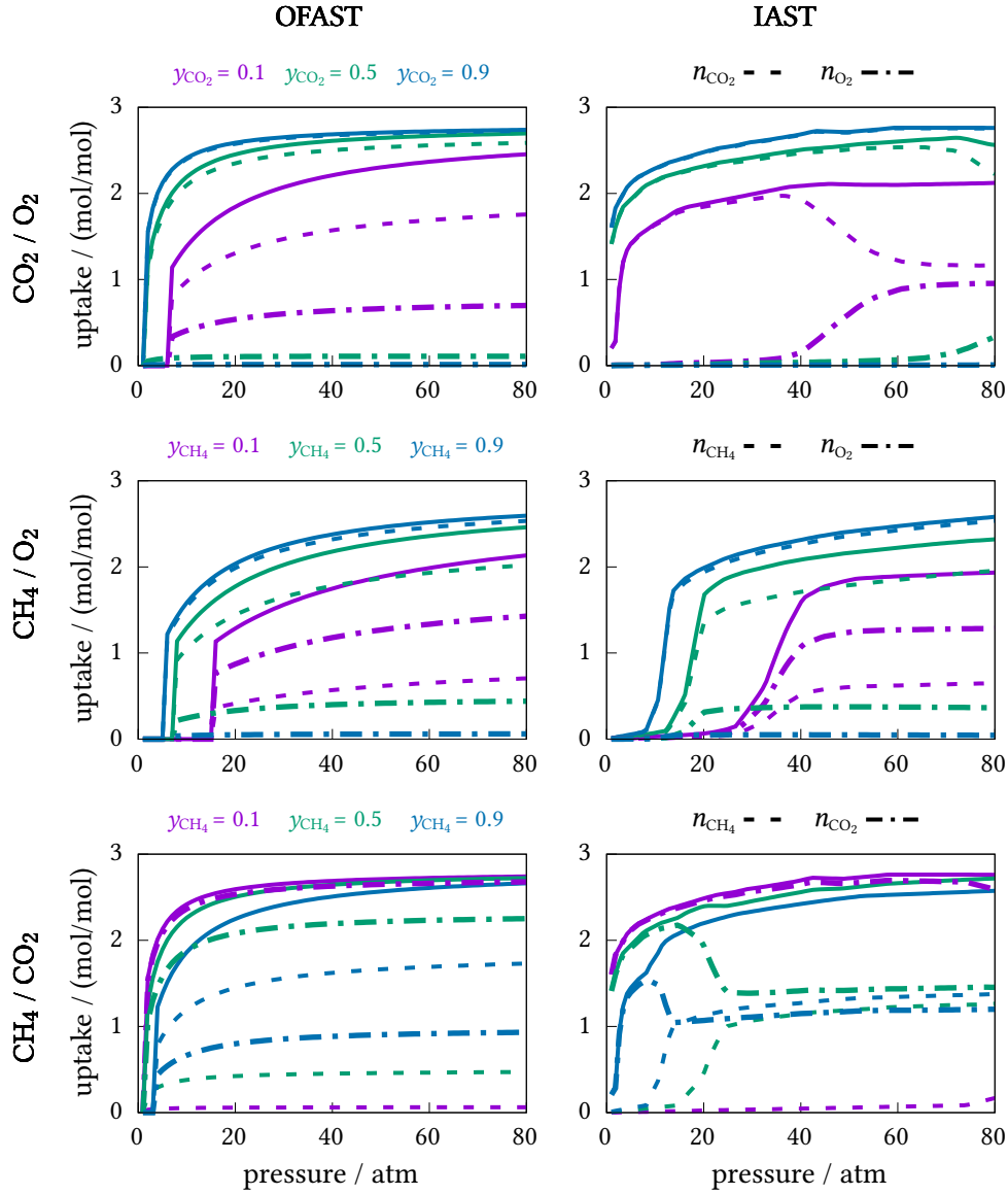
Figure 2.6 – Total (full lines) and partial (dashed lines) loading as function of pressure in \text{Cu(dhbc)}_2(4,4'\text{-bpy}) for all the gas pairs: from top to bottom \text{CO}_2 / \text{O}_2 ; \text{CH}_4 / \text{O}_2 ; and \text{CH}_4 / \text{CO}_2 . OFAST results are presented on the left, and IAST results on the right.
