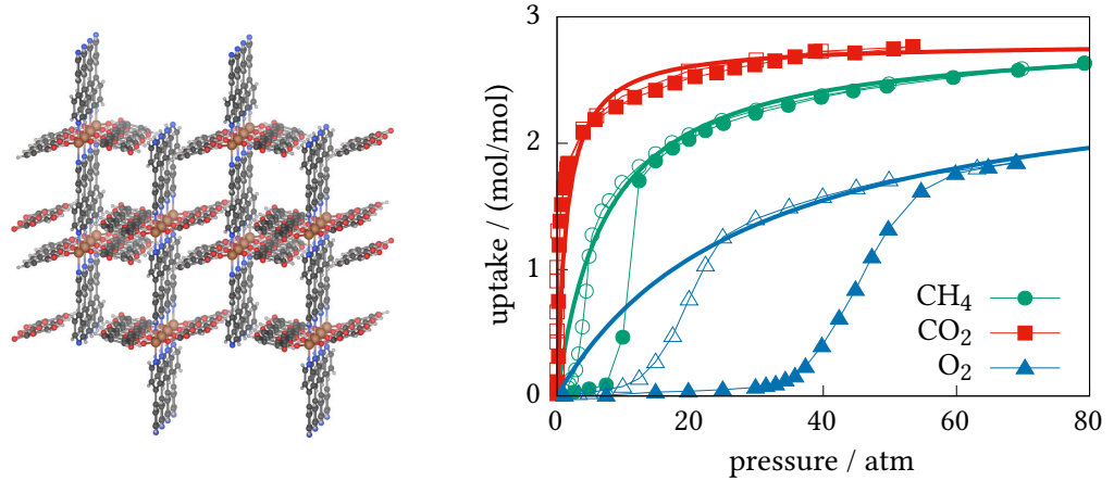
Figure 2.4 – (left) Cu(dhbc) 2 (4,4'-bpy) structure (from reference. [66]). (right) Sorption isotherms and model isotherms fit at 298 K in Cu(dhbc) 2 (4,4'-bpy) for various gas compounds. Adsorption data are presented using filled symbols, and desorption data using empty symbols. Thick lines are Langmuir isotherms fitted at high loading. Experimental data published by Kitaura et al.[66]
