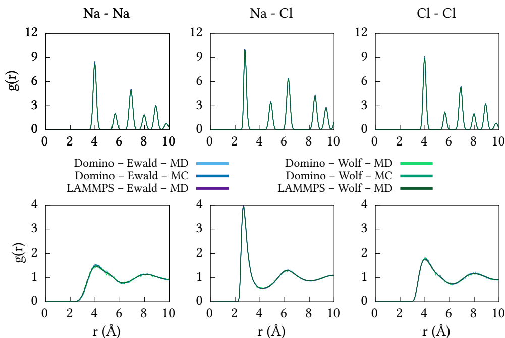
Figure 6.6 – Radial distribution function for three pairs (from left to right Na–Na, Na–Cl, and Cl–Cl) on two system: a solid NaCl crystal at 300 K on top, and melted NaCl at 2000 K on bottom.
