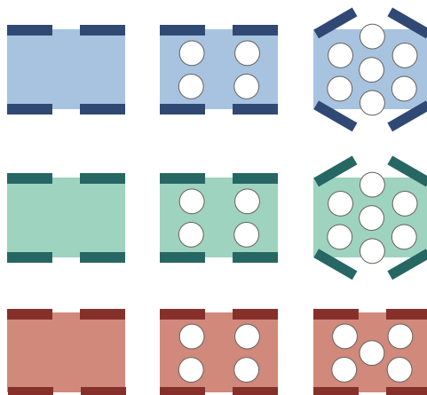
Figure 4.9 – Schematic overview of the adsorption process in the three ZIF-8 frameworks. Blue is ZIF-8(CH 3 ), green is ZIF-8(Cl) and red is ZIF-8(Br); loading increases from left to right.
