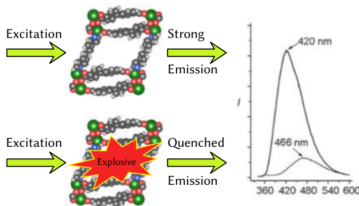
Figure 1.11 – Schematic representation of optical properties modifications of \text{Zn}_2(\text{bpdc})_2(\text{bpee}) MOF. Image adapted with permission from reference [39], copyright (2009) Wiley.
