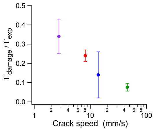
Figure 40: Evolution of \Gamma_{damage} / \Gamma_{exp} with the averaged crack velocity for crack propagation test on DAEAEA(2.3) at \dot{\lambda} = 3 \times 10^{-3} s^{-1} . \Gamma_{damage} calculated using U=64 kJ/mol
