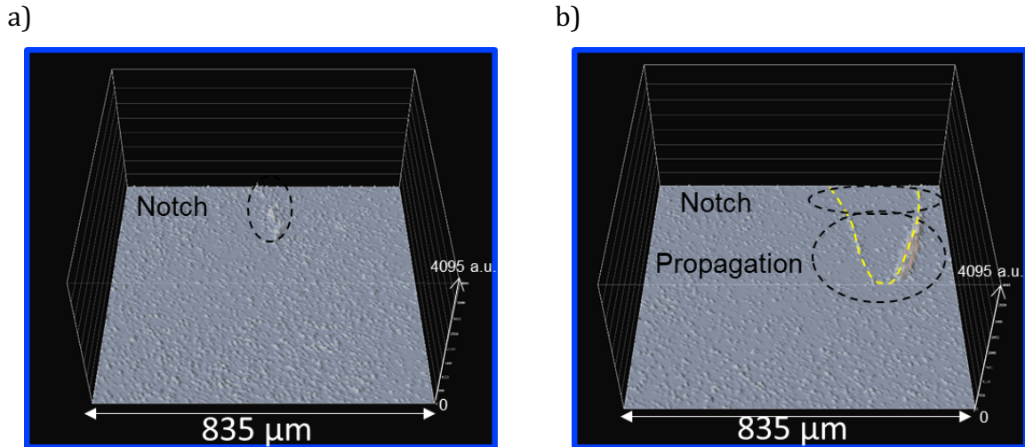
Figure 37: Surface intensity plots of single optical sections (5x, 835 μm x 835 μm, Laser 5 Gain 15) of EADAEA(2.5)(mechanophore in the 2 nd network) in the initial position (a) and after cyclic loading, after macroscopic crack propagation (b) Yellow dotted lines indicate crack edge. The crack is slightly opened as the reference position was defined slightly opened to better visualize edges.
