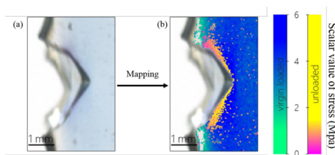
Figure 44: Raw image of a triple network ( \lambda_0 \sim 2.2 ) during crack propagation (a) and associated stress-color map of loading (green to blue) and unloading (pink to yellow)
