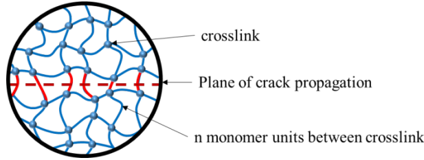
Figure 13: Schematic representation of Lake Thomas theory, red strands cross the crack plane
