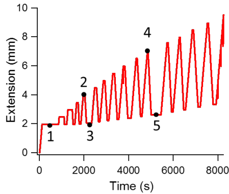
Figure 28: Cyclic test on notched sample and corresponding schematic representation of the sample. For cycles 1 to 4, an extension criteria was chosen to get back to the reference position (initial clamp position). From 5 th cycle, a force criteria was chosen ( F=0N ); as returning to the initial clamp displacement led to sample buckling because of slippage in the clamps.
