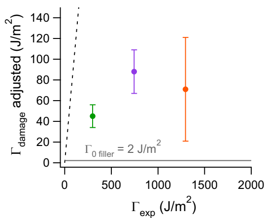
Figure 20: Evolution of \Gamma_{\text{damage}} adjusted (using U=64 \text{ kJ/mol} ) with \Gamma_{\text{exp}} for crack propagation test on DAMAEA(1.5) at different stretch rate: 3 \times 10^{-4} \text{ s}^{-1} (in green), 3 \times 10^{-3} \text{ s}^{-1} (in purple) and 3 \times 10^{-2} \text{ s}^{-1} (in orange). Average value calculated over 4 pictures, error bar correspond to the standard deviation. Dotted line corresponds to \Gamma_{\text{damage}} = \Gamma_{\text{exp}} curve.
