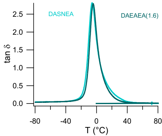
Figure 13: Evolution of \tan \delta with temperature, analyzed by DMA, for ethyl acrylate single (in green) and in a multiple network (in darker green)
