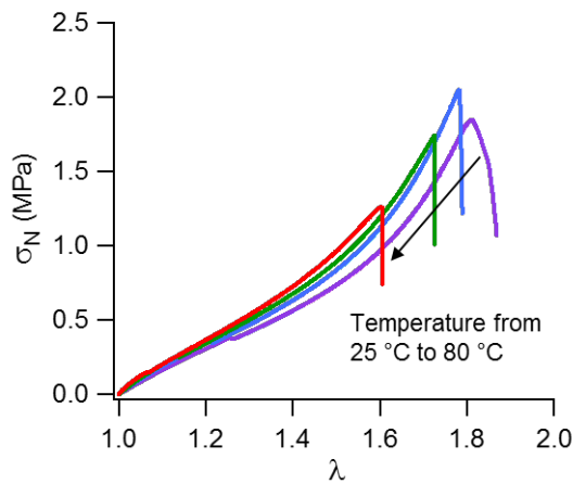
Figure 30: Examples of stress-strain curves of crack propagation tests on notched DAEAEA(2.3) at \dot{\lambda} = 3 \times 10^{-3} \text{ s}^{-1} and 25 °C (in purple), 40 °C (in blue), 60 °C (in green) and 80 °C (in red). One experiment was done on one DAEAEA(2.3) and one EAEA(2.3)
