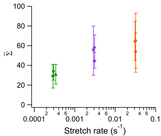
Figure 16: Evolution of the normalized number, \bar{\Sigma} , of broken chain as a function of the stretch rate in DASNMA. Average value calculated over 4 pictures, error bar correspond to the standard deviation. Different symbols correspond to samples from separate polymerizations.
