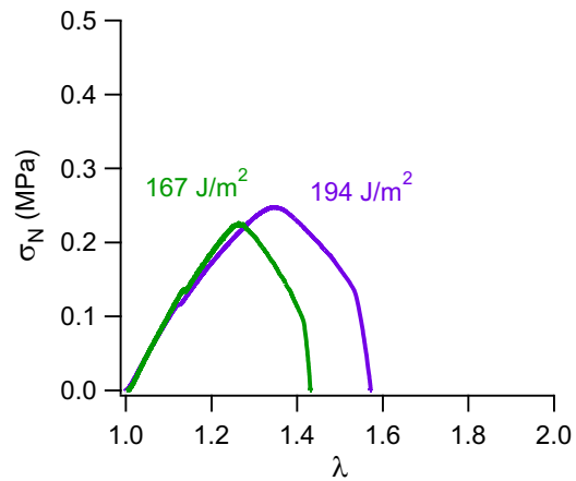
Figure 39: Stress-strain curve of crack propagation test on DASNEA at 25 °C (in purple) and DASNMA at 60 °C (in green) at \dot{\lambda} = 3 \times 10^{-3} \text{ s}^{-1} .
