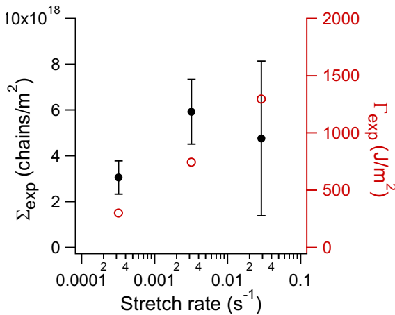
Figure 17: Evolution of the number, \Sigma_{exp} , of broken chain of the filler network (in black) and of the fracture energy, \Gamma_{exp} , (in red) as a function of the stretch rate.
