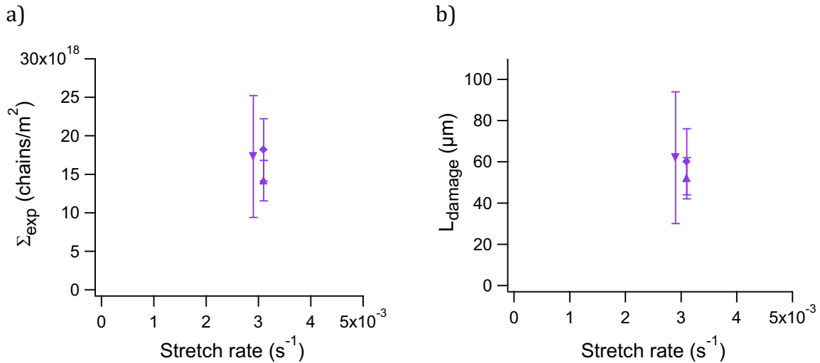
Figure 6: Reproducibility of the areal density of broken chains, \Sigma_{exp} (a) and the length, L_{damage} , over which damage was detected (b). Average value calculated over 4 pictures, error bar correspond to the standard deviation. Different symbols correspond to samples from separate polymerizations.
