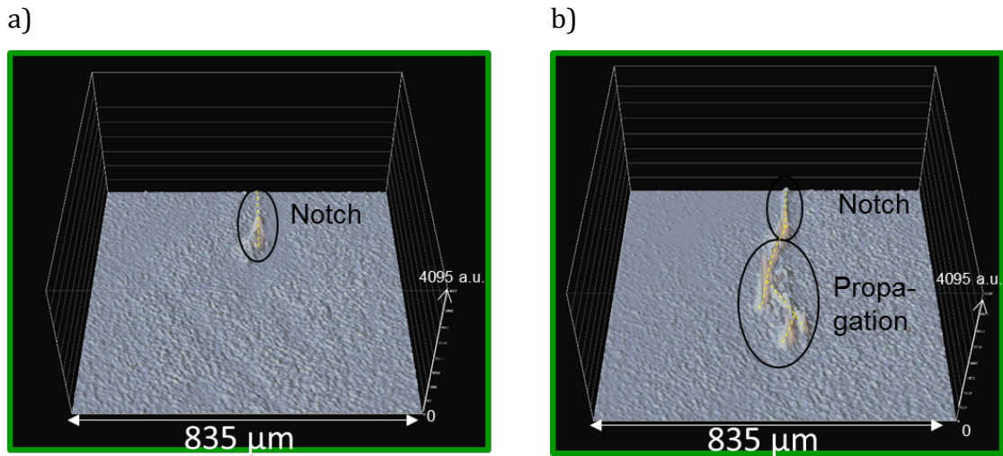
Figure 32: Surface intensity plots of single optical sections ( 5\times , 835\ \mu\text{m} \times 835\ \mu\text{m} , Laser 5 Gain 5) of DAEAEA(1.6) (mechanophore in filler network) in the initial position (a) and after cyclic loading, after macroscopic crack propagation (b) Yellow dotted lines indicate crack edge.
