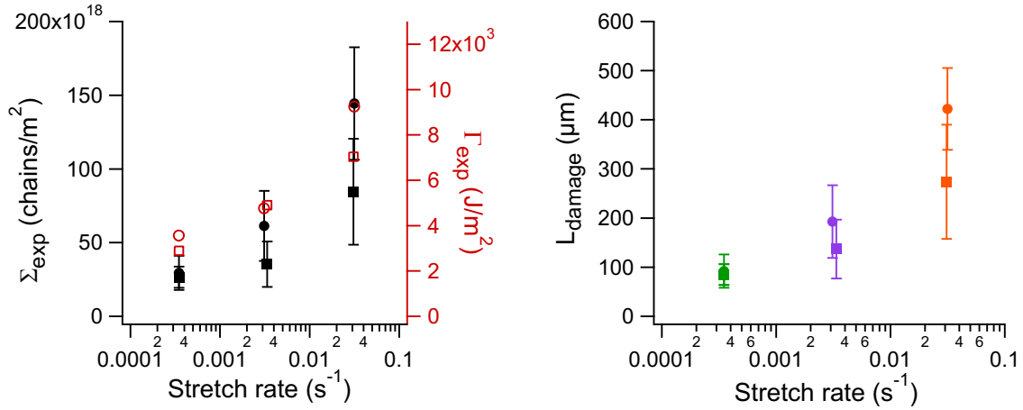
Figure 7: Evolution of the number, \Sigma_{exp} , of broken chain of the filler network (in black) and of the fracture energy, \Gamma_{exp} , (in red) as a function of the stretch rate in DAMAMA(1.6). Average value calculated over 4 pictures, error bar correspond to the standard deviation. Different symbols correspond to samples from different polymerizations.
