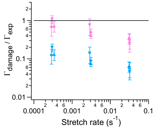
Figure 19: Evolution of \Gamma_{damage}/\Gamma_{exp} with the loading rate for crack propagation test on DASNMA at 25 °C. \Gamma_{damage} calculated using U_b=350 kJ/mol (in pink) and using U=64 kJ/mol (in blue)
