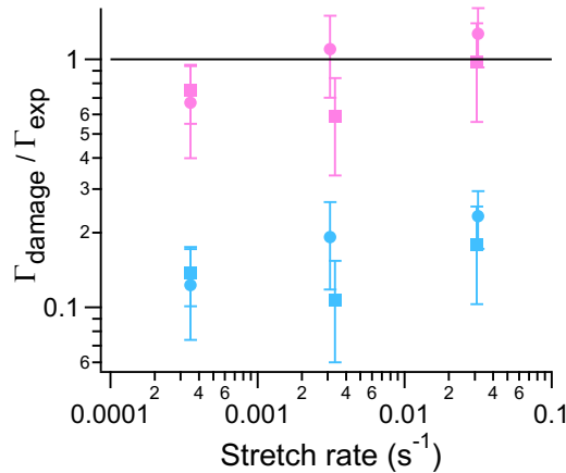
Figure 11: Evolution of \Gamma_{damage}/\Gamma_{exp} with the loading rate for crack propagation test on DAMAMA(1.6) at 25 °C. \Gamma_{damage} calculated using U_b=350 kJ/mol (in pink) and using U_b=64 kJ/mol (in blue)
