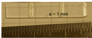
Figure 1: Picture of a sample before crack propagation test, with a the size of the initial notch and white dots for the extensometer
