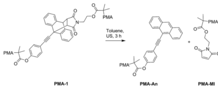
Figure 39: Retro Diels-Alder reaction on \pi -extended anthracene mechanophore
