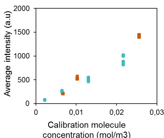
Figure 46: Evolution of the average intensity with the calibration molecule in PEA (in blue circle) and in PMA (in brown square).
