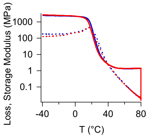
Figure 20: Storage (solid line) and loss modulus (dotted line) for a mechano-fluorescent sample (blue) and a reference sample (red)
