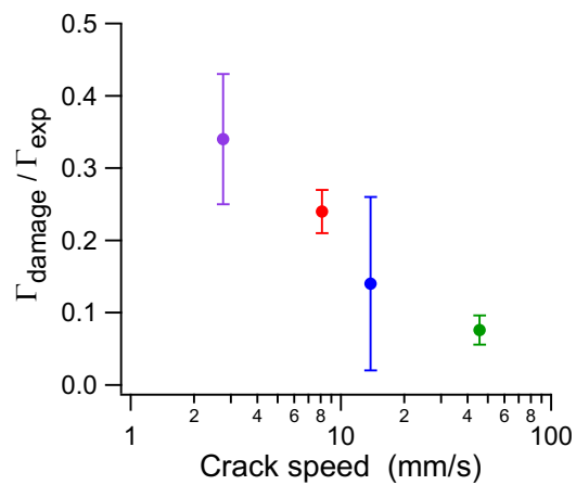
Figure 40: Evolution of \Gamma_{damage}/\Gamma_{exp} with the averaged crack velocity for crack propagation test on DAEAEA(2.3) at \lambda = 3 \times 10^{-3} \text{ s}^{-1} . \Gamma_{damage} calculated using U=64 \text{ kJ/mol}
