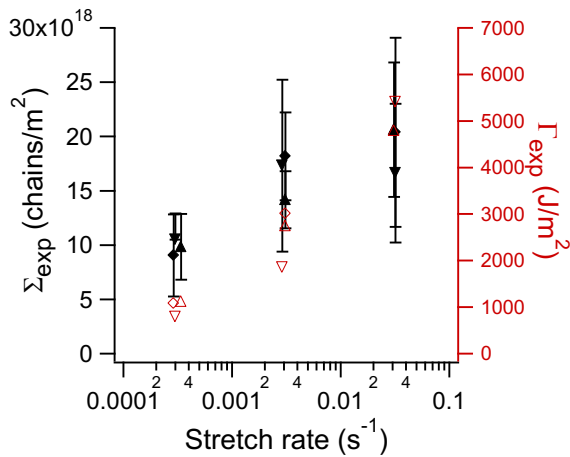
Figure 15: Evolution of the number, \Sigma_{exp} , of broken chain (in black) and of the fracture energy, \Gamma_{exp} , (in red) as a function of the stretch rate in DASNMA. Average value calculated over 4 pictures, error bar correspond to the standard deviation. Different symbols correspond to samples from separate polymerizations.
