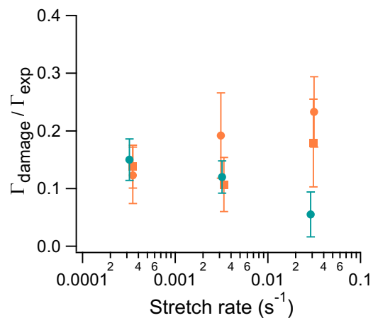
Figure 21: Evolution of \Gamma_{\text{damage}} / \Gamma_{\text{exp}} with the loading rate for crack propagation test on DAMAMA(1.6) at 25 \text{ }^\circ\text{C} (in orange) and DAMAEA(1.5) (in green). \Gamma_{\text{damage}} calculated using U_b=64 \text{ kJ/mol}
