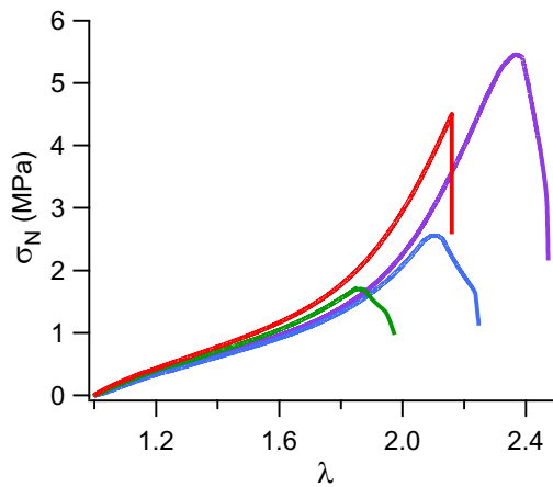
Figure 49: Example of stress-strain curves of crack propagation test on notched DAMAMA(2.3) at \dot{\lambda} = 3 \times 10^{-3} \text{ s}^{-1} and 25 °C (in purple), 40 °C (in blue), 60 °C (in green) and 80 °C (in red). Two DAMAMA(2.3) and one MAMA(2.3) were tested.
