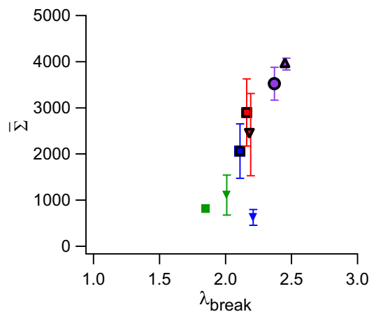
Figure 61: Evolution of \bar{\Sigma} with maximal strain before crack propagation in DAMAMA(2.3) at 50 \mu\text{m/s} and different temperature: 25 °C (in purple), 40 °C (in blue), 60 °C (in green) and 80 °C (in red). Means values calculated over 4 pictures, error bars correspond to the standard deviations. Different symbols correspond to sample from different polymerizations. Values at 25 °C and 80 °C are underestimated (off-limit).
