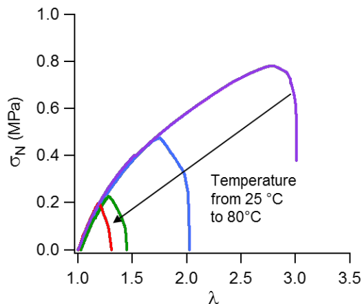
Figure 21: Example of stress strains curve of crack propagation test on notched DASNMA at \dot{\lambda} = 3 \times 10^{-3} \text{ s}^{-1} and at 25 \text{ }^\circ\text{C} (in purple), 40 \text{ }^\circ\text{C} (in blue), 60 \text{ }^\circ\text{C} (in green) and 80 \text{ }^\circ\text{C} (in red). One DASNMA and one SNMA were tested.
