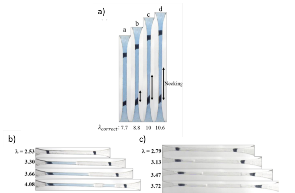
Figure 42: Uniaxial tensile test on quadruple network with the spiropyran incorporated in the first (a), the second (b) and in the third network (c)
