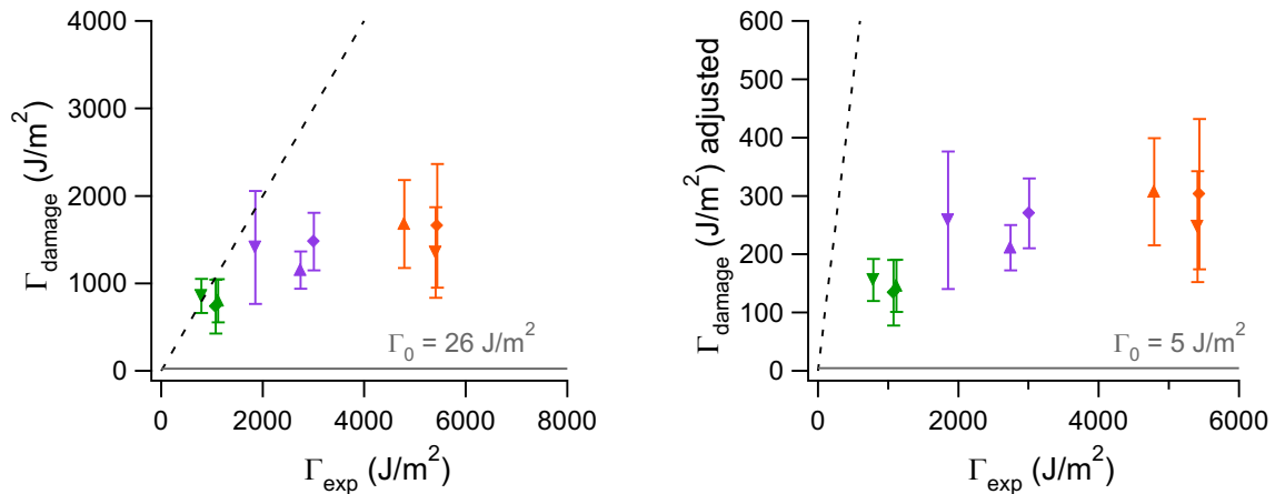
Figure 18 : Evolution of \Gamma_{damage} (using U_b=350 kJ/mol) (a) and \Gamma_{damage} adjusted (using U=64 kJ/mol) (b) with \Gamma_{exp} for crack propagation test on DASNMA at 25 °C and different loading rates \dot{\lambda} = 3 \times 10^{-4} \text{ s}^{-1} (in green), 3 \times 10^{-3} \text{ s}^{-1} (in purple) and 3 \times 10^{-2} \text{ s}^{-1} (in orange). Average value calculated over 4 pictures, error bar correspond to the standard deviation. Different symbols correspond to samples from separate polymerizations. Dotted line corresponds to \Gamma_{damage} = \Gamma_{exp} curve.
