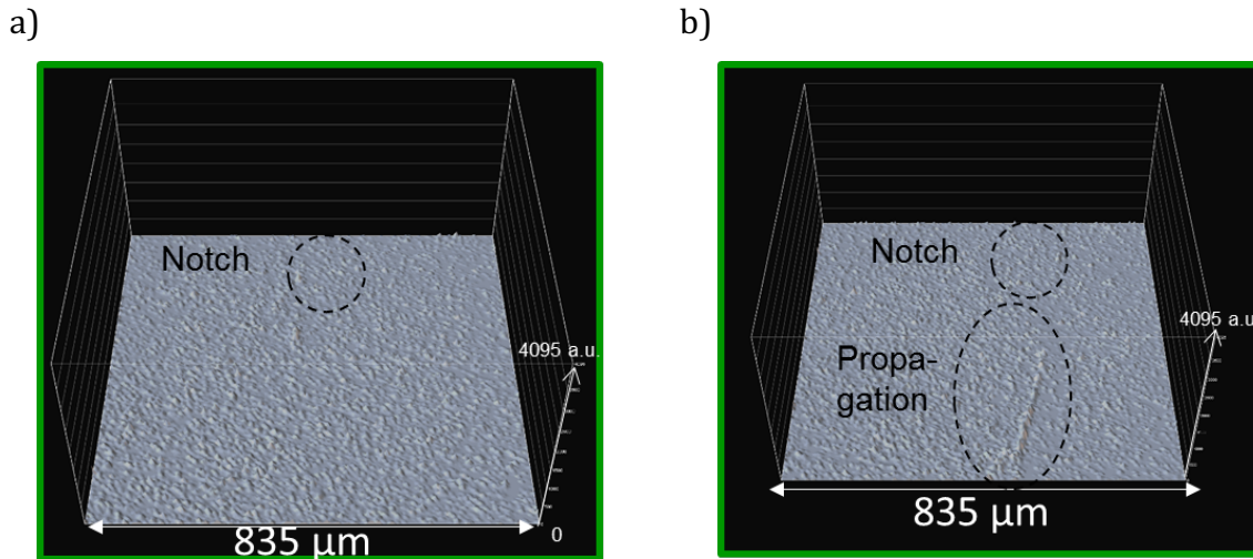
Figure 33: Surface intensity plots of single optical sections (5x, 835 μm x 835 μm, Laser 5 Gain 15) of EADAEA(1.6)(mechanophore in the 2 nd network) in the initial position (a) and after macroscopic crack propagation (b)
