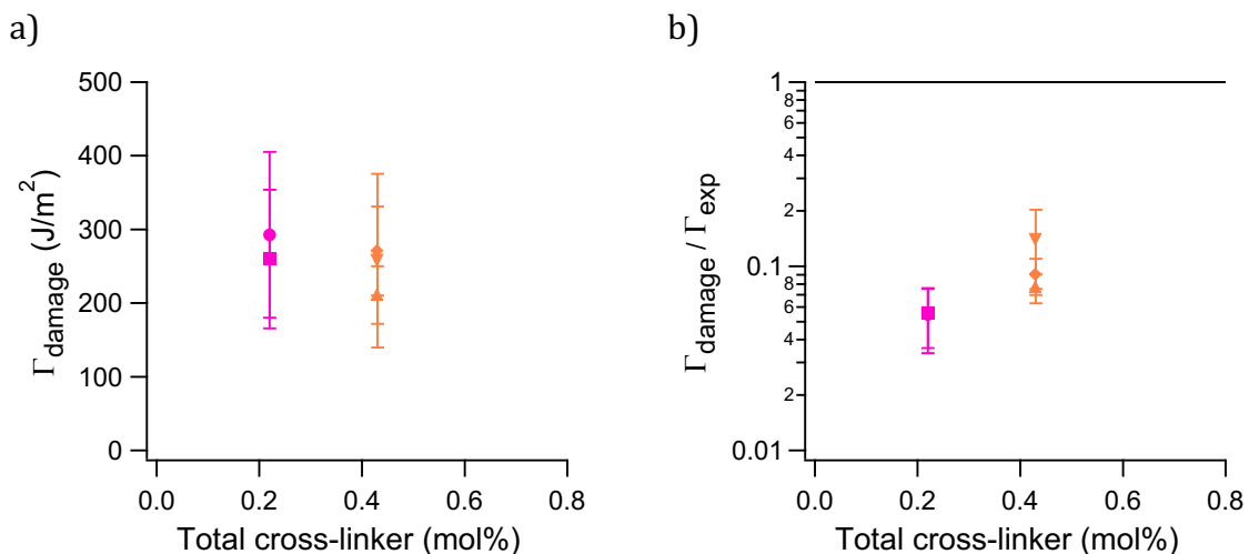
Figure 38: Evolution of \Gamma_{damage} (a) and \Gamma_{damage}/\Gamma_{exp} (b) for crack propagation test on DASNMA (orange) and DASNMA 0.2 (pink) at 25 °C and \dot{\lambda} = 3 \times 10^{-3} s^{-1} . \Gamma_{damage} calculated using Craig's assumption ( U=64 kJ/mol). Average value calculated over 4 pictures, error bar correspond to the standard deviation. Different symbols correspond to samples from separate polymerizations.
