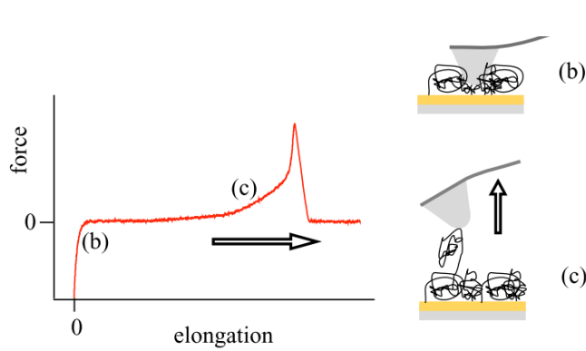
Figure 6: Schematic of a single molecule force spectroscopy experiment, upon retraction of the cantilever the polymer chain is stretched while force and elongation are recorded
