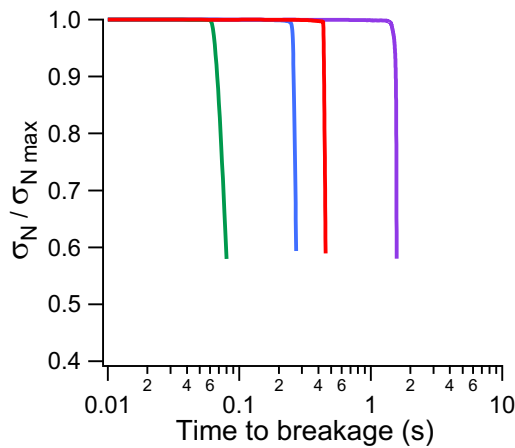
Figure 39: Normalized stress as a function of time during crack propagation in DAEAEA(2.3) at \lambda = 3 \times 10^{-3} \text{ s}^{-1} and 25 °C (in purple), 40 °C (in blue), 60 °C (in green) and 80 °C (in red)
