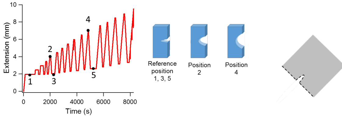
Figure 28: Cyclic test on notched sample and corresponding schematic representation of the sample. For cycles 1 to 4, an extension criteria was chosen to get back to the reference position (initial clamp position). From 5 th cycle, a force criteria was chosen ( F=0N ); as returning to the initial clamp displacement led to sample buckling because of slippage in the clamps.
