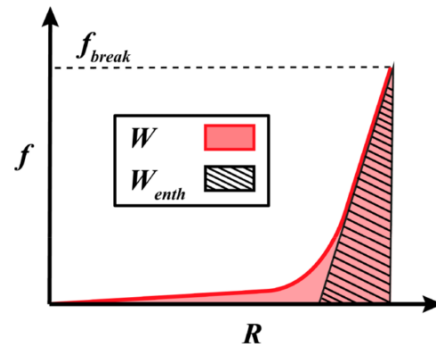
Figure 7: Work done to extend a polymer chain ( W ) is the area under the force vs. end-to-end distance curve. The enthalpic part is the area shaded by black lines.
