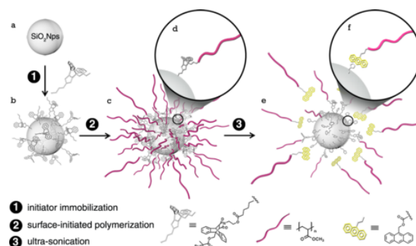
Figure 38: Anthracene-maleimide mechanophore at the interphase between nanoparticle and polymer
