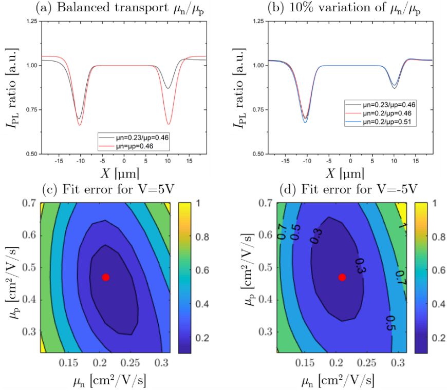
Figure 6-5 Variations of the PL ratio and reconstruction error for different couples (\mu_n, \mu_p) . (a) I_{PL} ratio simulated for \mu_n = \mu_p = 0.46 \text{ cm}^2/\text{V/s} and for \mu_p = 0.46 & \mu_n = 0.23 \text{ cm}^2/\text{V/s} . (b) I_{PL} ratio simulated for small variations of \mu_n or \mu_p around the fitted point. (c) Variations of the reconstruction error at V=5\text{V} . A lower reconstruction error indicates a better fit. A red point designates the optimal point. ((d) for opposite bias)
