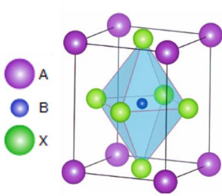
Figure 1-6 Generic perovskite crystal structure ( ABX_3 ).
