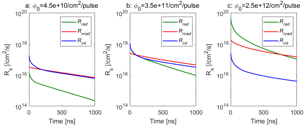
Figure 4-10 Temporal evolution of recombination terms simulated for perovskite P 2 at the same excitations powers employed during TRPL decay (a: \Phi_{0,1} b: \Phi_{0,2} c: \Phi_{0,3} ) These terms are defined in eq. (4-16), (4-17) & (4-18)
