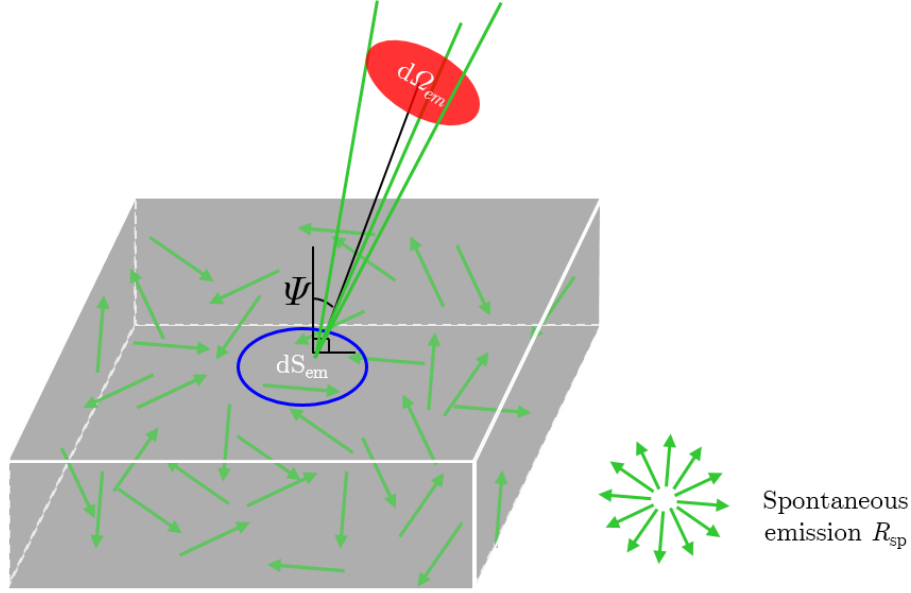
Figure 1-2 Volume of semi-conductor material and photons in equilibrium, in which the spontaneous emission R_{\text{sp}} and from which a photon flux j_{\gamma} is emitted through dS_{\text{em}} in the direction d\Omega_{\text{em}} .
