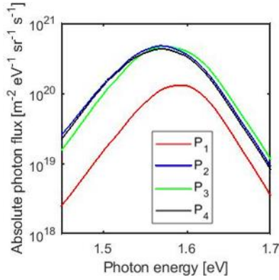
Figure 4-2 Absolute PL spectrum for the considered perovskite samples, optically excited at \lambda = 532 \text{ nm} at \Phi_0 = 5.5 \times 10^3 \text{ W}\cdot\text{m}^{-2} .
