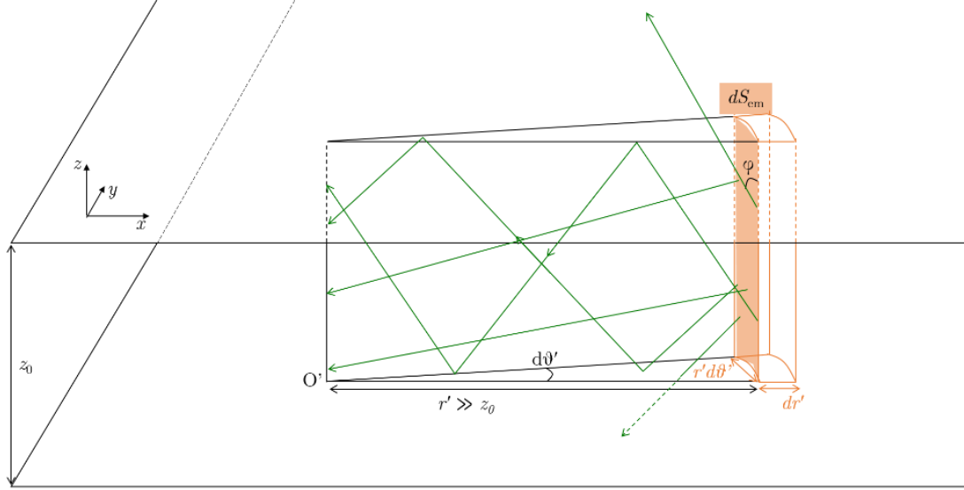
Figure 5-7 Geometrical sketch of the elementary volume dV in the long-range scenario, showing the photons (green rays) emitted in dV (orange), towards the origin of a secondary frame, where the recycling term g_{\text{rec}} is calculated. Various solid angles of emission ultimately propagate towards the origin thanks to total internal reflection at front and back interfaces for \varphi_c < \varphi < \pi - \varphi_c .
