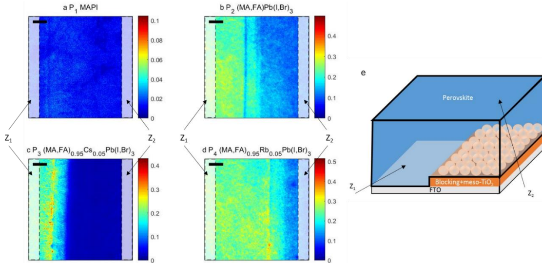
Figure 4-3 Photoluminescence images taken 10 ns after the laser pulse I_{\text{PL}}(x,y,t=10\text{ns}) in arbitrary units for different compositions considered throughout this study ( P_1 to P_4 from a to d). On the left of each image, Z_1 appears with a whitish framed area, while, Z_2 appears on the right. (e) summarizes the sample structure investigated. Scaling bar is 100\mu\text{m} long
