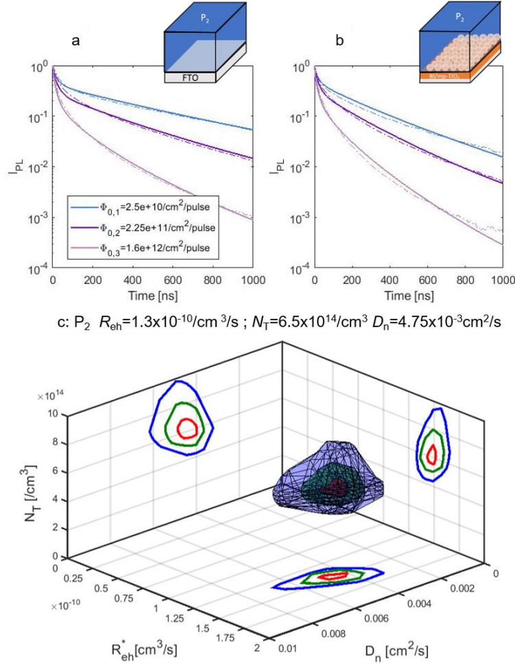
Figure 4-7 (a)-Experimental (dotted lines) and numerically fitted (plain lines) I_{PL} decays for a mixed cation perovskite MA_{0.17}FA_{0.83}Pb(I_{0.83}Br_{0.17})_3 (also P_2 ) layer deposited on FTO (A) or on mesoporous- TiO_2 (b). Various orders of magnitude of the fluence level \Phi_0 have been tested. (c) Iso-surfaces showing a set of parameters ( R_{eh}^* , D_n , N_T ) leading to a reconstruction error not higher than 10% (red), 20% (green), 50% (blue) of the optimal reconstruction error. The green one is used for confidence intervals indicated in Table 4-1.
