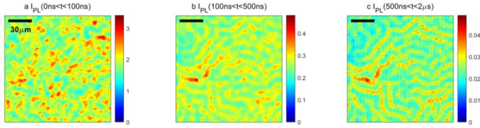
Figure 5-18 Temporal aspect of multi-dimensional PL imaging of a wrinkle-containing perovskite sample, showing the temporal evolution of PL signal after the laser pulse (at t=0 ns).
