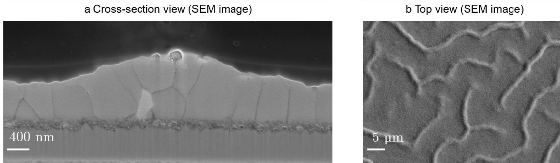
Figure 5-16 Morphological properties of a wrinkle-containing perovskite sample. Focused Ion Beam was used to observe a cross-section SEM of a perovskite PV device (B) SEM image (top-view) of a similar perovskite layer deposited on FTO/bl-TiO 2 /mp-TiO 2
