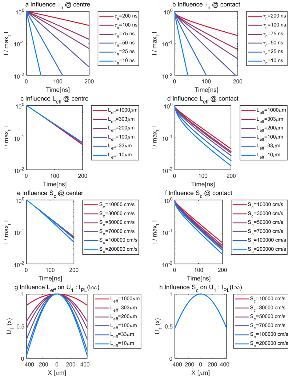
Figure 3-6 Simulations of I_{PL} transients/profiles according to eq. (3-8) at the center of the cell (a,c,e) and at the contact (b,d,f). \tau_n is varied in (a,b). L_{\text{eff}} is varied in (c,d), and S_c is varied in (e,f). Simulations of PL profile at long times according to eq. (3-9) for L_{\text{eff}} and S_c variation. When one parameter is varied, others stay at the following values: L_{\text{eff}}=200\mu\text{m} , S_c=5 \cdot 10^4 \text{cm/s} , \tau_n=75\text{ns} .
