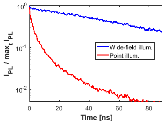
Figure 3-9 I_{PL} transient for a wide-field illumination and a local excitation taken in between fingers, integrated on a 10\ \mu\text{m} \times 10\ \mu\text{m} square ( \Phi_0=3 \times 10^{12} /pulse/cm 2 in WF & \Phi_0=2 \times 10^{14} /pulse/cm 2 in point illumination).
