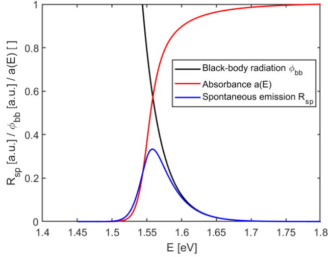
Figure 1-1 Gray-body radiation decomposed as the product of absorptivity a(E) and black-body radiation. Calculation is done for E_g = 1.55\text{eV} , E_u = 15\text{meV} , \Theta = 1.5 , u_0 = 10 (see section 1.1.4 for more details on spectrum)
