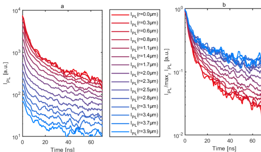
Figure 5-4 I_{PL} decays of a perovskite sample after point pulsed illumination at incremental distances from the illumination point(a), also normalized to their maximum at t=0 ns in (b)
