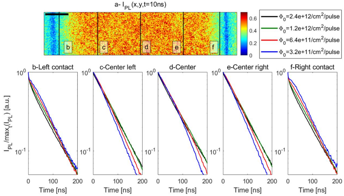
Figure 3-2 Photoluminescence image of a GaAs solar cell at open-circuit conditions (a). It is taken at t=10\text{ns} after the laser pulse. The scaling bar is 100\ \mu\text{m} . Each black line corresponds to an extraction zone for the normalized TRPL decays shown in b-e. Several decays are represented with a color for each power \Phi_0 (see caption on the top right corner)
