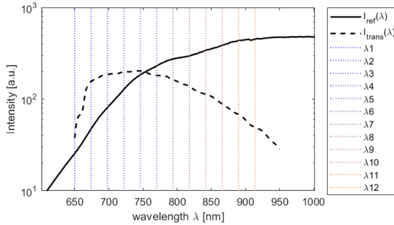
Figure 2-3 Reference spectrum of the calibration lamp, and measured spectrum I_{\text{trans}} (spatially averaged). 12 characteristic wavelengths used also used in Figure 2-4 are indicated by straight colored lines.
