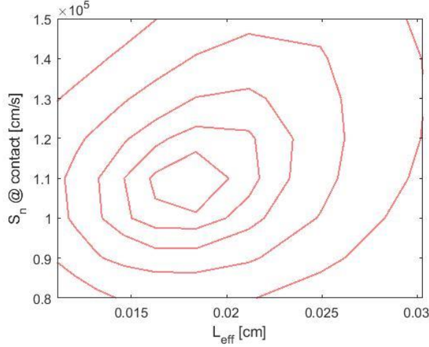
Figure 3-8 Reconstruction error between the experimental transient and the theoretical model calculated with the least square method. This corresponds to n_0=1.2 \times 10^{12} /cm 2 /pulse and \tau_n=75 ns. Contour lines limit an area where the reconstruction error does not rise by more than 10 %; 25 %; 50 %; 100 %; 200 %
