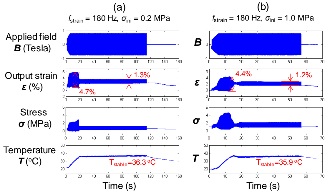
Figure 3.4 Typical responses of Ni-Mn-Ga under the same frequency f_{strain} = 180 Hz ( f_{mag} = 90 Hz) with different initial compressive stress: (a) \sigma_{ini} = 0.2 MPa and (b) \sigma_{ini} = 1.0 MPa.
