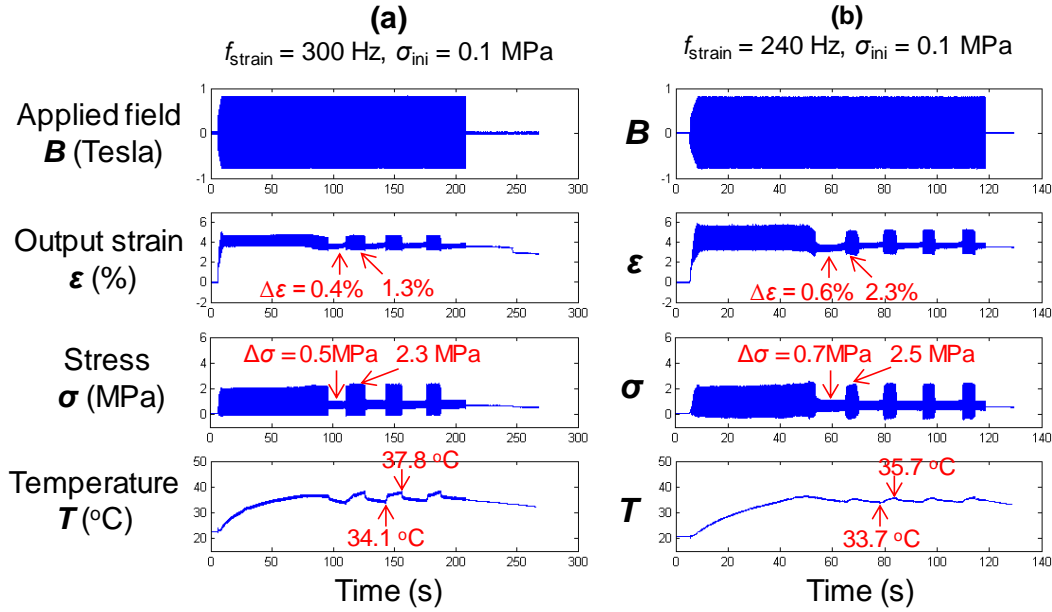
Figure 3.17 Oscillation phenomenon observed in the tests at the low initial compressive stress \sigma_{ini} = 0.1 MPa: the strain amplitude \Delta\epsilon and the stress amplitude \Delta\sigma periodically switch between two “stabl” states.
