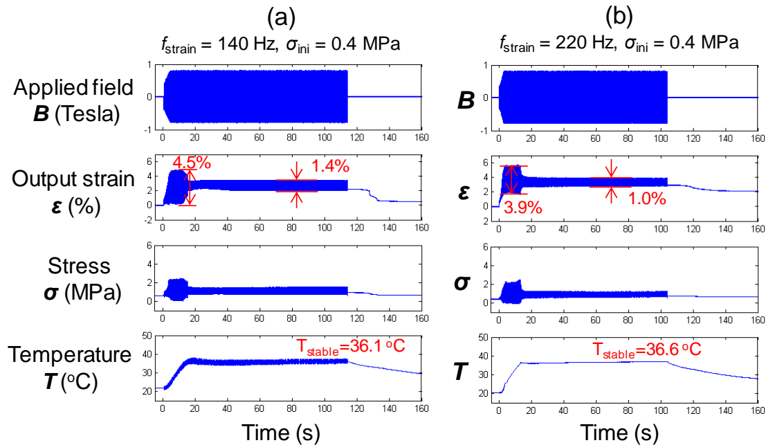
Figure 3.3 Typical responses of the Ni-Mn-Ga specimen under the same initial compressive stress \sigma_{ini} = 0.4\text{ MPa} with different frequency: (a) f_{strain} = 140\text{ Hz} ( f_{mag} = 70\text{ Hz} ) and (b) f_{strain} = 220\text{ Hz} ( f_{mag} = 110\text{ Hz} ).
