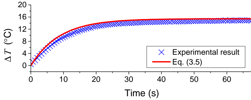
Figure 3.12 Comparison of the temperature rise between Eq. (3.5) and the experimental data from the test of f_{strain} = 180 Hz, \sigma_{ini} = 0.4 MPa and V_{air} = 15 m/s ( t_h = 8.8 s), whose responses of the strain and the stress can be found in Fig. 3.7(c).
