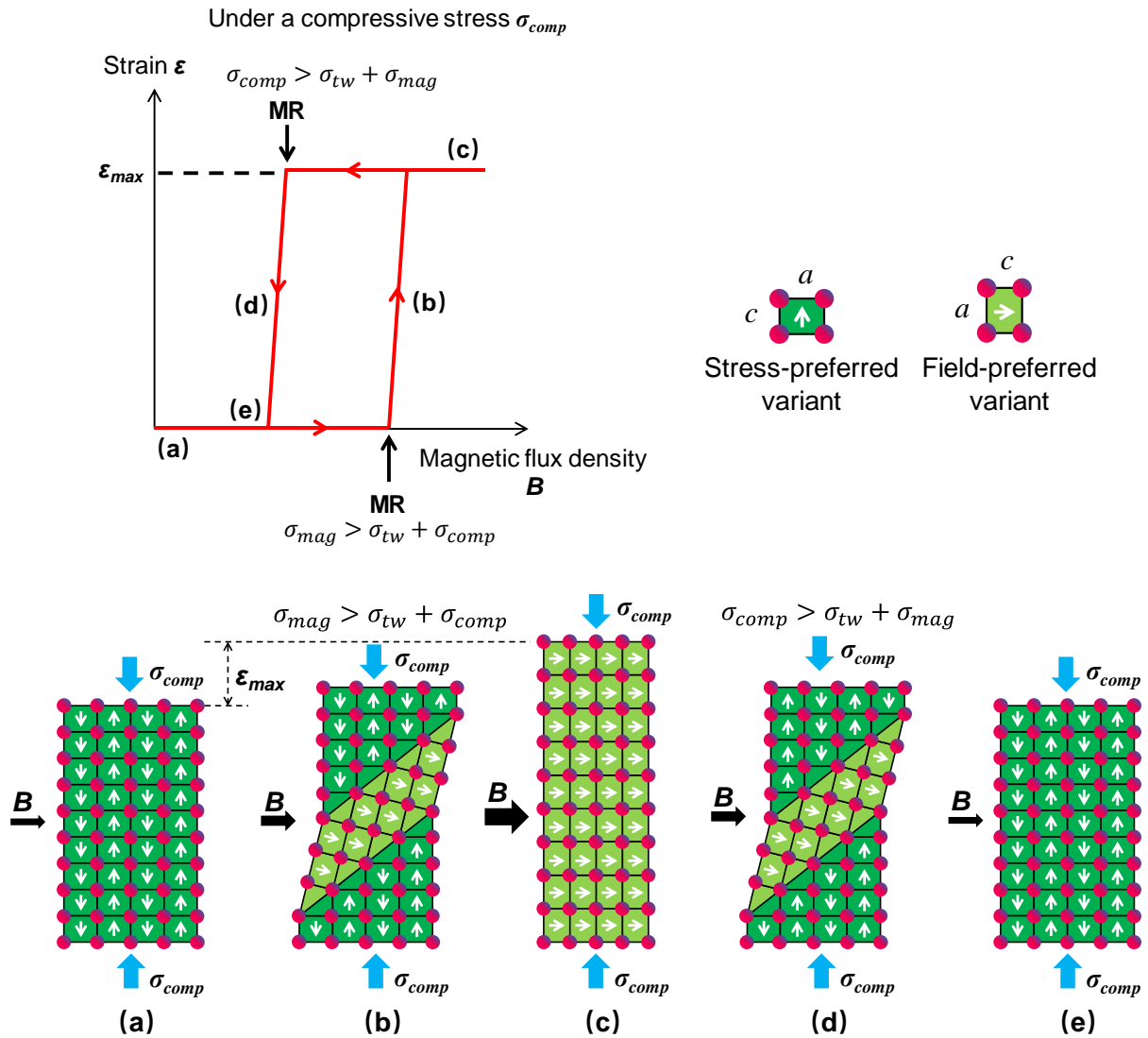
Figure 1.5 Schematic of magneto-mechanical loading-induced reversible martensite reorientation.
