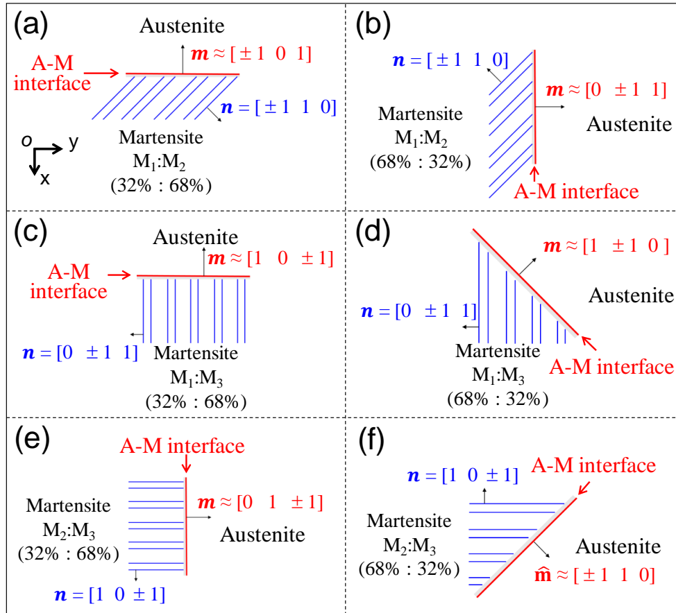
Figure 4.5 Theoretical predictions of all the possible patterns of A-M interface and martensite fine-twins (projections on x - y plane). The patterns in (a) and (b) are formed by fine twins of M_1:M_2 , (c) and (d) are formed by fine twins of M_1:M_3 , (e) and (f) are formed by fine twins of M_2:M_3 .
