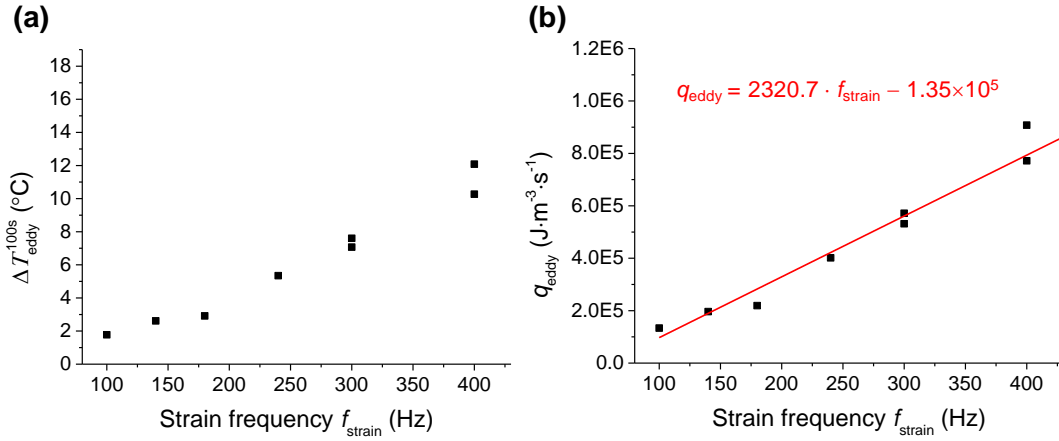
Figure 3.11 The temperature rise due to eddy current after the actuation of 100 s at different strain frequencies f_{strain} are shown in (a) and the corresponding heat generation rate is shown in (b).
