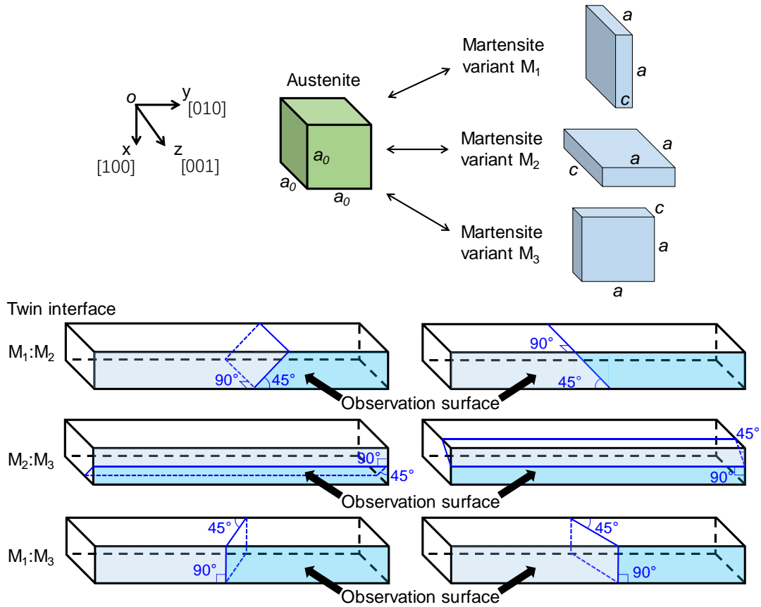
Figure 4.4 Twin boundaries of the tetragonal martensite variants of Ni-Mn-Ga. The x - y plane (the experimentally observed surface) is shown in color in each 3D schematic, where different colors represent different variants.
