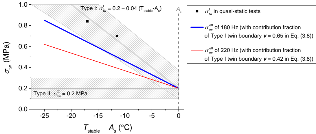
Figure 3.13 The temperature dependence of twinning stress for the twin boundary motion during the magneto-mechanically driven martensite reorientation. The two shaded regions represent the temperature dependence of the twinning stresses of the Type I and Type II twin boundaries, respectively, reported in (Heczko and Straka, 2003; Soroka et al., 2018; Sozinov et al., 2017; Straka et al., 2012; Zreihan et al., 2015). The thick blue and thin red lines (determined by Eq. (3.8) with \nu = 0.65 and 0.42 respectively) represent the temperature dependences of the effective twinning stress of the mixed Type I and Type II twin boundaries in the dynamic actuation of f_{strain} = 180 Hz and f_{strain} = 220 Hz, respectively.
