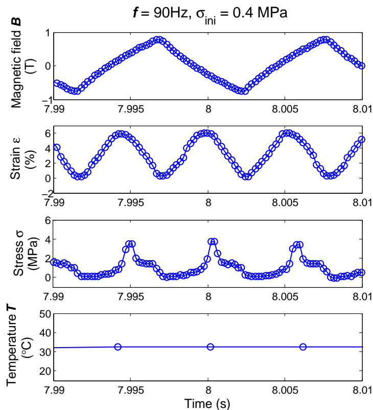
Figure 2.2 Typical acquired data sets of a cyclic dynamic test.
