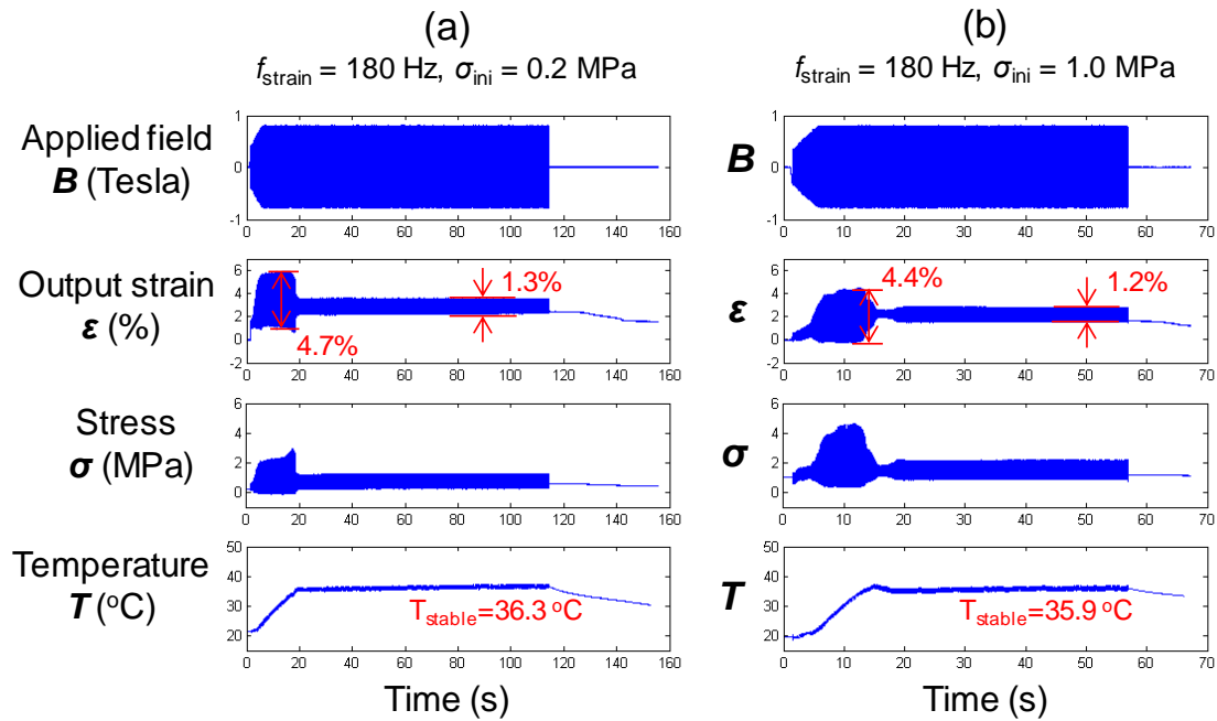
Figure 3.4 Typical responses of Ni-Mn-Ga under the same frequency f_{strain} = 180 Hz ( f_{mag} = 90 Hz) with different initial compressive stress: (a) \sigma_{ini} = 0.2 MPa and (b) \sigma_{ini} = 1.0 MPa.
