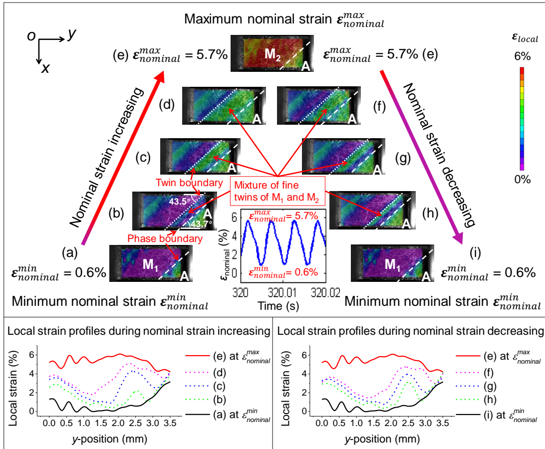
Figure 4.3 DIC local strain evolutions in a typical cycle of the martensite reorientation process with the existence of the non-active A-phase (the green region of A-phase (at lower right corner in each DIC map) has a constant local strain around 4%) at the time slot t_6 .
