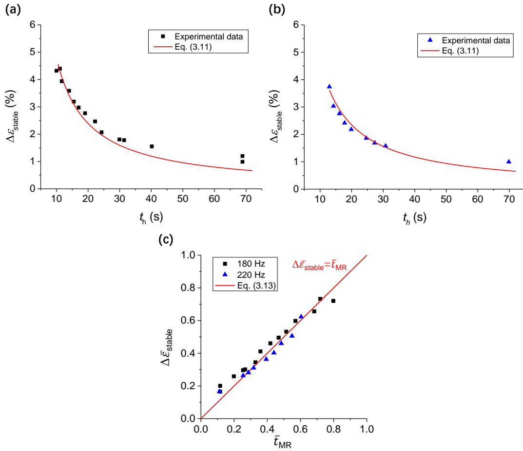
Figure 3.15 The comparison between the theoretical model (Eq. (3.11)) and the experimental data for the tests at f_{strain} = 180 Hz (a) and 220 Hz (b). (c) The comparison between the normalized model (Eq. (3.13)) and the normalized experimental data of f_{strain} = 180 and 220 Hz in terms of \Delta\bar{\epsilon}_{stable} and \bar{t}_{MR} .
