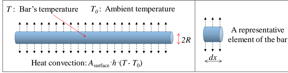
Figure 3.9 One-dimensional heat-transfer model
