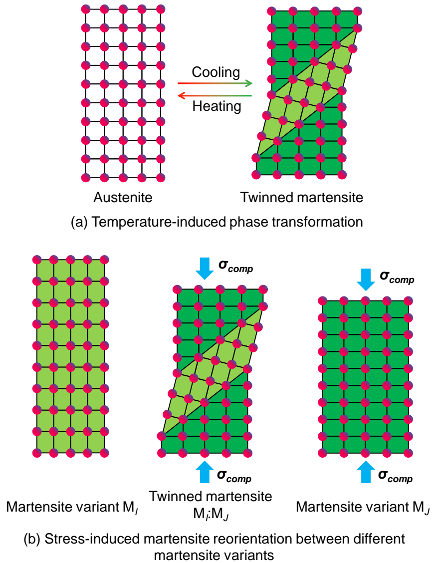
Figure 1.2 Schematics of (a) phase transformation and (b) martensite reorientation.
