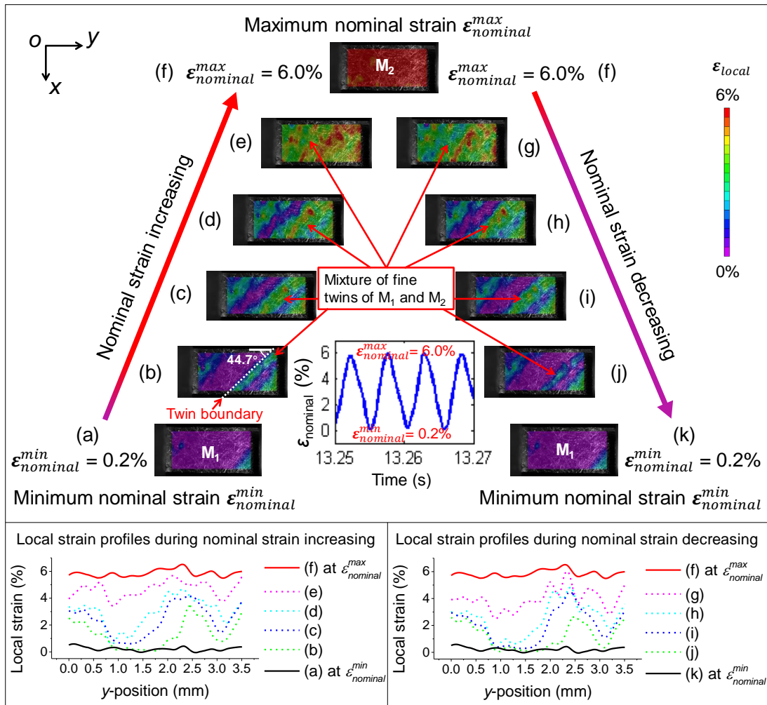
Figure 4.2 DIC local strain evolutions in a typical cycle of the martensite reorientation process before the occurrence of the strain drop phenomenon (pure martensite phase) at the time slot t_1 .
