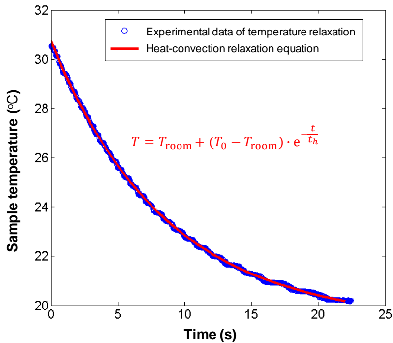
Figure 2.3 Temperature relaxation of Ni-Mn-Ga single crystal sample ( 2 \times 3 \times 15 mm) under the ambient airflow of 15 m/s. The fitted characteristic heat-relaxation time t_h is 8.8 s.
