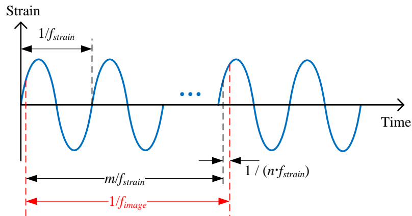
Figure 2.4 Schematic of the optical imaging method during high-frequency deformation.
