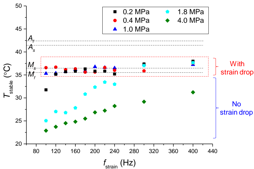
Figure 3.6 Stable temperatures T_{stable} of all tests conducted in still air with different loading conditions (different strain frequencies and initial compressive stresses). The cases with strain drop are marked by the red dashed rectangle.
