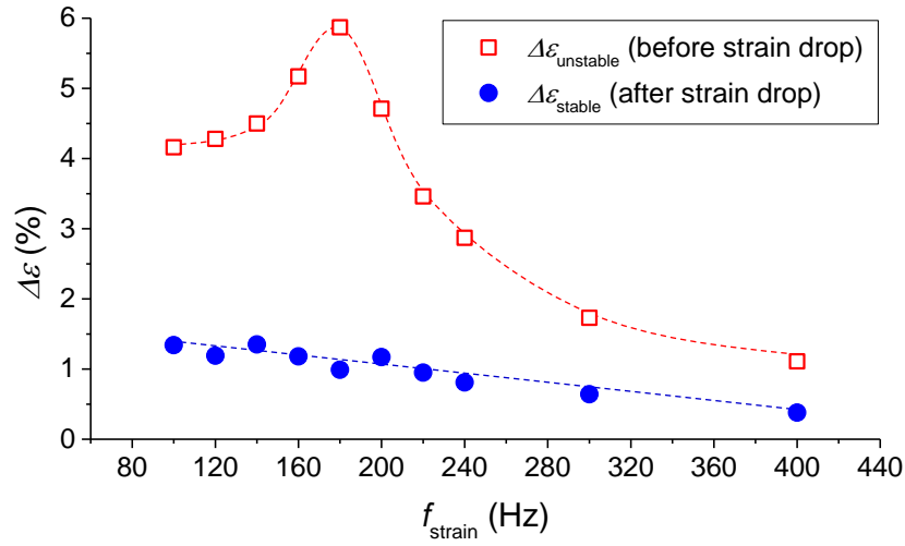
Figure 3.5 The frequency-dependent stable and unstable strain amplitudes of the tests with the initial compressive stress \sigma_{ini} = 0.4 MPa in still air. \Delta\epsilon_{unstable} and \Delta\epsilon_{stable} represent the strain amplitudes of the short-time actuation (before strain drop) and the long-time actuation (after strain drop), respectively. The dashed lines are for guiding eyes.
