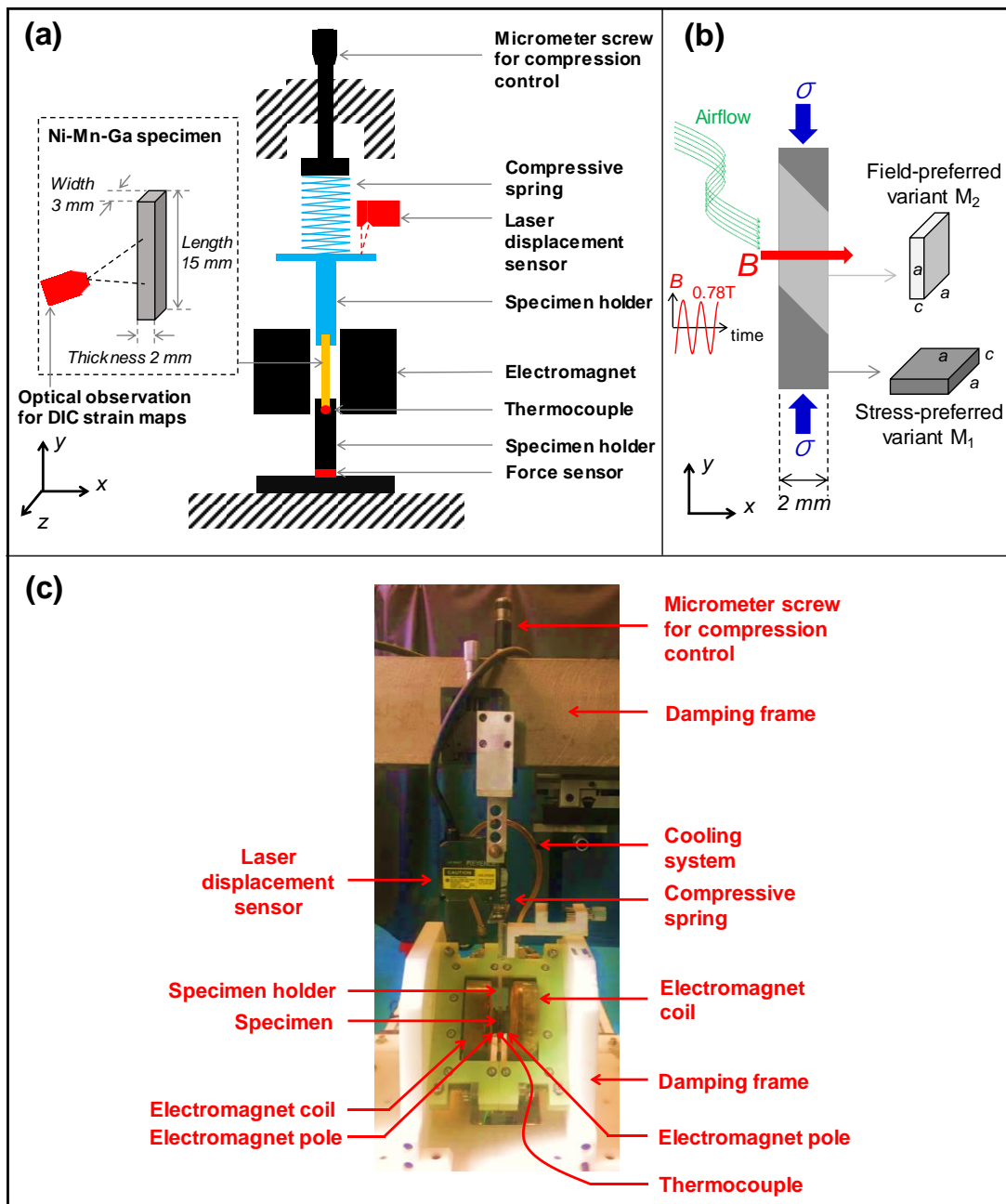
Figure 2.1 (a) Schematic of actuation system to achieve high-frequency cyclic martensite reorientation, where the fixed parts (immobile components) during the dynamic actuation are in black, the moving parts (the spring and the upper sample holder) are in blue and the measuring sensors are in red. (b) Schematic of the martensite reorientation between the stress-preferred martensite variant ( M_1 ) and the magnetic-field-preferred martensite variant ( M_2 ) in Ni-Mn-Ga specimen under the magneto-mechanical actuation. Approximated tetragonal martensite variant of one short axis ( c -axis) and two long axes ( a -axis) are adopted and the difference between a and c is shown exaggeratedly here. (c) Photo of the experimental setup for high-frequency magnetic actuation.
