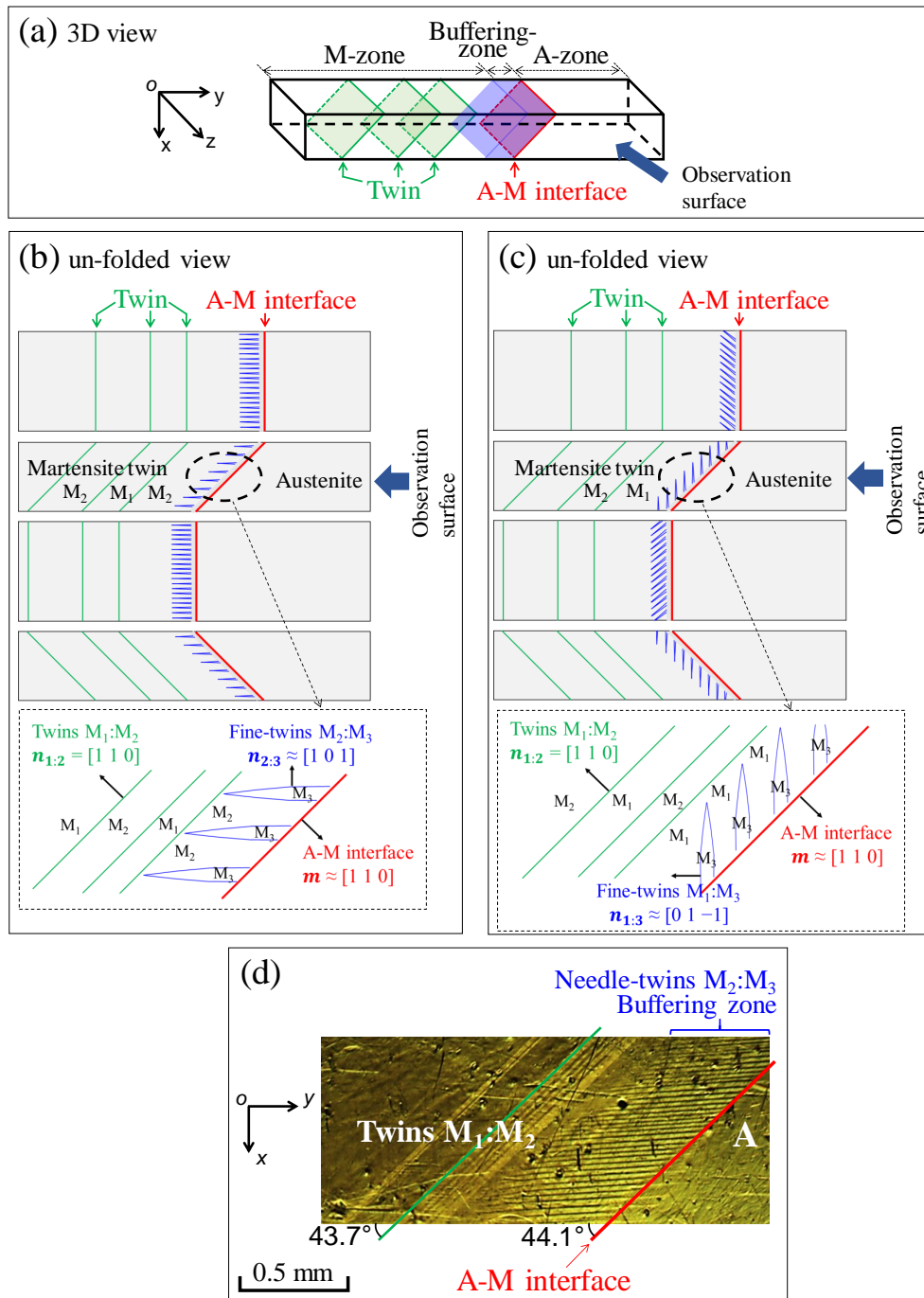
Figure 4.6 The 3D and unfolded schematics and of the compatible microstructures with the coexistence of non-active austenite zone, buffering needle zone and active martensite zone in (a) ~ (c); (d) The optical observation of the needle fine-twins jointly generated with A-M interface in a quasi-static thermo-mechanical test.
