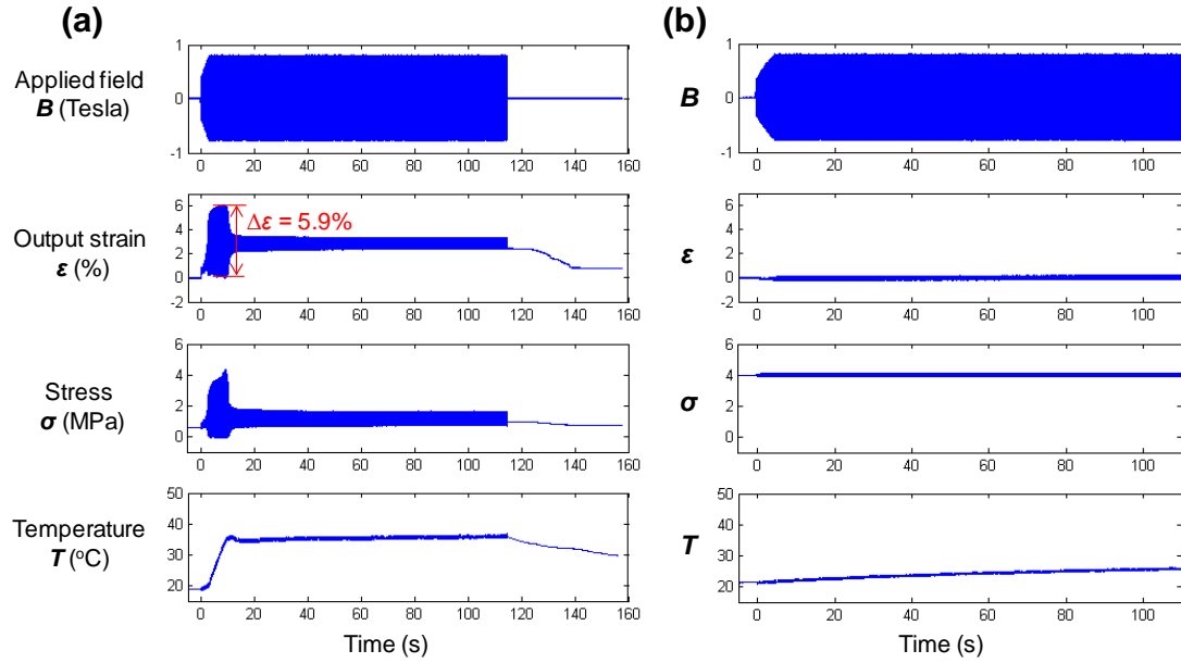
Figure 3.10 Typical tests to compare the temperature rises induced by the martensite-reorientation dissipation and the eddy current at the strain frequency f_{strain} = 180 Hz, with the different initial compressive stresses: (a) 0.4 MPa and (b) 4.0 MPa.
