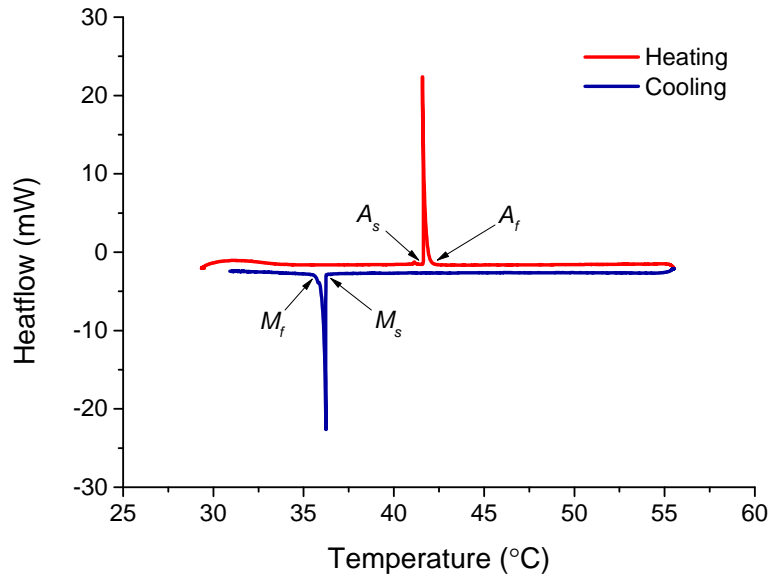
Figure 3.1 DSC curves of the single-crystal Ni-Mn-Ga at the heating/cooling rate of 0.5 °C/min.
