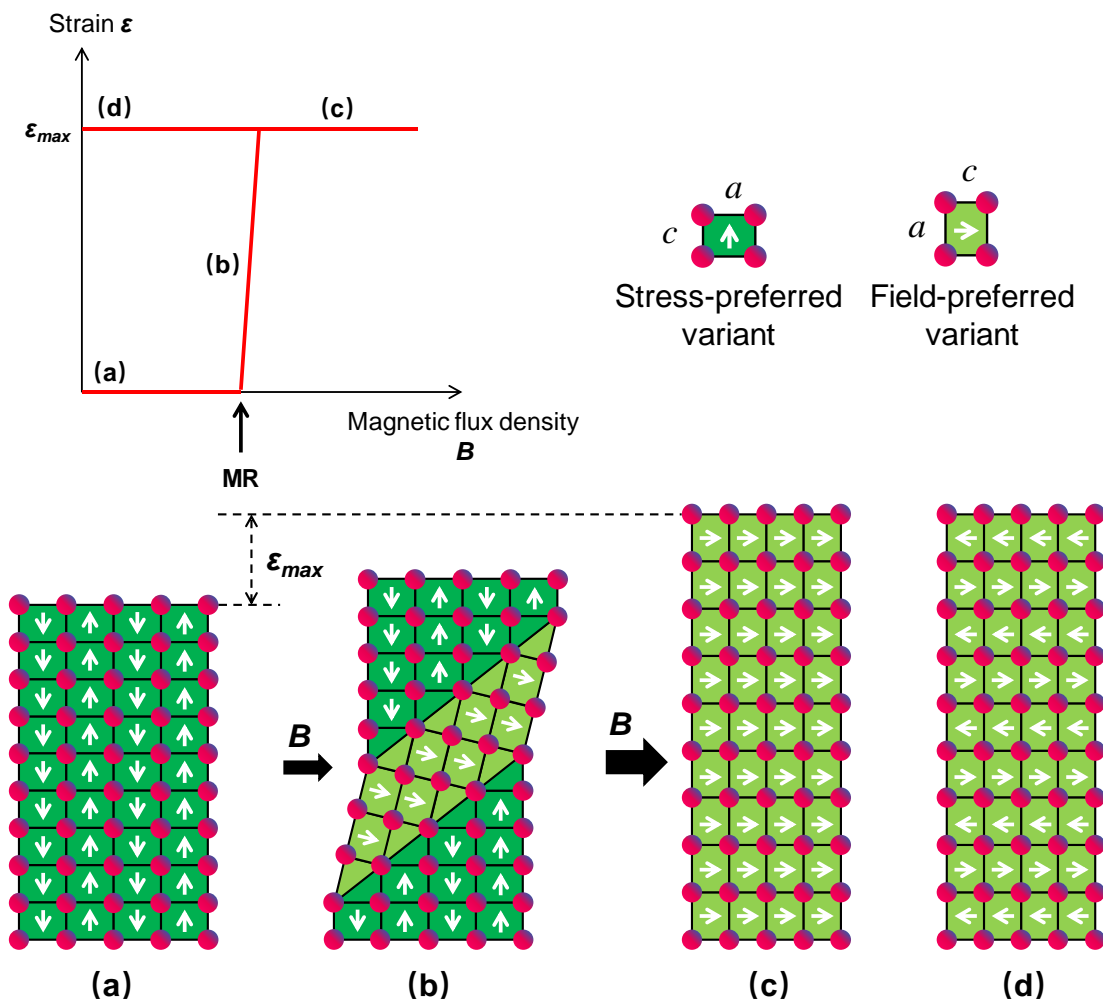
Figure 1.4 Schematic of magnetic field-induced martensite reorientation.
