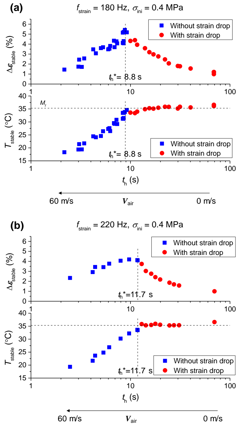
Figure 3.8 Airflow-dependence ( t_h -dependence) of the stable strain amplitude \Delta \epsilon_{stable} and the stable temperature T_{stable} for all the tests with ambient airflow of different velocities for the two typical loading frequencies: (a) f_{strain} = 180 \text{ Hz} and (b) f_{strain} = 220 \text{ Hz} .
