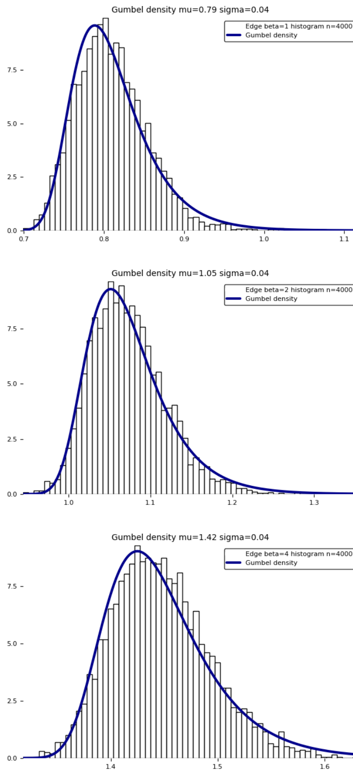
Figure 7.6 – Study of the fluctuation of the largest particle in modulus for the \beta complex Ginibre ensemble with N = 50 , in the cases \beta \in \{1, 2, 4\} . The solid line is the plot of the fit with a translation-scale Gumbel distribution. The Gumbel fluctuation is proved only in the case \beta = 2 , see [365, 86]. These simulations suggest to conjecture that the Gumbel fluctuation is valid for any \beta > 0 . The simulation matches pretty well the edge support at \sqrt{\beta/2} and suggests that the variance is not very sensitive to \beta .
