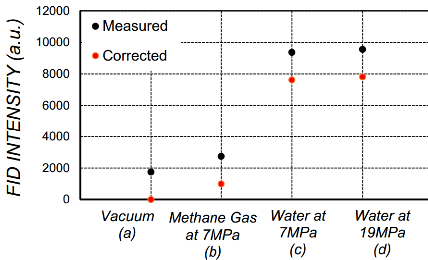
Figure 4.3: Reference signal.
