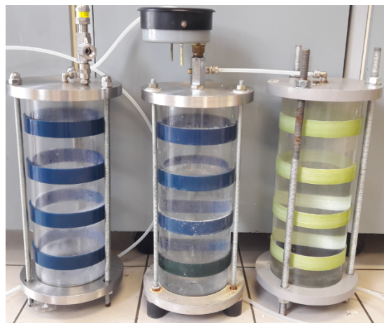
Figure 3.6: The system to measure methane gas quantity released from MH dissociation.
