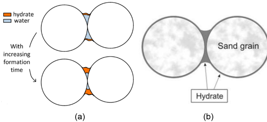
Figure 2.27: (a) Mechanism of the MH formation at grain contacts (Pinkert and Grozic, 2014); (b) MH distribution at the grain scale (Priest et al., 2009).
