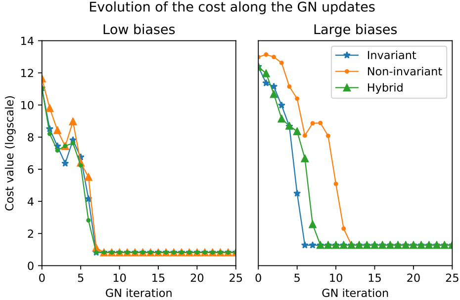
Figure 6.3: Evolution of the cost associated to each smoothing method along the GN iterations, in log scale. Left: With the IMU’s true measurements, the three methods behave similarly. Right: With inflated bias and drift, Invariant and Hybrid smoothing converge much faster than the non-invariant method, with a slight advantage for the first one.
