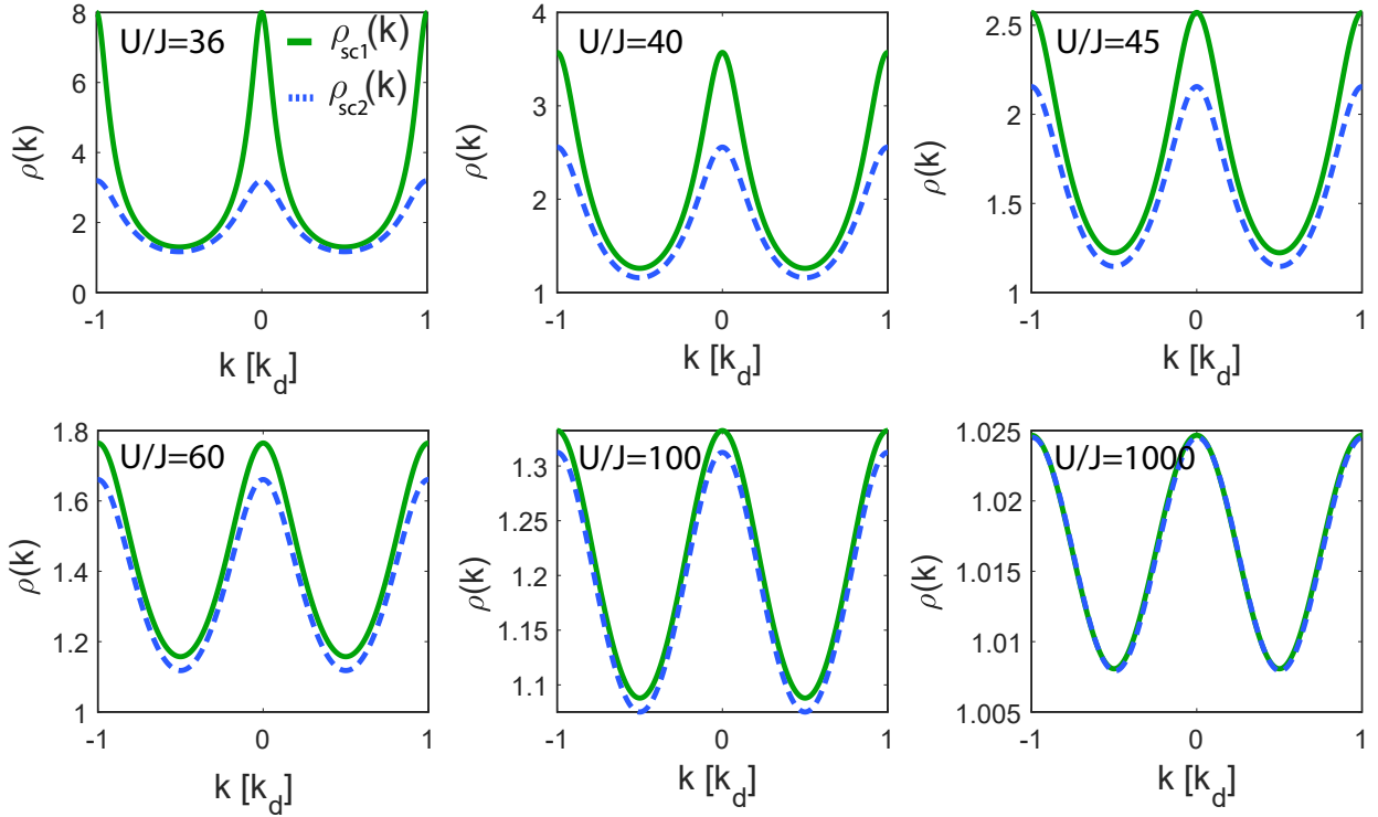
Figure 5.2: Strong coupling momentum distributions. Values of \rho_{sc1}(\vec{k}) (green lines) and \rho_{sc2}(\vec{k}) (blue dashed lines) as a function of k = (k_x, 0, 0) for different values of U/J .
