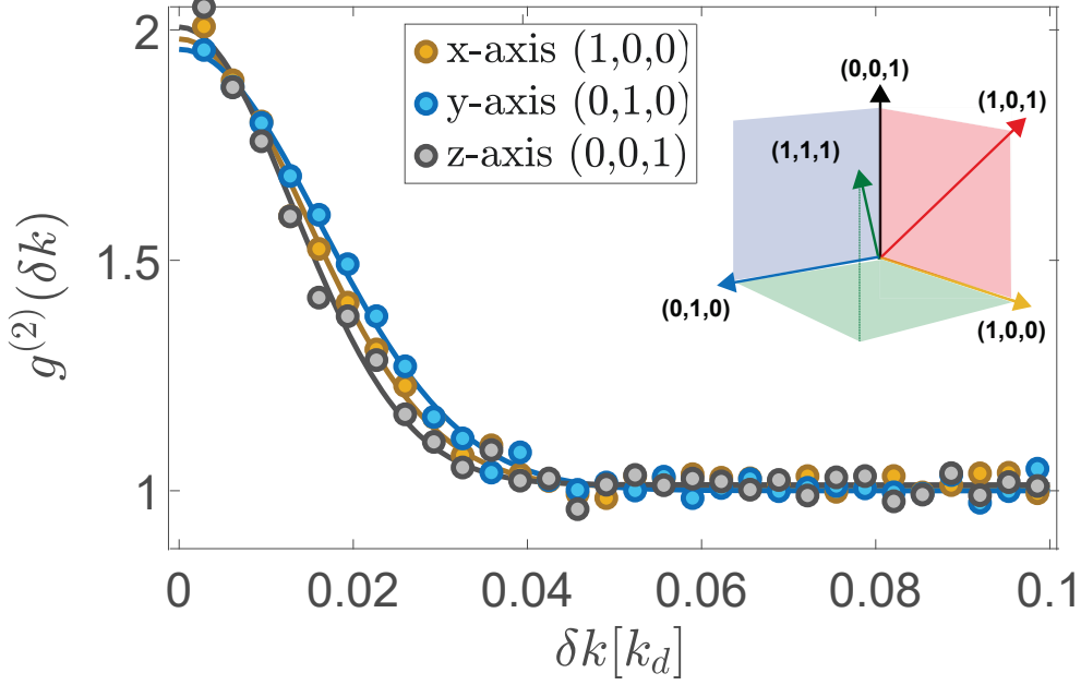
Figure 6.7: Second-order correlation function g^{(2)}(\delta k) of a Mott insulator.
