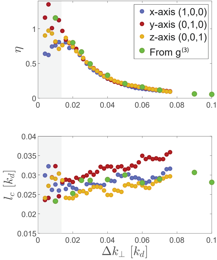
Figure 6.16: Effect of the transverse integration on g^{(3)}(\delta \mathbf{k}_1, \delta \mathbf{k}_2 = 0.5 \mathbf{k}_d) . The profile g^{(3)}(\delta k_1, \delta k_2 = 0.5 k_d) is fitted by the function f(\delta k_1) = c + \eta e^{-2(\delta k_1/l_c)^2} in order to extract the width and the amplitude of the second-order correlation peak as a function of the transverse integration. The results are displayed by the green points. The values of \eta and l_c obtained are similar to the ones found in §.6.1.3 and displayed in Fig. 6.3. These data are also displayed in the graph (yellow, red and blue points).
