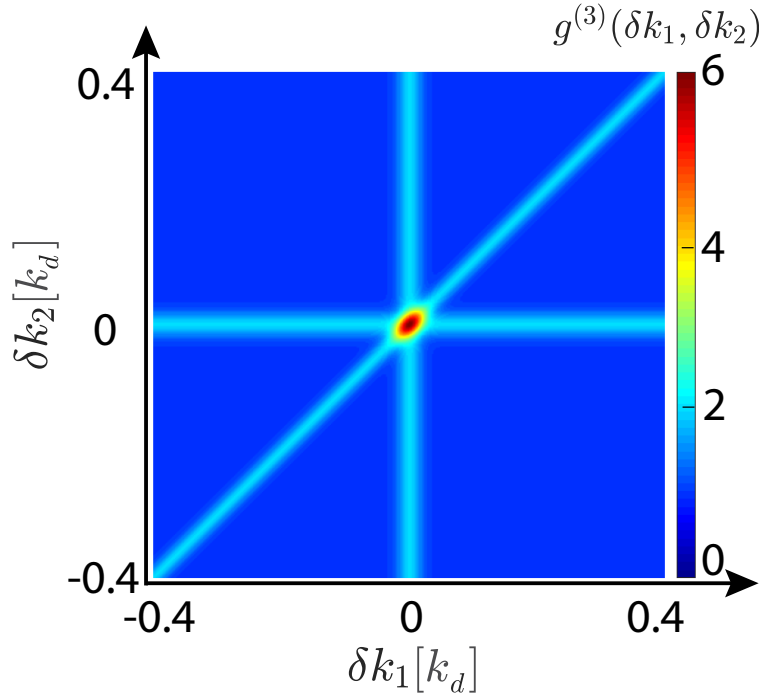
Figure 6.14: Third-order correlation function g^{(3)}(\delta \mathbf{k}_1, \delta \mathbf{k}_2) for a perfect Mott insulator. Plot of the function written in Eq. 6.18 with l_c = 0.028 k_d corresponding to the value of the two-body coherence length measured in §.6.2.3.
