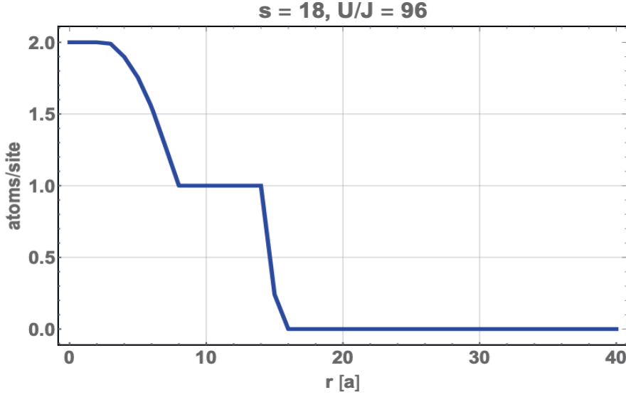
Figure 6.8: In-situ density profile of a Mott insulator at s = 18 and N = 15\,000 atoms calculated with the Guzwiller method. A plateau with a filling n = 2 is present at the center of the cloud. A superfluid, a Mott plateau with n = 1 and an other superfluid region are then present when going to the border of the cloud. The total size of the cloud is about L = 2 \times 16 d \approx 32 d .
