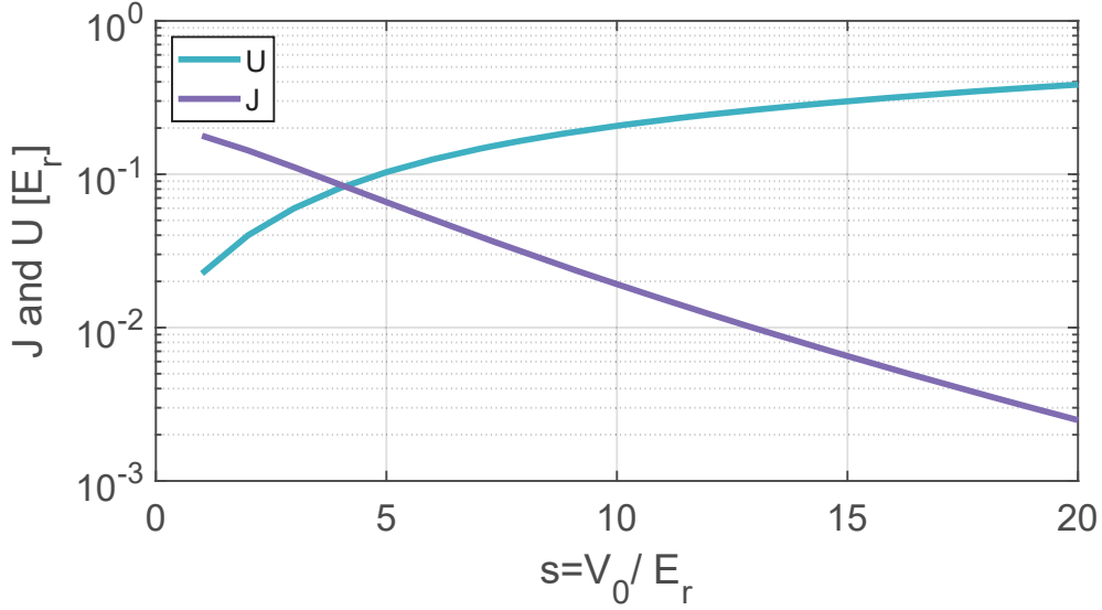
Figure 1.4: Numerical values computed for J and U as a function of the lattice depth V_0 for Helium atoms and d = 775 \text{ nm} (see §.3.1). When the lattice depth increases, J decreases exponentially as it becomes more difficult for the particles to tunnel from one site to another one. Meanwhile, the on-site energy term U increases due to the tightening of the Wannier wavefunctions.
