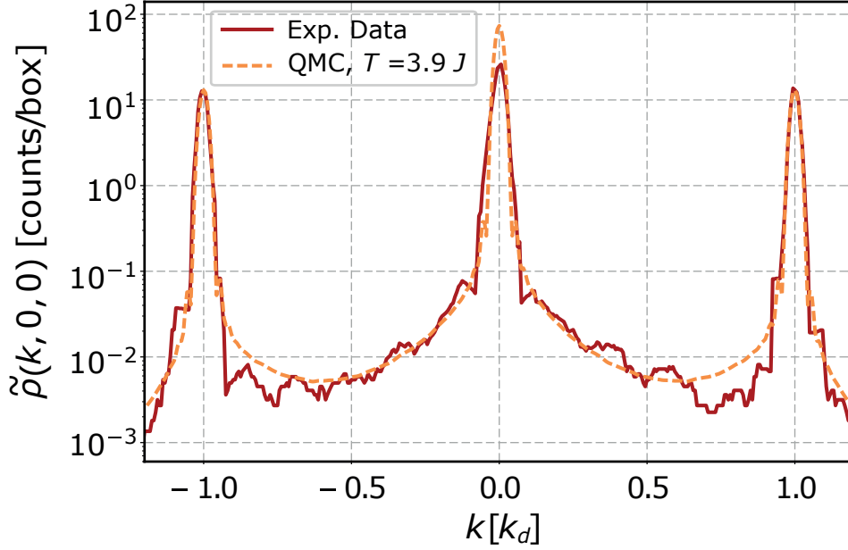
Figure 3.23: Comparison of the measured atom distribution \tilde{\rho} with ab-initio Quantum Monte-Carlo calculation of the in-trap momentum distribution \tilde{\rho}_{\text{QMC}} . Log-plot of 1D high flux cuts through the measured 3D distribution \tilde{\rho} (red), and \tilde{\rho}_{\text{QMC}}(k, 0, 0) through the QMC momentum distribution (dashed orange line) obtained for our experimental parameters and T = 3.9 J . The temperature T is the only adjustable parameter.
