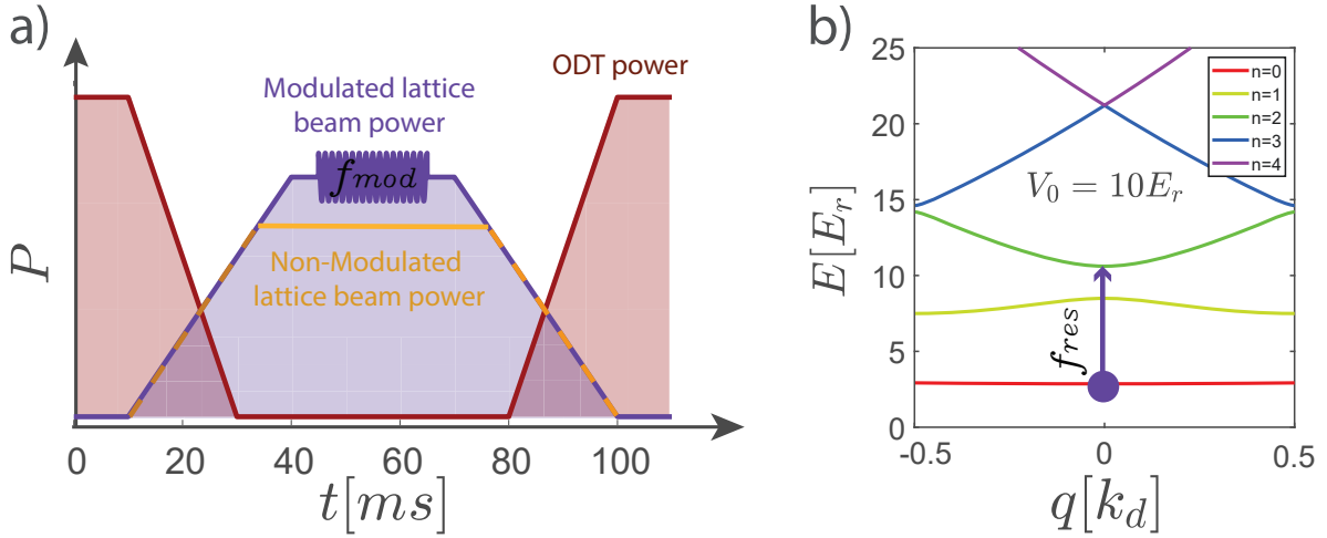
Figure 3.7: Calibration of the optical lattice with the technique of amplitude modulation.
