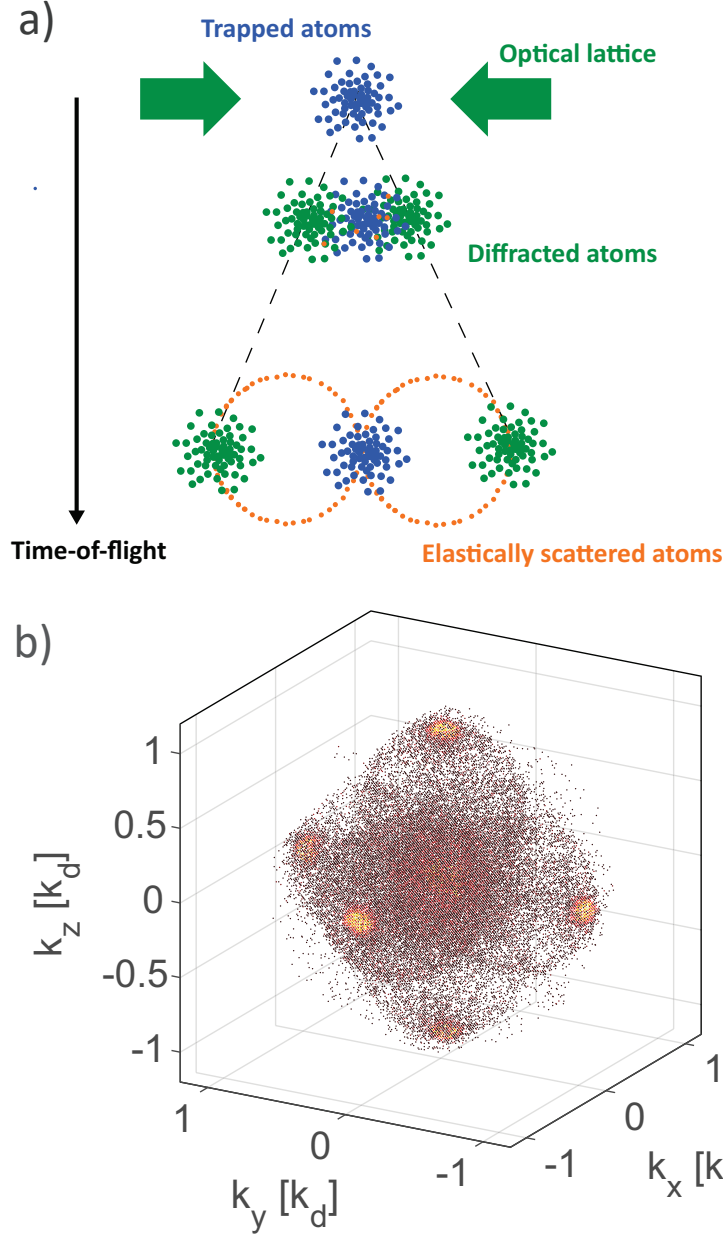
Figure 3.24: 3D collisions happening during the time-of-flight of a lattice gas. a) 1D Sketch of the collision spheres production during the time-of-flight. b) Atomic distribution of a 3D lattice gas with N = 594 (100) \times 10^3 atoms and s = 5 detected using the electronic detection. The momentum distribution has been modified by the collisions happening at the beginning of the time-of-flight. The associated collision spheres are clearly visible in between the central peak and the first-order diffraction peaks.
