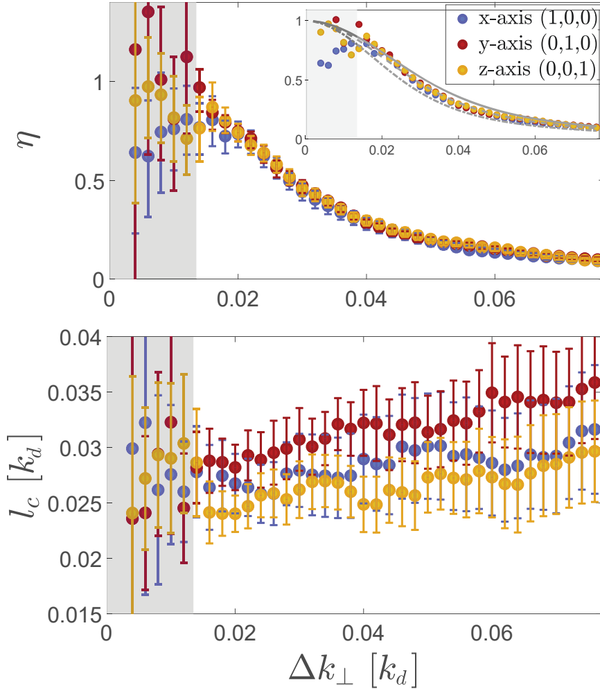
Figure 6.3: Effect of the transverse integration on g^{(2)}(\delta \mathbf{k}) . a) Amplitude of the bunching \eta as a function of \Delta k_\perp . In the inset, are represented the theoretical expectation for \eta(\Delta k_\perp) considering \eta(\Delta k_\perp = 0) = 1 and l_c = 0.028 k_d (grey line), l_c = 0.032 k_d (grey dashed line) and l_c = 0.035 k_d (grey dotted-dashed line). b) Correlation length l_c as a function of \Delta k_\perp . Grey areas on both graphs correspond to the region where the signal is too noisy to provide quantitative information.
