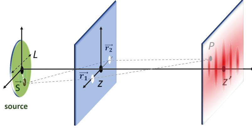
Figure 2.1: Measurement of the first-order coherence using a double-slit experiment.
