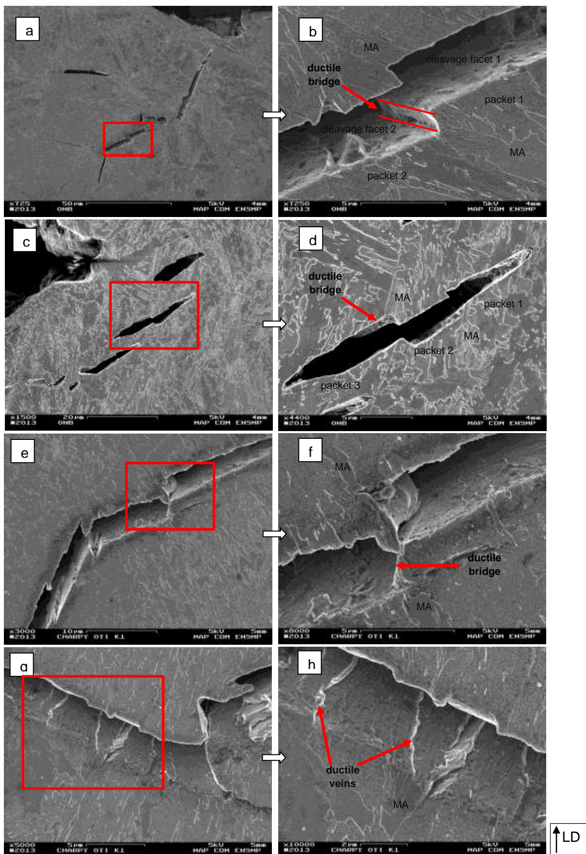
Figure 81: SEM, Nital2%, cross-section, from the middle of impact specimen, SE in-lens. Interactions between secondary microstructural constituents and secondary cleavage cracks. (a) to (d) 0Nb 35 (specimen 3, 23.1J), (e) to (h) 0Ti 35 (specimen 1, 60.3J).
