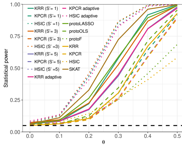
Figure 3.3: Statistical power of kernelPSI variants and benchmark methods, using Gaussian kernels for simulated Gaussian data.
