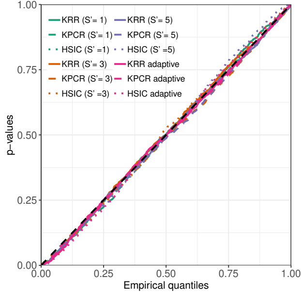
Figure 3.1: Q-Q plot comparing the empirical kernelPSI p-values distributions under the null hypothesis ( \theta = 0.0 ) to the uniform distribution.
