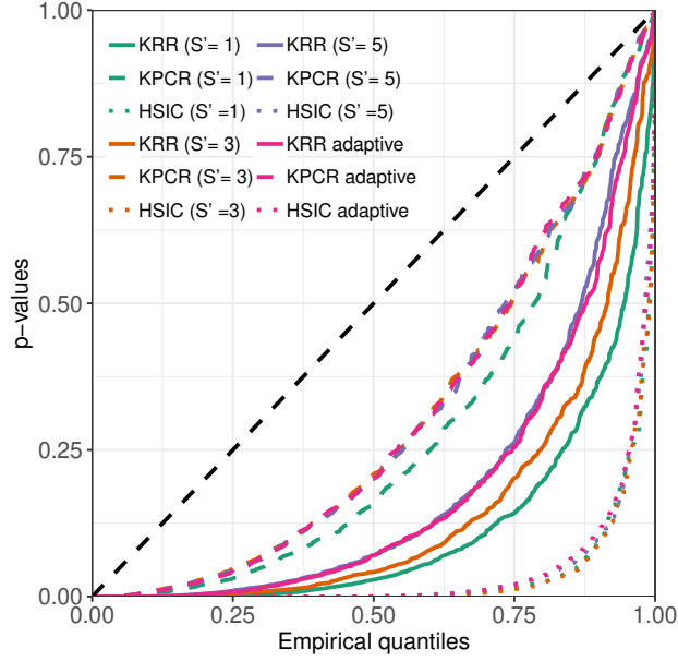
Figure 3.2: Q-Q plot comparing the empirical kernelPSI p-values distributions under the alternative hypothesis ( \theta = 0.3 ) to the uniform distribution.
