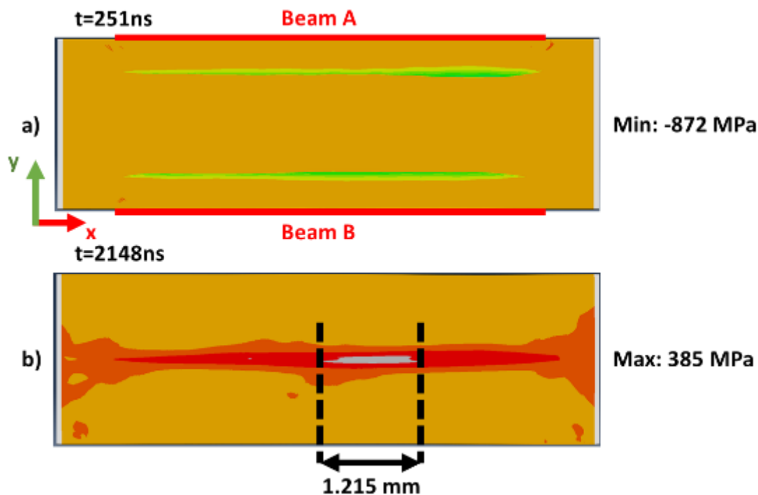
Figure 3-15 Shockwaves propagation using the real spatial experimental loading a) at t=251\text{ns} b) at t=2148\text{ns}
