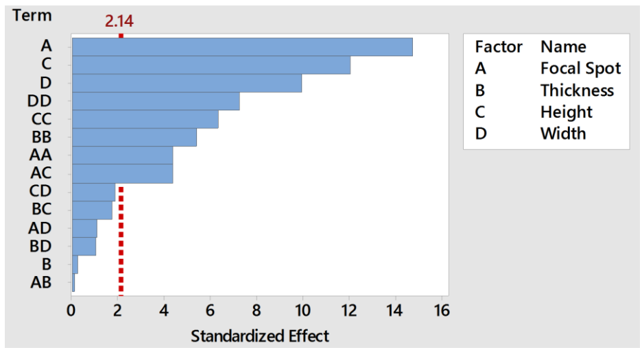
Figure 3-19 Model's Pareto chart (P = 0.05)
