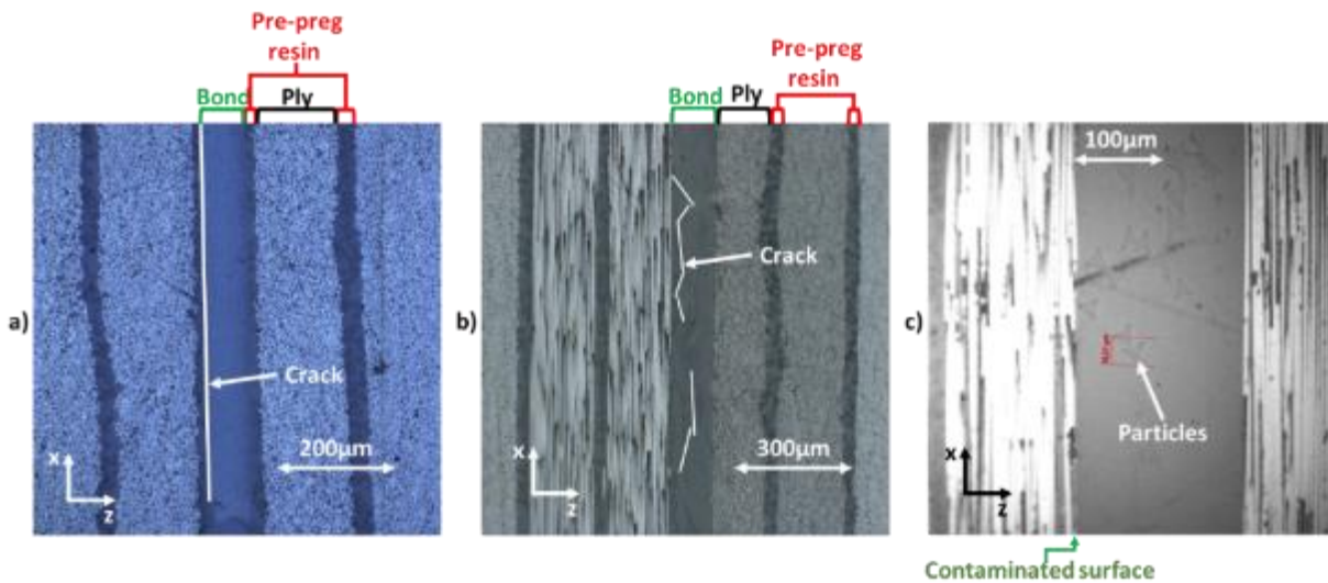
Figure 4-6 Photomicrographs of the bond after damage created by S-LASAT: a) production reference sample. b) repair reference sample. c) highest degree of de-icing fluid contamination
