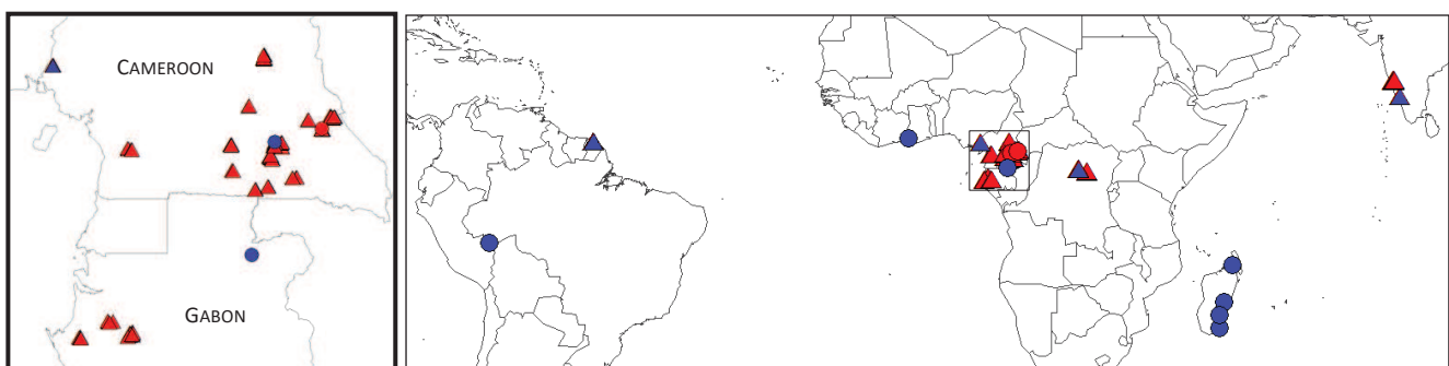
Figure 1-3. Distribution of datasets across the tropics. Dots and triangles represent tree-level destructive datasets and field plot inventories, respectively. Red color indicates that data have been collected by IRD. Blue color indicates that data were compiled from literature, collaborating institutions or shared by the peer researchers.
