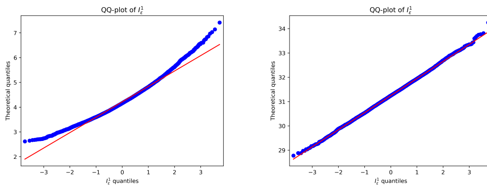
Figure 2.11: [Test case 1] QQ-plot for the distribution of I_\epsilon (left: \epsilon = 1/10 ; right: \epsilon = 1/70 ) computed from \mathcal{M} = 10^4 realizations.
