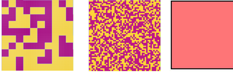
Figure 1.4: Example of a random stationary material: random checkerboard for different values of \varepsilon ( \varepsilon = 1/10 , \varepsilon = 1/50 , \varepsilon \ll 1 , from left to right).
