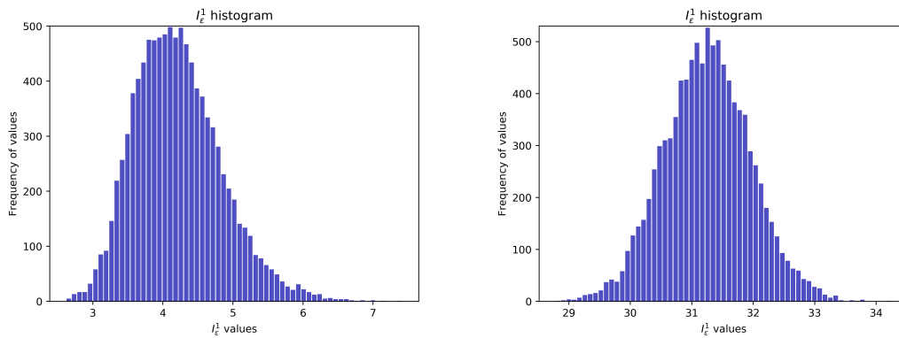
Figure 2.10: [Test case 1] Empirical distribution of I_\epsilon (left: \epsilon = 1/10 ; right: \epsilon = 1/70 ) computed from \mathcal{M} = 10^4 realizations.
