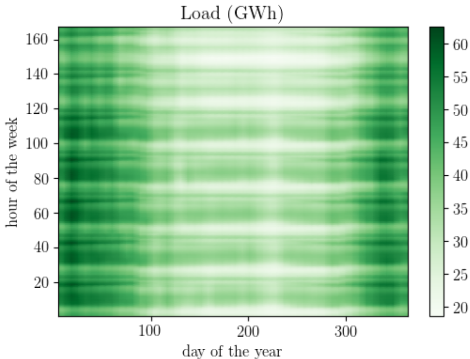
FIGURE 2.14: Load conditioned on hours and days of the year Expectation of the nationally aggregated load conditioned on the hour of the week and the day of the year. Note that the shift during the year of the peaks in the morning and in the evening described with Figure 2.9 are also visible in this illustration. They are particularly visible but not limited to the transition to Daylight Saving Time around days 90 and 300.
