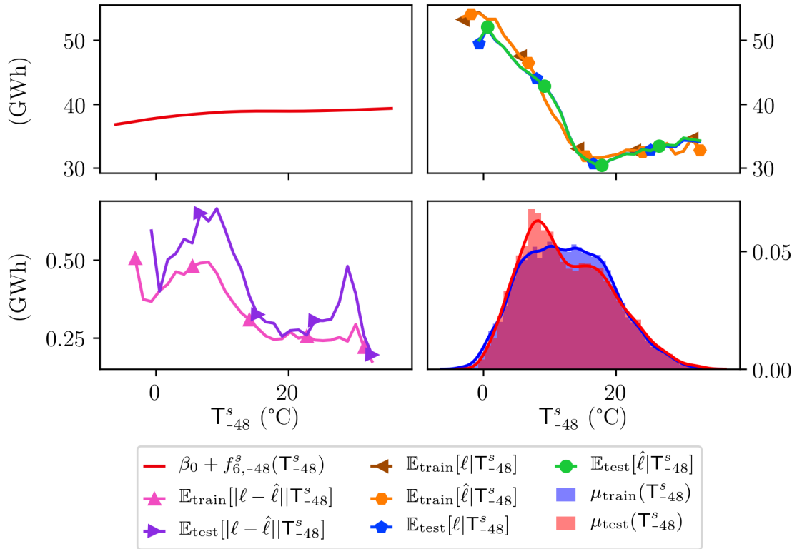
FIGURE F.23: Estimated effect of the 48 h-delayed temperature
