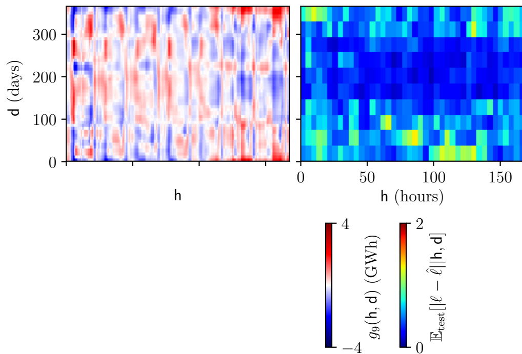
FIGURE F.34: Interaction between hours and days of the year ( left ) Interaction g_9(\mathbf{h}, \mathbf{d}) between the hour of the week \mathbf{h} and the day of the year \mathbf{d} in the short-term national model. ( right ) Average residuals in the test set \mathbb{E}_{\text{test}}[|y - \hat{y}| | \mathbf{h}, \mathbf{d}] .
