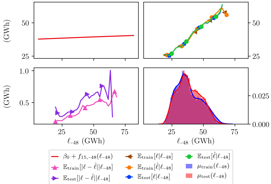
FIGURE F.28: Estimated effect of the 48 h-delayed load ( top left ) Effect \beta_0 + f_{15,-48}(\ell_{-48}) learned by the national short-term model for the 48 hours-delayed load. ( bottom left ) Norm of the conditional residuals \mathbb{E}_{\text{train}}[|\ell - \hat{\ell}||\ell_{-48}] and \mathbb{E}_{\text{test}}[|\ell - \hat{\ell}||\ell_{-48}] . ( top right ) Conditional loads \mathbb{E}_{\text{train}}[\ell|\ell_{-48}] and \mathbb{E}_{\text{test}}[\ell|\ell_{-48}] with the conditional forecasts \mathbb{E}_{\text{train}}[\hat{\ell}|\ell_{-48}] and \mathbb{E}_{\text{test}}[\hat{\ell}|\ell_{-48}] . ( bottom left ) Density of the data in the training and the test sets.
