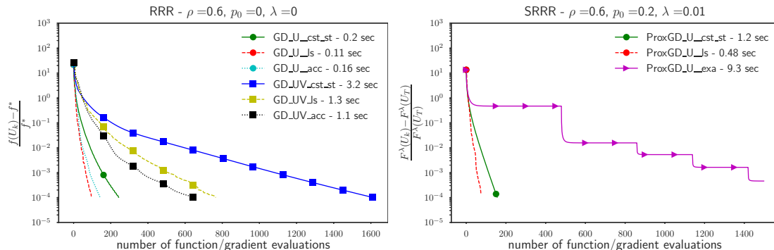
FIGURE 5.3: (Left) RRR : Convergence of f(U_k) - f^* for gradient descent on our formulation in U with constant step size (GD_U_cst_st), with line search (GD_U_ls), with the acceleration (GD_U_acc) proposed by Li and Lin [2015] and gradient descent for the formulation of [Park et al., 2016] with constant step size, line search and acceleration (GD_UV_cst_st, GD_UV_ls, GD_UV_acc). (Right) SRRR with \lambda = 0.01 : Convergence for T large of F^\lambda(U_k) - F^\lambda(U_T) for proximal gradient descent on our formulation with and without line search (ProxGD_U_ls, ProxGD_U_cst_st), compared with the alternating optimization algorithm (ProxGD_U_exa) proposed in Bunea et al. [2012]. The running time to reach a precision of 10^{-4} is given at the top right.
