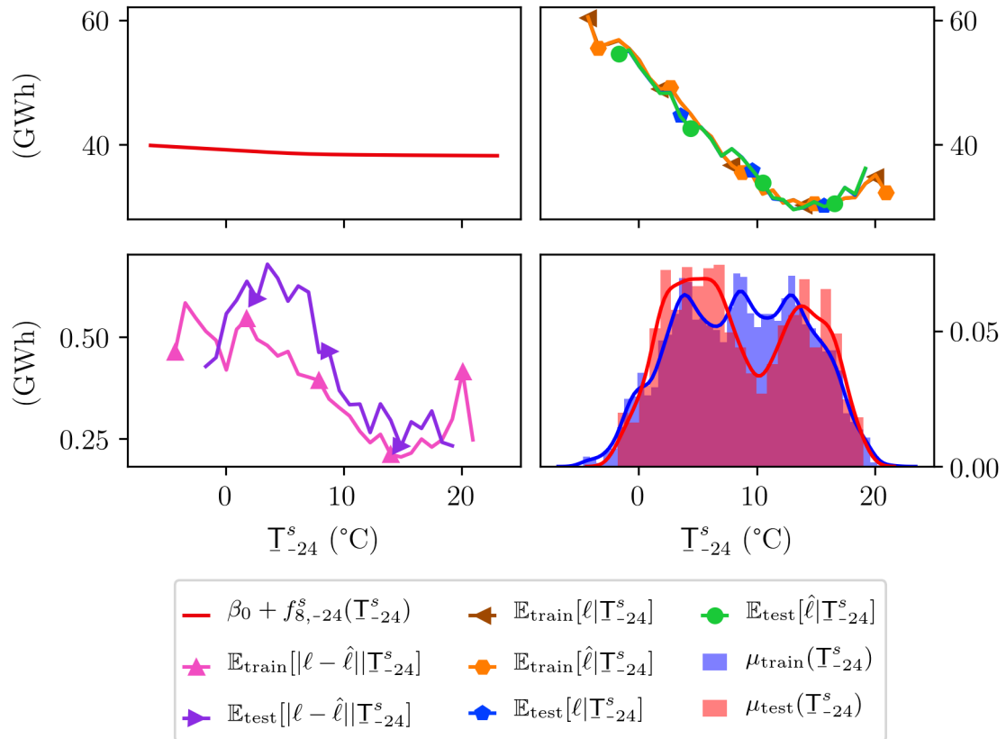
FIGURE F.26: Estimated effect of the 24 h min temperature ( top left ) Effect \beta_0 + f_{8,-24}^s(\Gamma_{-24}^s) learned by the national short-term model for the minimum over 24 hours of the weighted temperature defined with Table F.1. ( bottom left ) Norm of the conditional residuals \mathbb{E}_{\text{train}}[|\ell - \hat{\ell}| | \Gamma_{-24}^s] and \mathbb{E}_{\text{test}}[|\ell - \hat{\ell}| | \Gamma_{-24}^s] . ( top right ) Conditional loads \mathbb{E}_{\text{train}}[\ell | \Gamma_{-24}^s] and \mathbb{E}_{\text{test}}[\ell | \Gamma_{-24}^s] with the conditional forecasts \mathbb{E}_{\text{train}}[\hat{\ell} | \Gamma_{-24}^s] and \mathbb{E}_{\text{test}}[\hat{\ell} | \Gamma_{-24}^s] . ( bottom left ) Density of the data in the training and the test sets.
