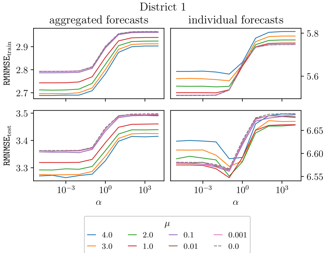
FIGURE 4.7: Success with the sum consistent loss in District 1 ( top left ) RMNRMSE on the training set of the forecasts aggregated in District 1. It measures the error \left\| \frac{1}{\eta_1} \sum_{k \in Z_1} (y_k - \hat{y}_k) \right\|_2^2 . ( bottom left ) RMNRMSE on the test set of the forecasts aggregated in District 1. ( top right ) RMNRMSE on the training set of the individual forecasts in District 1. It measures the error \frac{1}{\eta_7} \sum_{k \in Z_1} (y_k - \hat{y}_k)^2 . ( bottom right ) RMNRMSE on the test set of the individual forecasts in District 1.
