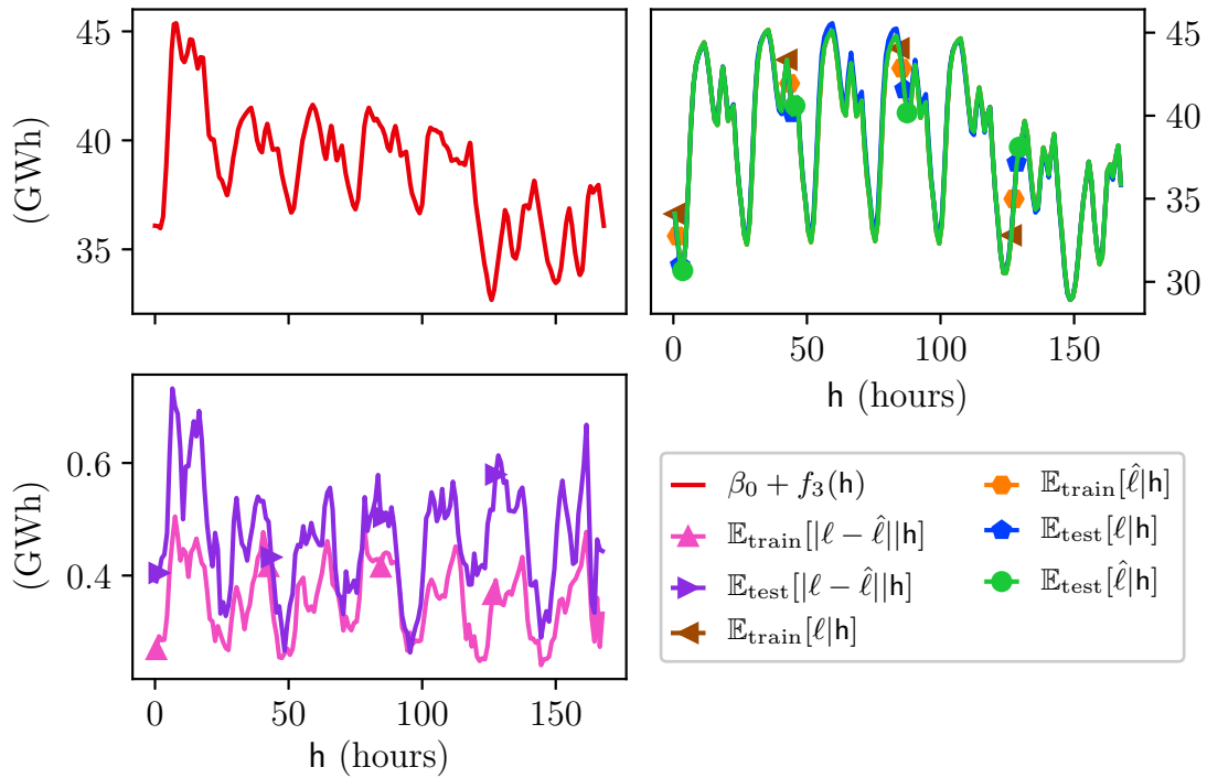
FIGURE 3.7: Estimated effect of the hour of the week
