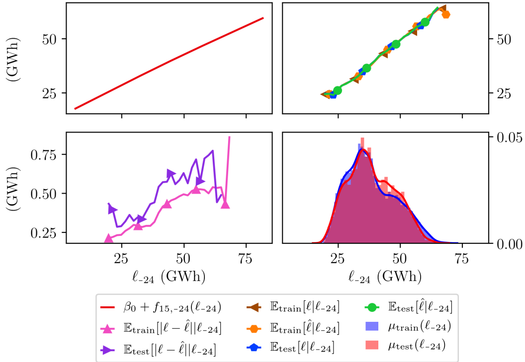
FIGURE 3.11: Estimated effect of 24 h-delayed load ( top left ) Effect \beta_0 + f_{15,-24}(l_{-24}) learned by the national short-term model for the 24 hours-delayed loads after renormalization. ( bottom left ) Conditional norm of the residuals \mathbb{E}_{\text{train}}[|l - \hat{l}||l_{-24}] and \mathbb{E}_{\text{test}}[|l - \hat{l}||l_{-24}] . ( top right ) Conditional loads \mathbb{E}_{\text{train}}[l|l_{-24}] and \mathbb{E}_{\text{test}}[l|l_{-24}] with the conditional forecasts \mathbb{E}_{\text{train}}[\hat{l}|l_{-24}] and \mathbb{E}_{\text{test}}[\hat{l}|l_{-24}] . ( bottom right ) Density of the loads in the training and the test sets.
