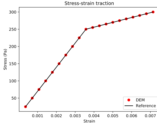
Figure 3.6 – Beam in quasi-static traction: stress-strain response curve for the analytical solution and the DEM solution.
