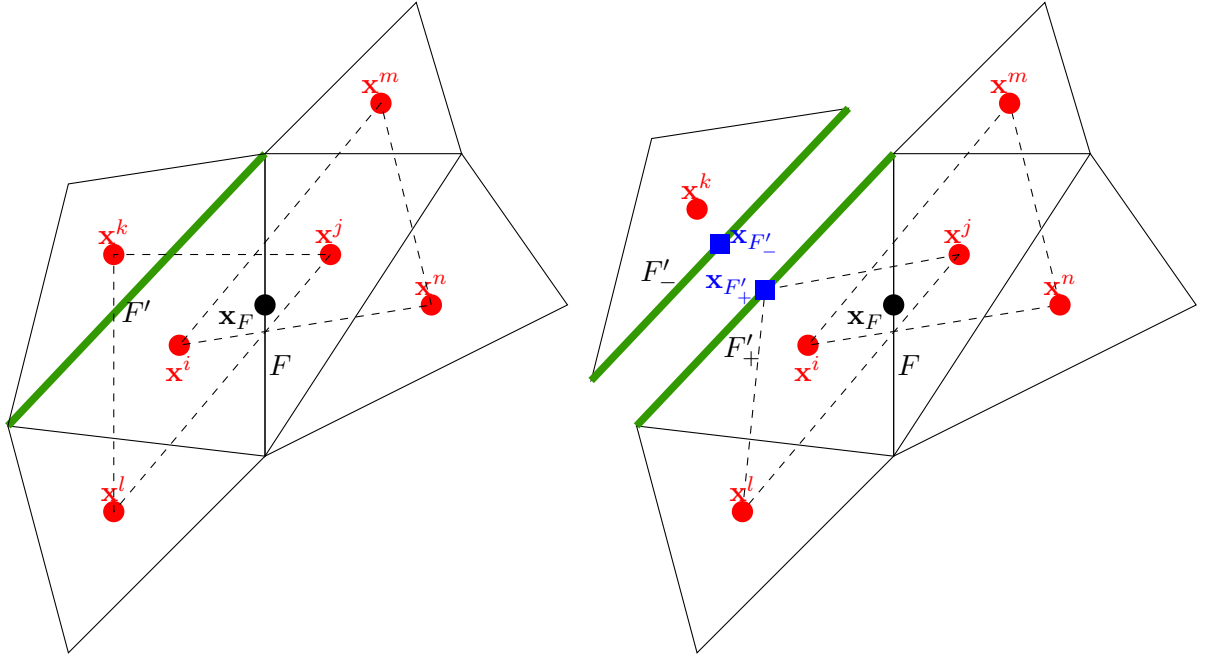
Figure 4.10 – Re-computation of the reconstruction stencil associated with the inner facet F after the breaking of the neighbouring inner facet F' . Left: reconstruction before cracking. Right: reconstruction after cracking. (The two cells separated by the crack are drawn slightly apart.)
