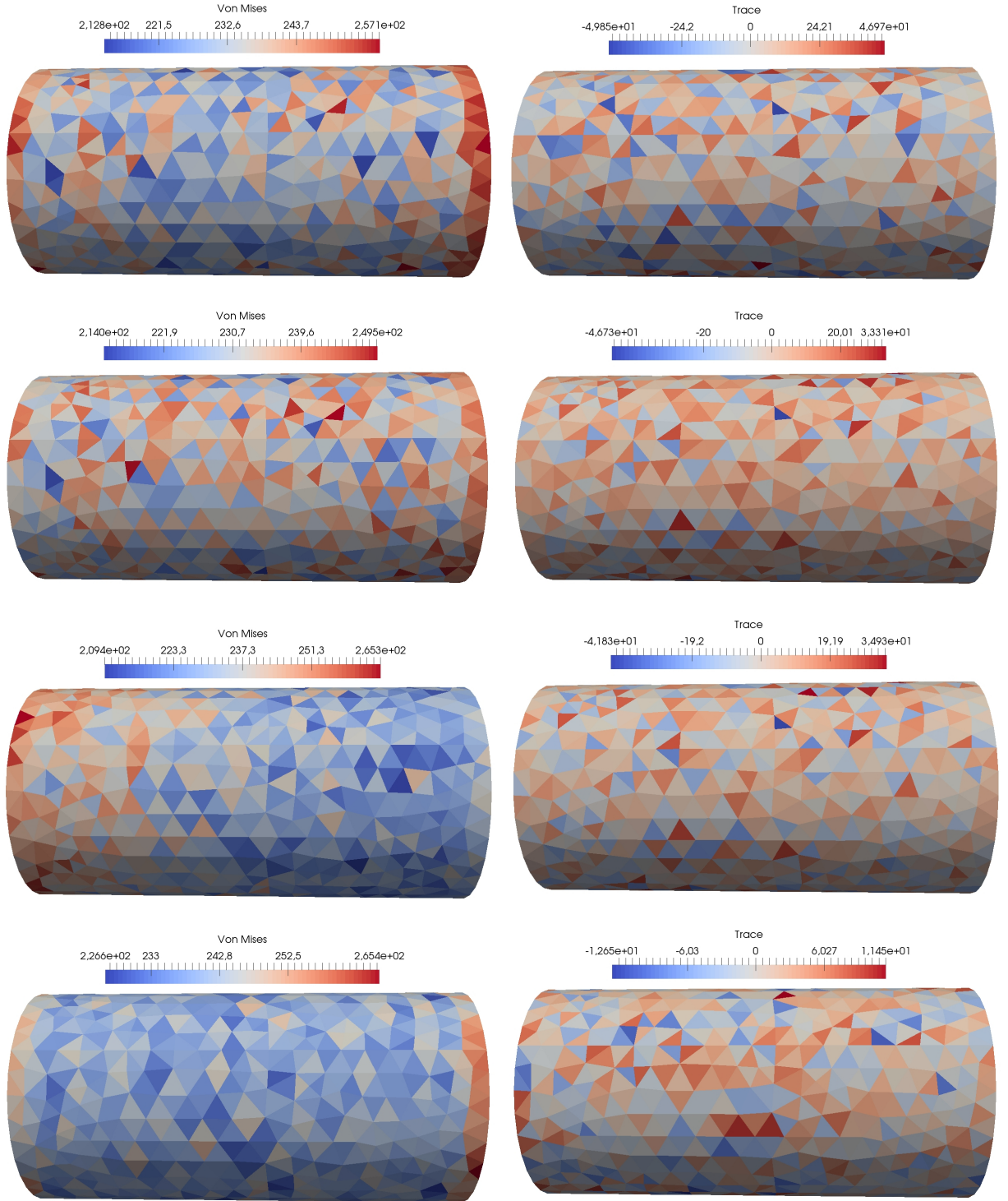
Figure 3.4 – Choice of penalty factor: Left: Von Mises equivalent stress. Right: Trace of the stress tensor. First row: DEM with \beta = 1 . Second row: DEM with \beta = 0.1 . Third row: DEM with \beta = 0.01 . Fourth row: Penalised Crouzeix–Raviart FE with \beta = 1 (reference).
