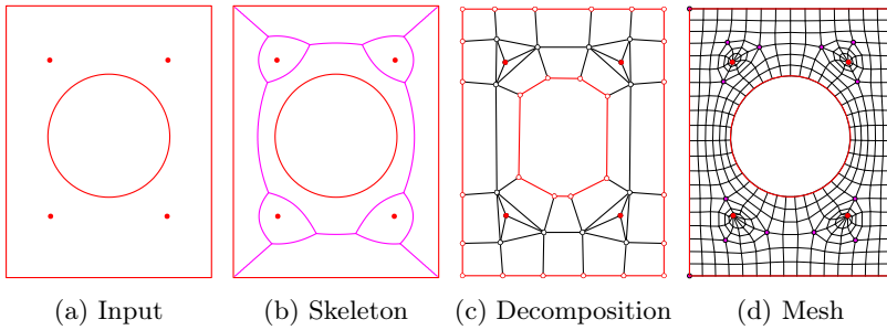
Figure 4.13 – Skeleton-based decomposition of a surface in a coarse quad mesh to yield a pattern aligned with the boundary and point features of the boundary.
