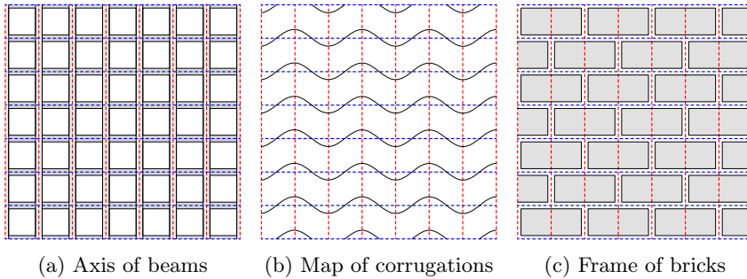
Figure 1.9 – Quad meshes in dashed red and blue lines representing different structural systems in black and grey.
