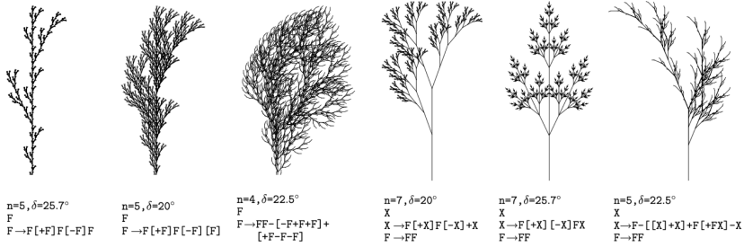
Figure 2.3 – L-systems are a specific type of formal grammars interpreted by turtle graphics designed for algorithmic generation of plants [Prusinkiewicz and Lindenmayer, 2012]. Here, the designs stem from a different number of iterations n , a different branching angle \delta , a starting string axiom and one or several rule to iteratively apply.
