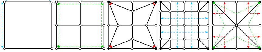
(b) Temporarily adding the strips in cyan to add the the strips in green and red to obtain a quad-mesh topology with a pole at each corner, to provide many load paths to the supports.
