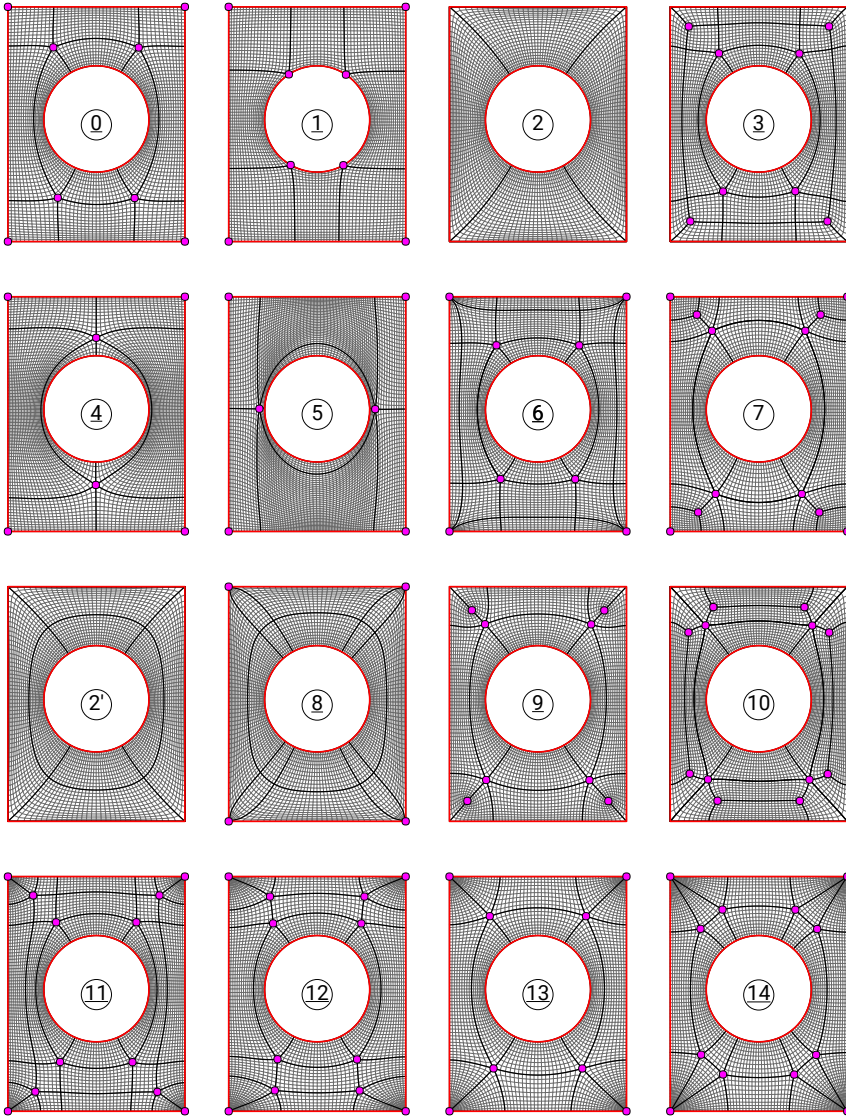
Figure 5.26 – Resulting quad-mesh patterns with different topologies. The labels of the Pareto designs are underlined.
