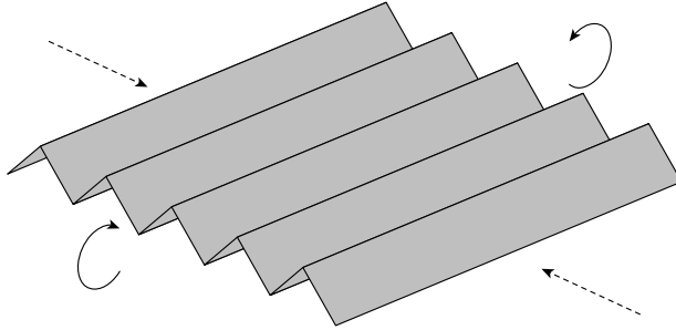
Figure 7.32 – Folded patterns increase the bending stiffness along the folds and decrease the membrane stiffness across the folds.
