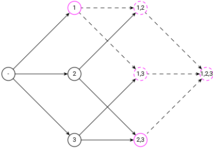
Figure 7.24 – Principle of the search algorithm for two-coloured quad meshes. The search yields only the closest two-coloured quad meshes in independent design directions. The two-coloured quad meshes are highlighted in pink, and the discarded quad meshes downstream are marked by dashes.
