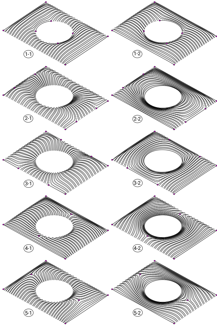
Figure 7.37 – The ten folded shells resulting from the five pattern topologies times the two folded directions, marked as X and Y in the X-Y labels, respectively.
