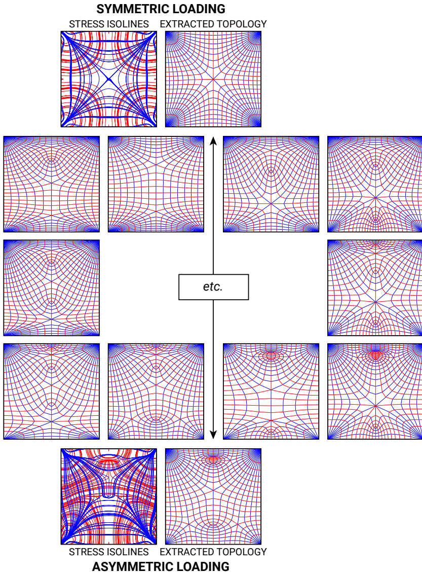
Figure 6.30 – Similarity-informed topology finding based on structural performance against multiple load cases. Obtaining a performance trade-off is sensitive to parameters of geometrical processing and may require geometrical optimisation.
