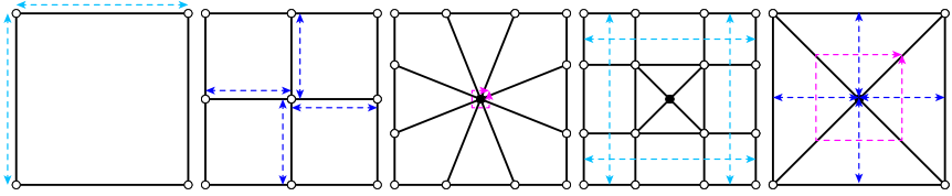
(a) Temporarily adding the strips in cyan to add the the strips in blue and pink to obtain a quad-mesh topology with a pole at the centre, to provide many load paths to the point load.
