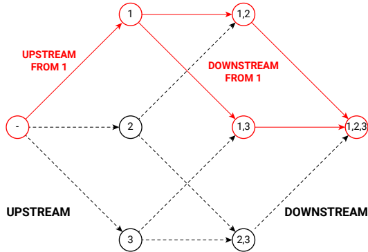
Figure 7.20 – This graph represents the search organisation through the combinations of three deletion rules 1, 2 and 3. The search algorithm applies only deletion rules, defining an orientation the upstream combination (-) to the downstream combination (1,2,3). For instance, (1,2) is in the downstream direction of (1) but (2,3) is not in the direction of (1).
