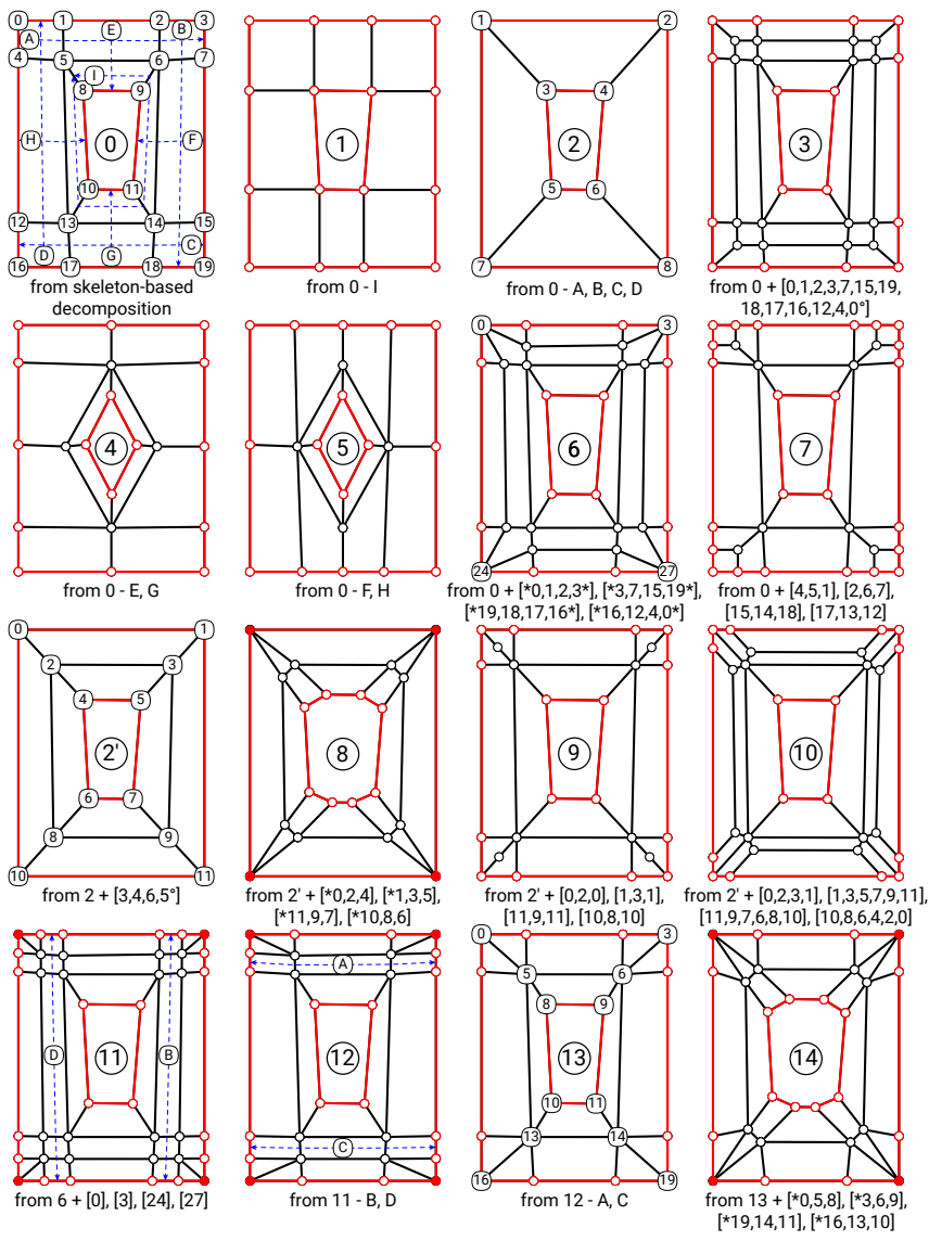
Figure 5.25 – Rule-based exploration of coarse quad meshes.
