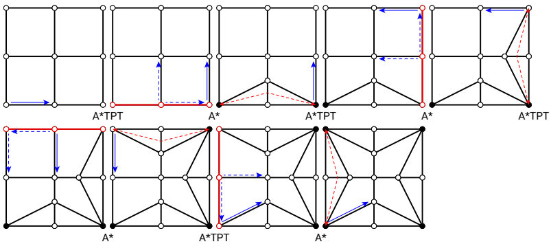
Figure 8.14 – The string A^* T P T A^* A^* T P T A^* A^* T P T A^* A^* T P T A^* adds four strips with poles along the boundary.
