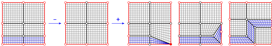
Figure 8.1 – The quad-mesh grammar allows deleting and adding the strips in blue. However, the grammar can not modify a strip, despite the similarity between the old and new strips.
