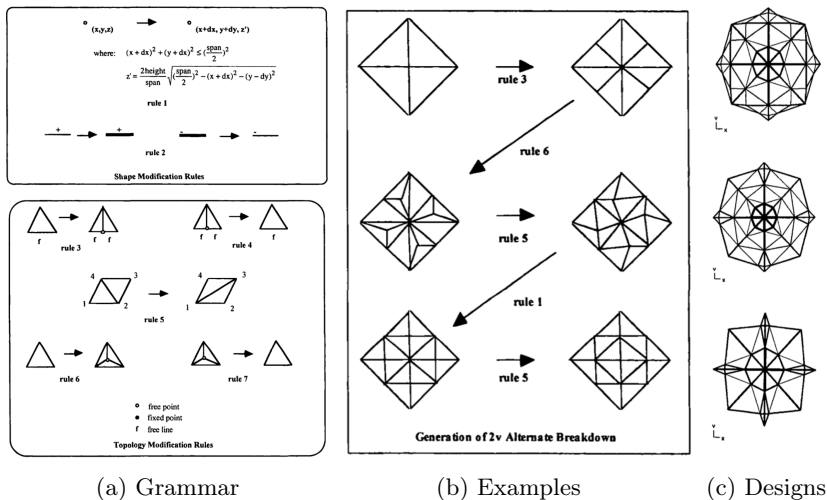
Figure 2.4 – Grammar for rule-based design of triangulated meshes for geodesic domes [Shea and Cagan, 1997].
