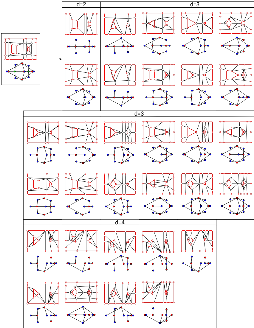
Figure 7.31 – Two-colour projection applied to a 14-strip quad mesh with a rectangular shape with two openings.
