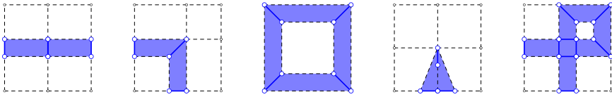
Figure 5.17 – Disconnected graphs of vertices to merge for the strip deletion rule.
