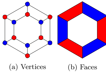
Figure 7.10 – The vertex and face elements along a closed strip can be two-coloured if crossed by an even number of elements.
