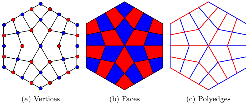
Figure 7.4 – The three types of two-colourability for quad-mesh patterns.
