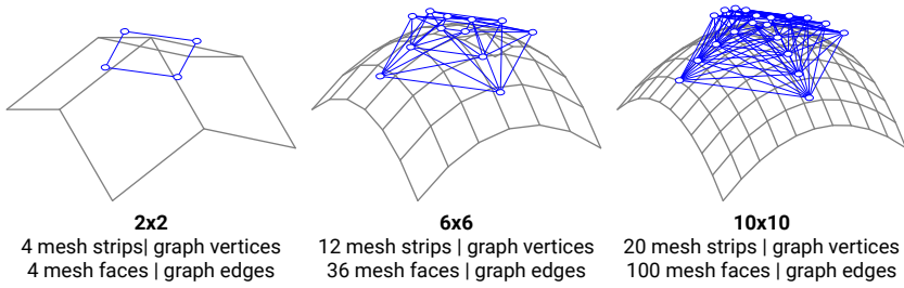
Figure 5.7 – The number of elements in the strip graph increases with the density of the quad mesh. An N \times N grid mesh has 2N strips and N^2 faces, and its strip graph has 2N vertices and N^2 edges.
