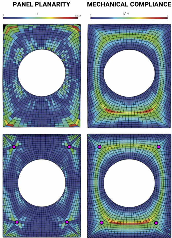
Figure 2.2 – Two pattern designs revisiting the British Museum roof. The topology at the top performs the best regarding the requirement on the right on minimising mechanical compliance. The topology at the bottom performs the best regarding the requirement on the left on minimising panel planarity [Schiftner and Balzer, 2010]. The singularities in a quad mesh, highlighted in pink, influence its efficiency and affordability, highlighting the importance of their design for the challenge of meeting trade-offs in multi-objective structural design.
