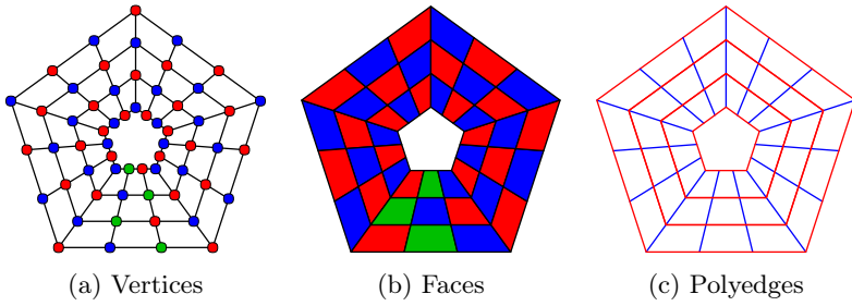
Figure 7.6 – Quad mesh with two-coloured polyedges but without two-coloured vertices or faces due to the odd number of elements along the closed strips.
