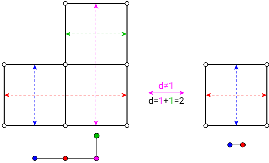
Figure 6.9 – Collateral strip deletion occurs when deleting one or several strips, like the one in pink, results in the deletion of other strips, like the one in green. Applying such a deletion rule counts as multiple deletions rules, two in this case.
