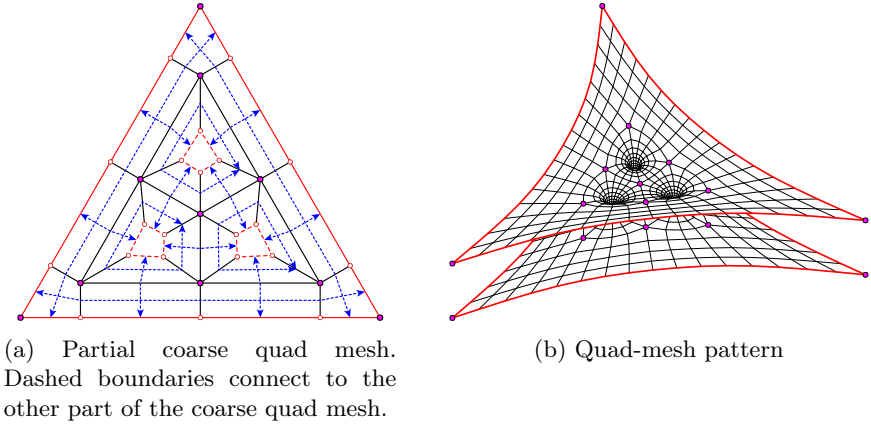
Figure 5.20 – Example of the strip structure in a quad-mesh pattern with a non-null genus.
