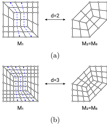
Figure 6.13 – Limitation examples for computing the topological distance between two dense quad meshes. The distances between the meshes M_1 and M_2 and between their submesh M_0 is provided along with one of the possible combination of strips to delete in blue.
