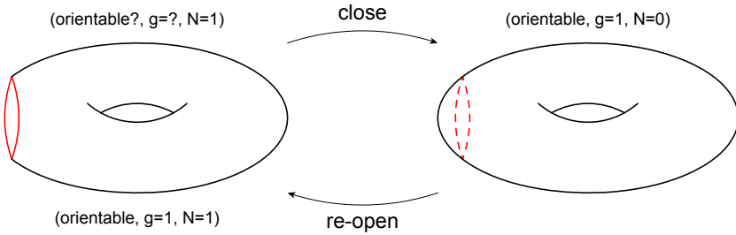
Figure 2.14 – Characterisation of an open compact manifold shape via the equivalent closed shape by temporarily zipping a topological disc along each boundary.
