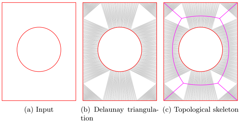
Figure 4.3 – Generation of the topological skeleton of a surface by connecting the circumcentres of adjacent faces of a Delaunay triangulation.
