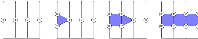
Figure 5.9 – Detailed addition of a strip along a polyedge.
