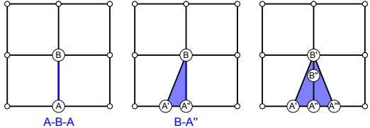
Figure 5.14 – Add a self-crossing strip with update of the polyedge.
