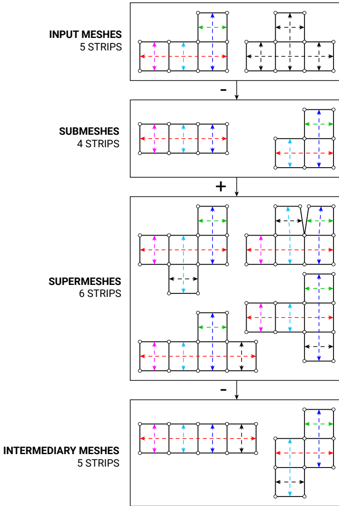
Figure 6.16 – Deleting the dissimilar strips between input meshes yields the submeshes. Adding the dissimilar strips on the submeshes yields the supermeshes. Deleting combinations of dissimilar strips yields the intermediary meshes. The strip structure of one of the input meshes is coloured in all hybrid meshes to highlight the similarity with this input mesh.
