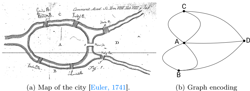
Figure 2.8 – The problem of the seven bridges of the city of Königsberg, encoded by Leonhard Euler in a graph, where each vertex represents a district and each edge represents a bridge between two districts.
