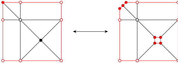
Figure 5.2 – Interpreting a pseudo-quad mesh as a quad mesh with poles as virtual boundary edges.
