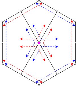
Figure 7.12 – The even numbers of strips around the non-boundary vertex in pink and along the boundary guarantee the fulfilment of the singularity requirement for two-colouring.
