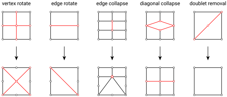
Figure 2.5 – A grammar rules for quad mesh visual-quality optimisation [Tarini et al., 2010].
