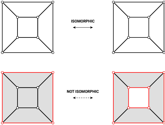
Figure 6.3 – Two quad meshes are isomorphic if their graph of edges are isomorphic while preserving edge boundary attribute marked in red. The corresponding mesh faces are marked in grey for clarity.
