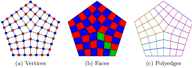
Figure 7.7 – Quad mesh with two-coloured vertices but without two-coloured faces or polyedges due to the odd number of elements around the singularity.
