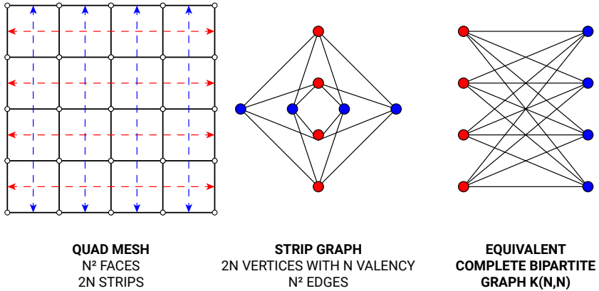
Figure 7.15 – A N \times N quad-mesh grid has a strip graph equivalent to a complete bipartite graph K(N, N) , with 2N vertices connected to N vertices, resulting in a quadratic time complexity O(n^2) for the two-colouring algorithm.
