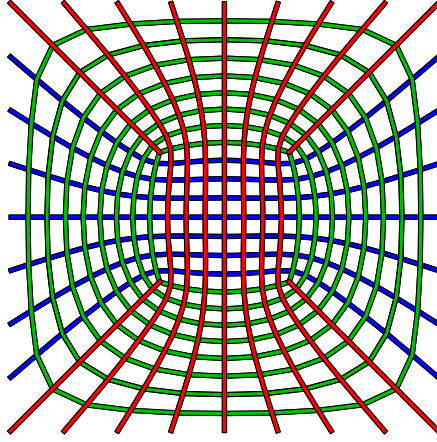
Figure 7.2 – A quad-mesh pattern with a three-valent singularity is an example of a topology that can not be two-coloured, in red and blue. A third group of elements, in green, is necessary to avoid having elements of the same group overlapping each other. This topology is not suitable for the design of an elastic gridshell made of continuous beams organised in two layers without having beams weaving between the two layers.
