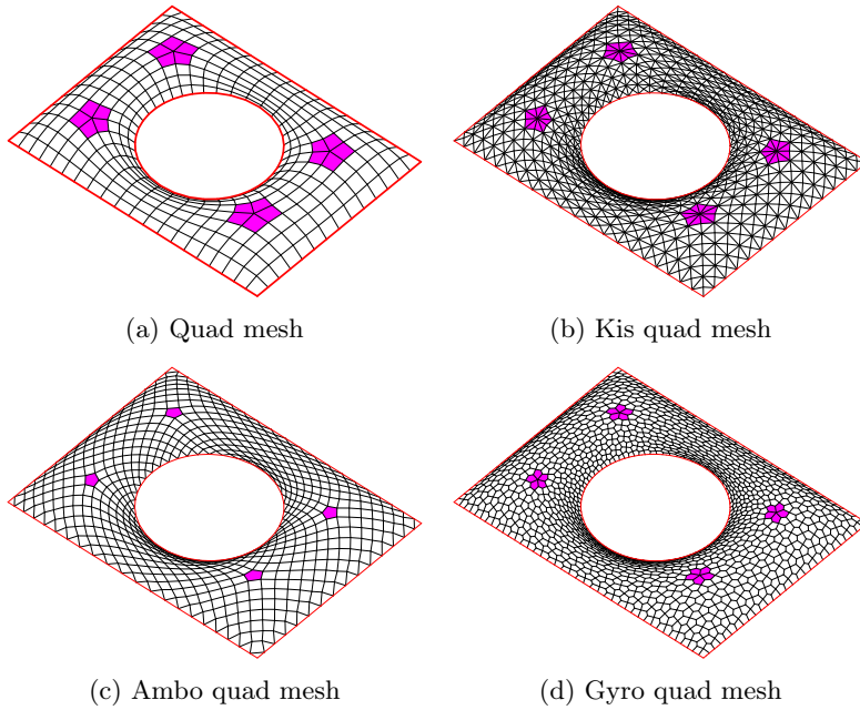
Figure 2.6 – Applying Conway operators on a seed quad mesh generates patterns with different tessellations but equivalent vertex or face singularities in pink.
