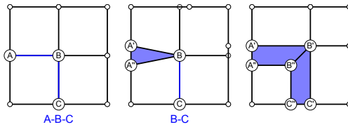
Figure 5.11 – Add a strip changing the singularities.
