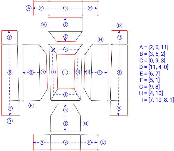
Figure 5.4 – Exploded map of the strips with their face data.
