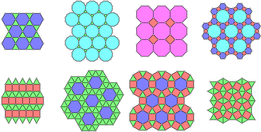
Figure 1.6 – The eight semi-regular tessellations of the plane. The colours represent the polygons with the same number of edges.
