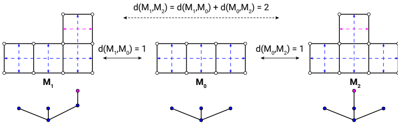
Figure 6.10 – Finding the distance between two quad meshes M_1 and M_2 via a common submesh M_0 using strip deletion rules only. The deleted strips are highlighted in pink.
