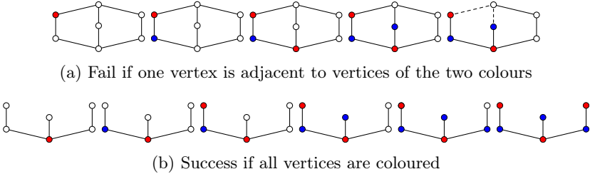
Figure 7.14 – Iterative two-colouring of the vertices of a graph.
