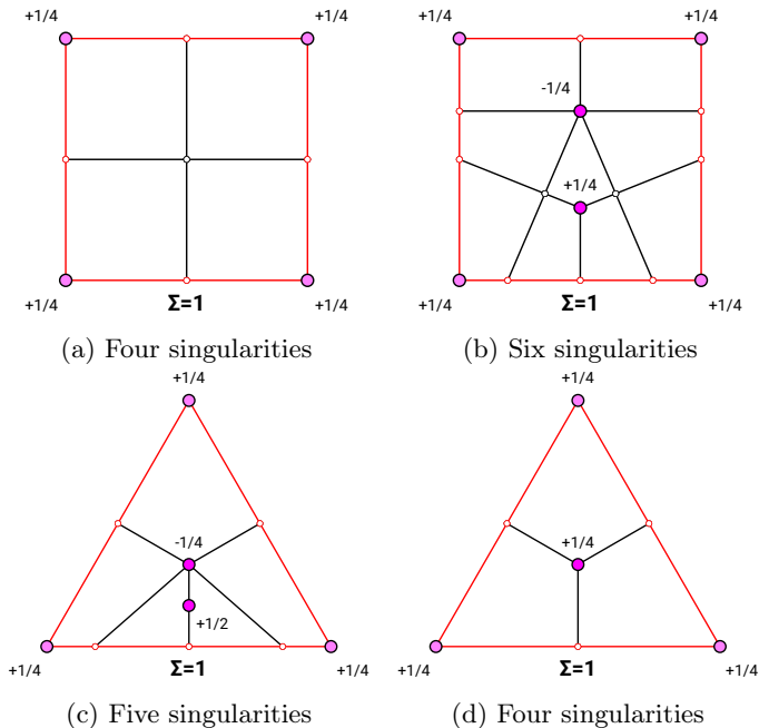
Figure 2.20 – For a given shape topology, the combination of singularities must respect the PHT. The circle-homotopic shapes have an Euler characteristic of one, therefore the sum of the vertex indices equals one.
