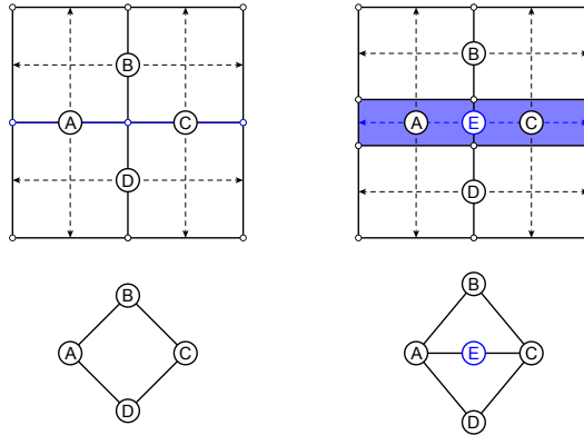
Figure 5.19 – Corresponding strip graph operations due to the addition and deletion of the quad-mesh strip E .
