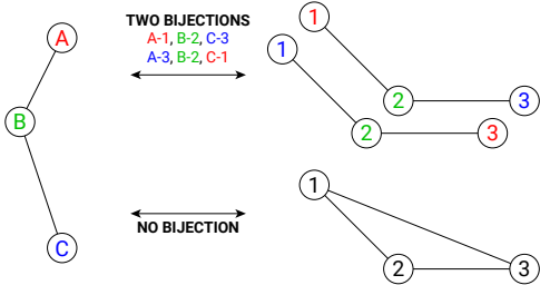
Figure 6.2 – Two graphs are isomorphic if a bijection exists between the vertices of two graphs that preserves the edge connectivity.
