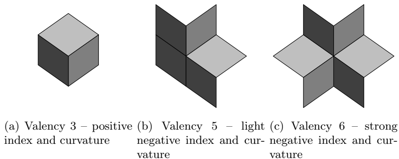
Figure 2.21 – Relation between valency, index and curvature in quad meshes with right angles.
