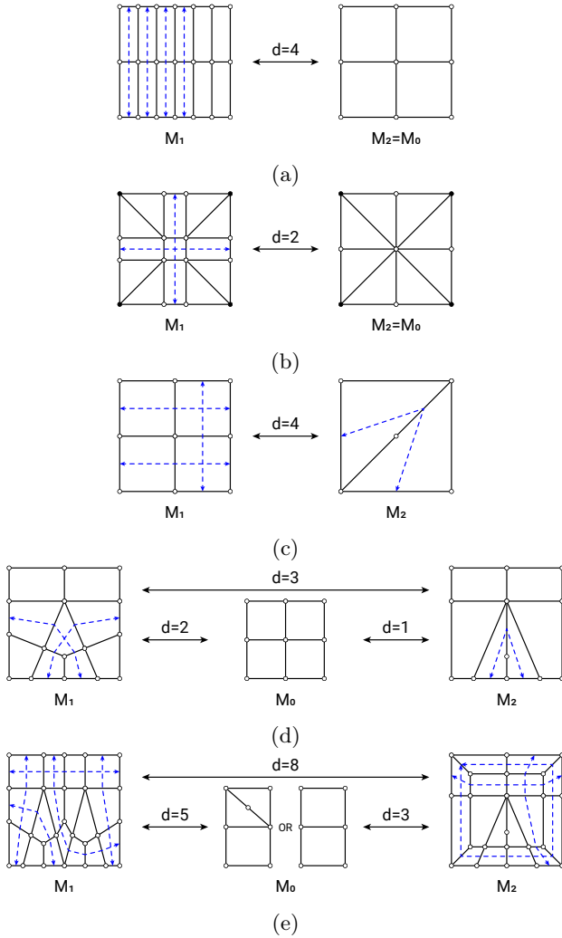
Figure 6.12 – Validation examples for computing the topological distance between two quad meshes. The distances between the meshes M_1 and M_2 and between their submesh M_0 is provided along with one of the possible combination of strips to delete in blue.
