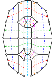
Figure 6.19 – The supermesh has ten strips, gathered in six coloured groups to preserve the twofold symmetry.
