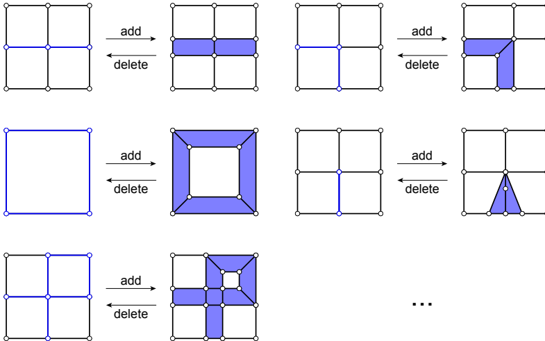
Figure 5.8 – Quad-mesh grammar of low-level rules for addition and deletion of strips with different configurations.
