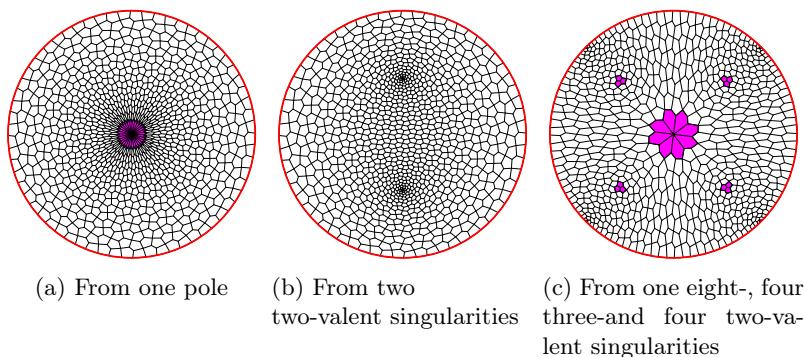
Figure 2.7 – Pentagonal tilings stemming from quad meshes with different singularities inducing different distortions when mapped to the same disc surface. The faces around the equivalent vertex singularities are highlighted in pink.
