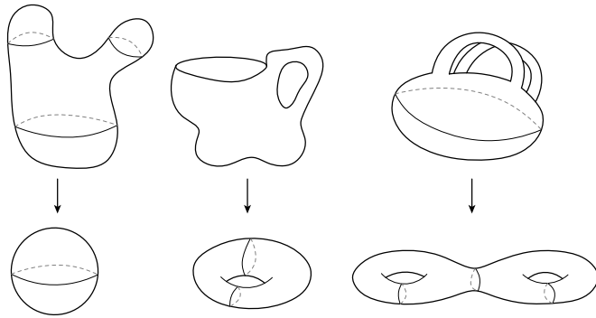
Figure 2.9 – Continuous and reversible deformation of a shape into another implies that they have the same shape topology. A sphere, a torus and double torus have different topologies. (Inspired from: learner.org)
