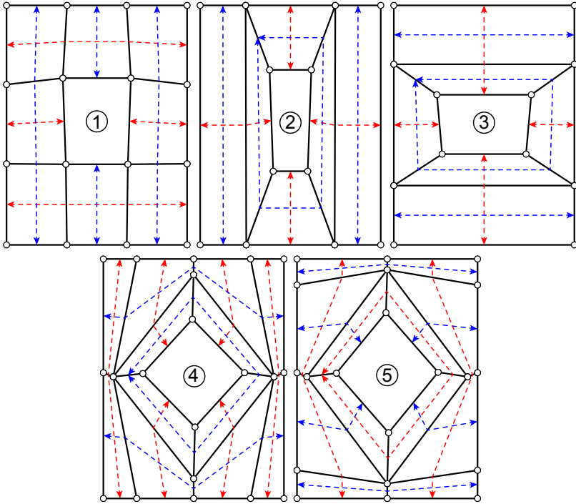
Figure 7.35 – Five symmetrical two-coloured topologies.
