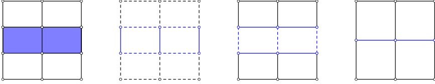
Figure 5.16 – Delete a strip.
