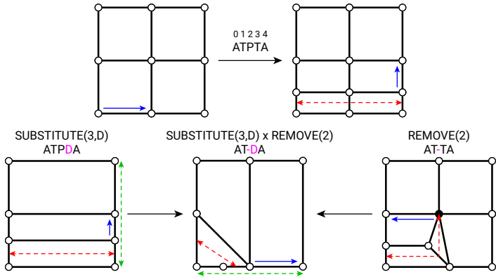
Figure 8.16 – Combining modifications: \text{substitute}(3,D) and \text{remove}(2) are applied on ATP\text{TA} to obtain AT\text{DA} . The results of the mutations are highlighted in pink.
