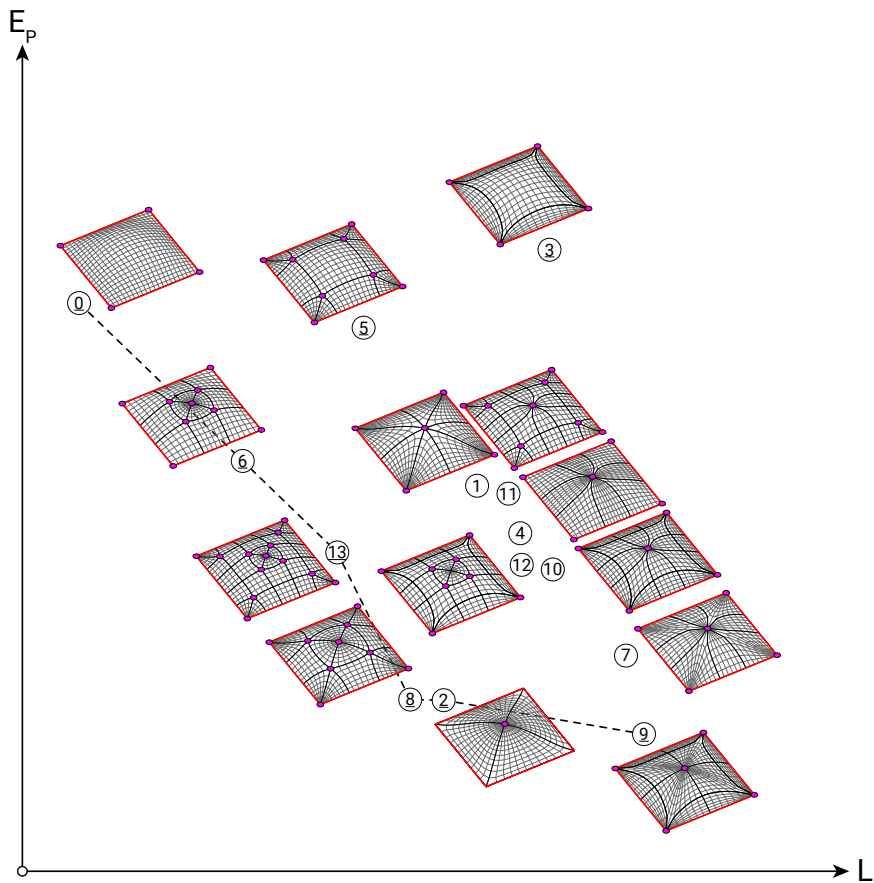
Figure 6.28 – Pareto front for the two metrics to minimised on edge-length disparity L and strain energy for a point load E_P . The Pareto designs for the three metrics are underlined.
