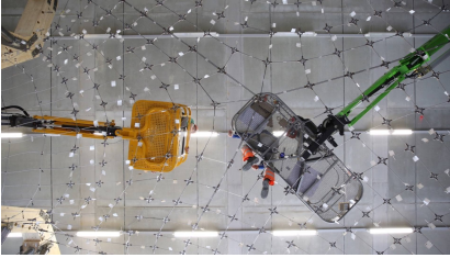
(c) Cable layout of the prototype for the NEST HiLo roof in Dübendorf, Switzerland [Méndez Echenagucia et al., 2018] (Photo credits: Naida Iljazovic)
