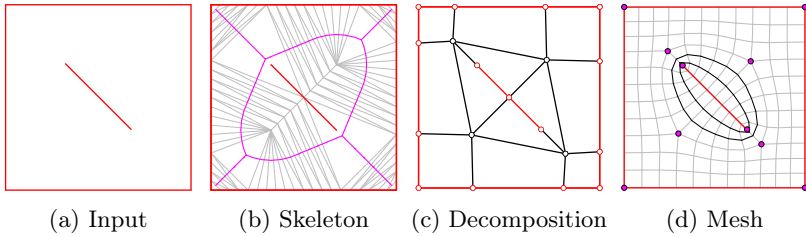
Figure 4.18 – Skeleton-based decomposition of a surface in a coarse quad mesh to yield a pattern aligned with curve features disconnected to the boundary.
