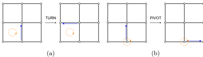
Figure 8.4 – The two movement operations to travel through the halfedges of a mesh.
