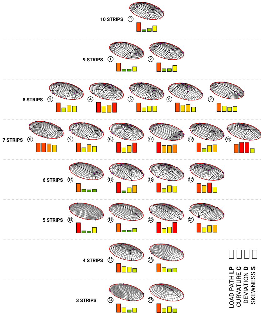
Figure 6.21 – Enumerating different topological designs for a dome on an elliptic boundary. The designs are organised based on topological similarity with design 0. All designs are close to a compression-only equilibrium against a vertical projected load and have quasi-planar faces. The bar charts show the multi-objective trade-offs. The 95%-Pareto designs are underlined.
