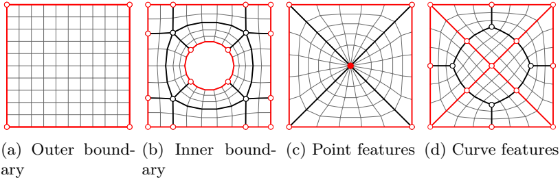
Figure 4.1 – Integrating geometrical aspects like boundaries and features in the design of quad-mesh patterns.
