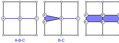
Figure 5.10 – Add a strip changing the density.
