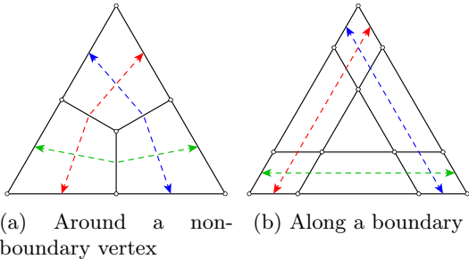
Figure 7.13 – Non-two-colourable coarse quad meshes because of odd numbers of strips.
