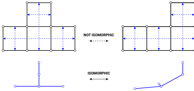
Figure 6.4 – Strip-graph isomorphism is not sufficient for quad-mesh isomorphism due to the lack of isomorphism between quad meshes and strip graphs.
