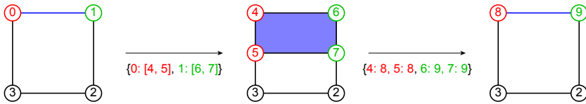
Figure 6.15 – Maps for vertex relabelling, in red and green, after strip addition and strip deletion rules, in blue.
