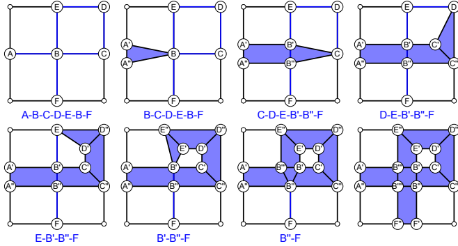
Figure 5.13 – Add a self-overlapping strip with update of the polyedge.
