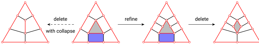
Figure 5.18 – When deleting some strips, in blue, refining other strips avoids boundaries to collapse to less than three edges and close an opening, in grey.
