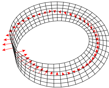
Figure 2.13 – The Möbius strip is a non-orientable shape because the normals in red can not be consistently oriented on the same side.
