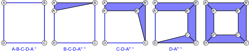
Figure 5.12 – Add a closed strip.
