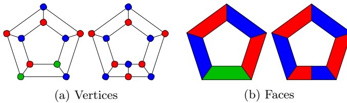
Figure 7.11 – The vertex and face elements along a closed strip can not be two-coloured if crossed by an odd number of elements. This number of elements can be tuned into an even number by modifying the density of the crossing strips.
