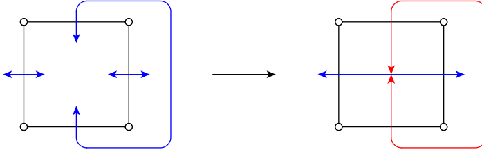
Figure 5.5 – Counting open strips S_o as one per edge E minus two per face F : S_o = E - 2F . Starting with one strip per edge, the connectivity of quad faces removes two open strips by merging open strips (in blue) or closing open strips (in red) for each pair of opposite edges.
