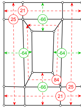
Figure 7.40 – The covariance in \text{kN}^2.\text{m}^2 of each strip with the structural performance when stiffened in the folded designs highlights their positive or negative influence.
