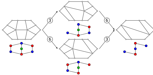
Figure 7.23 – Deleting two strips separately may not yield a two-colored quad mesh, but can yield a two-colored quad mesh at a farther distance in a new direction.
