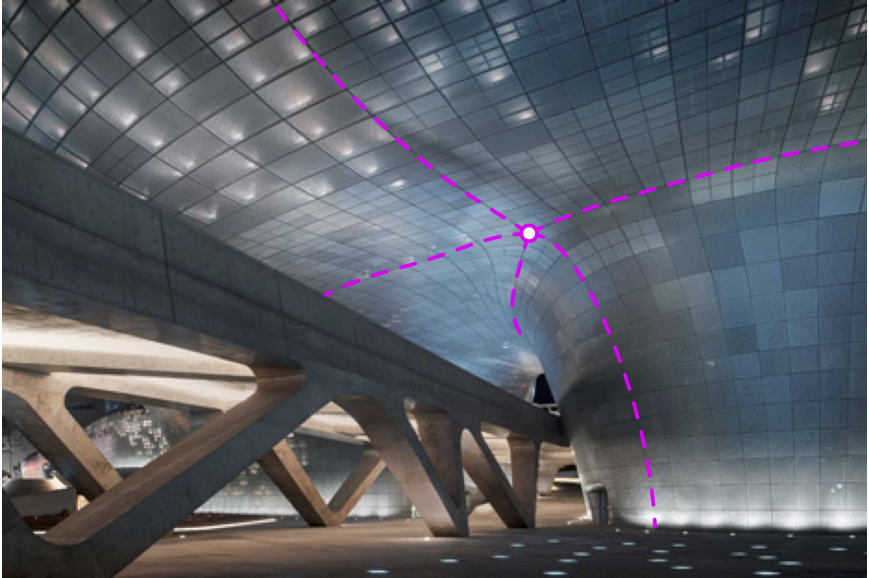
Figure 2.22 – The five-valent singularity in the cladding of the Dongdaemun Design Plaza in Seoul, South Korea, reduces panel distortion in the area with a negative curvature thanks to its negative index (source: dezeen.com).
