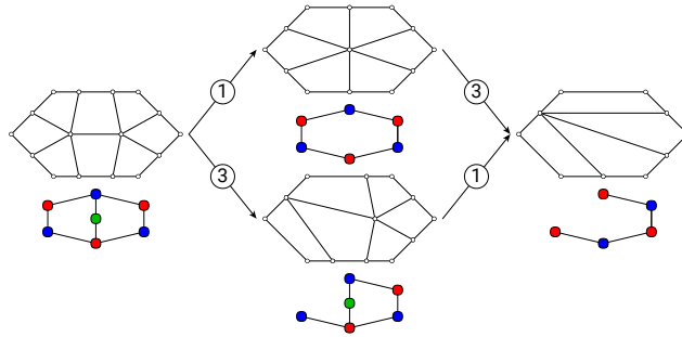
Figure 7.22 – Deleting a second strip of a two-colored quad mesh is redundant because it yields another two-colored quad mesh, but at a farther distance and in the same direction.
