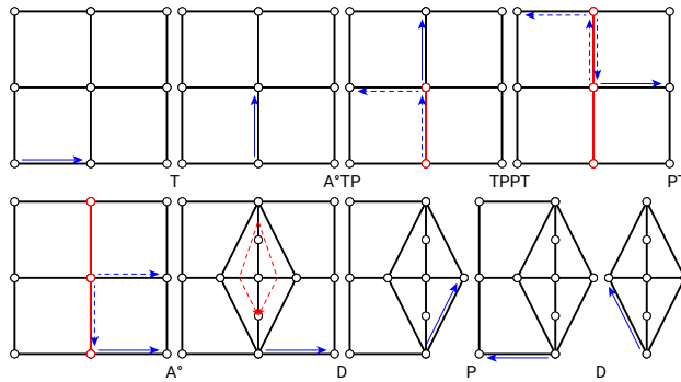
Figure 8.13 – The string T A^\circ T P T P P T P T A^\circ D P D adds another closed strip along the boundary and deleting two strips.
