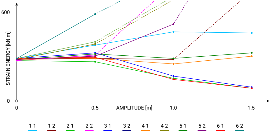
Figure 7.39 – Influence on the strain energy of introducing folds with different directions and amplitudes. Results above twice the initial strain energy are not shown, as evidenced by the dashed curves.
