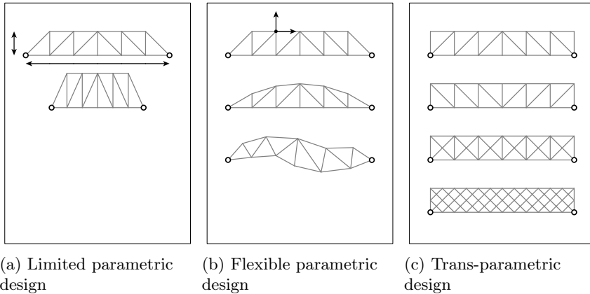
Figure 1.1 – Parametric and trans-parametric design spaces for a truss.
