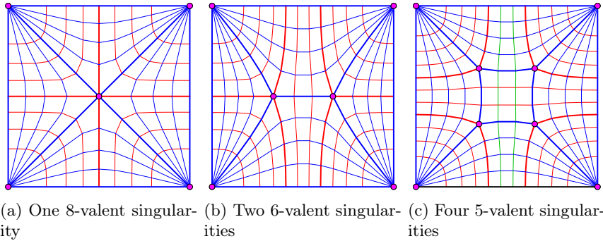
Figure 3.1 – Three similar but different quad-mesh patterns offer different pros and cons for structural design.
