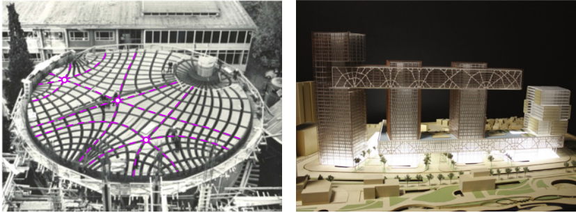
(c) The statics-integrated quad-mesh pattern of the zoology lecture hall at the University of Freiburg, Germany [Antony et al., 2014] (d) The topology-optimised quad-mesh pattern of the building bridge for the Zendai competition, China [Beghini et al., 2014]
