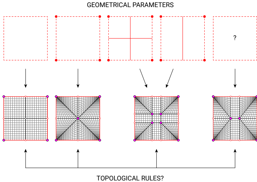
Figure 5.1 – Point and curve features in red serve as geometrical parameters in the skeleton-based decomposition for the generation of different designs inspired by the variations of Nervi slabs from Figure 3.1. The generation of these designs is not as intuitive, despite its topological similarity with the other designs.
