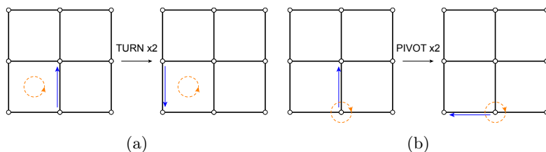
Figure 8.5 – Extension of the two movement operations with a parameter for multiple application of the operation.
