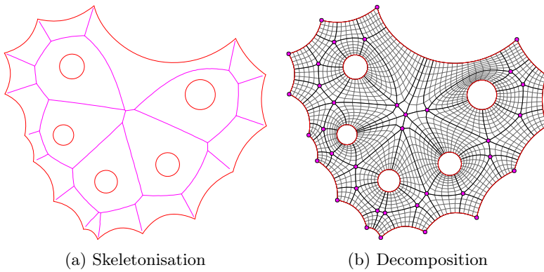
Figure 4.11 – Revisiting the roof of Solemar Therme in Bad Dürkheim, Germany, with a quad-mesh pattern including 38 singularities.
