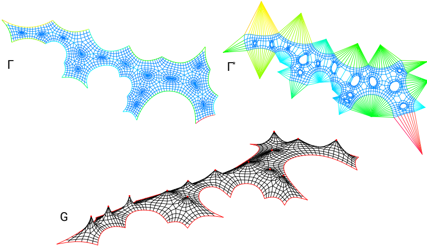
Figure 4.16 – Form diagram \Gamma , force diagram \Gamma^* and form-found network G for the Rhön-Klinikum Campus cable net using Thrust Network Analysis [Block and Ochsendorf, 2007] and RhinoVAULT [Rippmann et al., 2012, Rippmann and Block, 2013].
