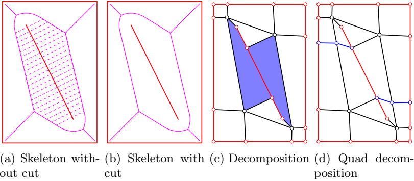
Figure 4.20 – Additional steps for skeleton-based generation of coarse quad meshes including curve features. Curve features are unwelded to avoid the crossing skeleton branches in dashed pink curves. Pentagonal or higher-valency faces, in blue, resulting from the unwelding become quad faces by propagating the seams of the discrepancies on the curve features.
