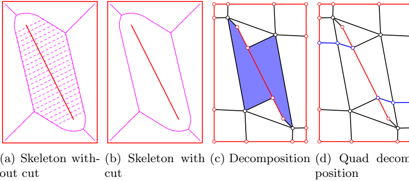
Figure 4.20 – Additional steps for skeleton-based generation of coarse quad meshes including curve features. Curve features are unwelded to avoid the crossing skeleton branches in dashed pink curves. Pentagonal or higher-valency faces, in blue, resulting from the unwelding become quad faces by propagating the seams of the discrepancies on the curve features.
