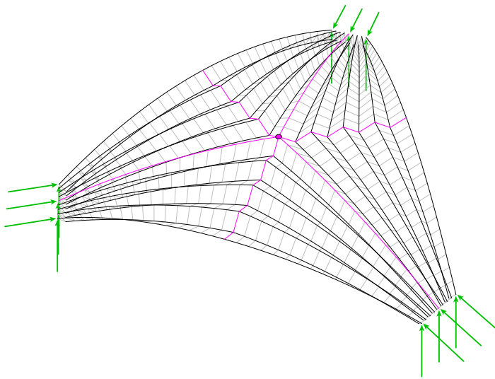
Figure 7.33 – Principle of the folding pattern of the CNIT. A six-valent singularity in pink provides a two-coloured pattern for stiffening the directions that carry the loads along the free edges directly to the supports in green. The stiff primary direction is in black and the secondary direction in grey.
