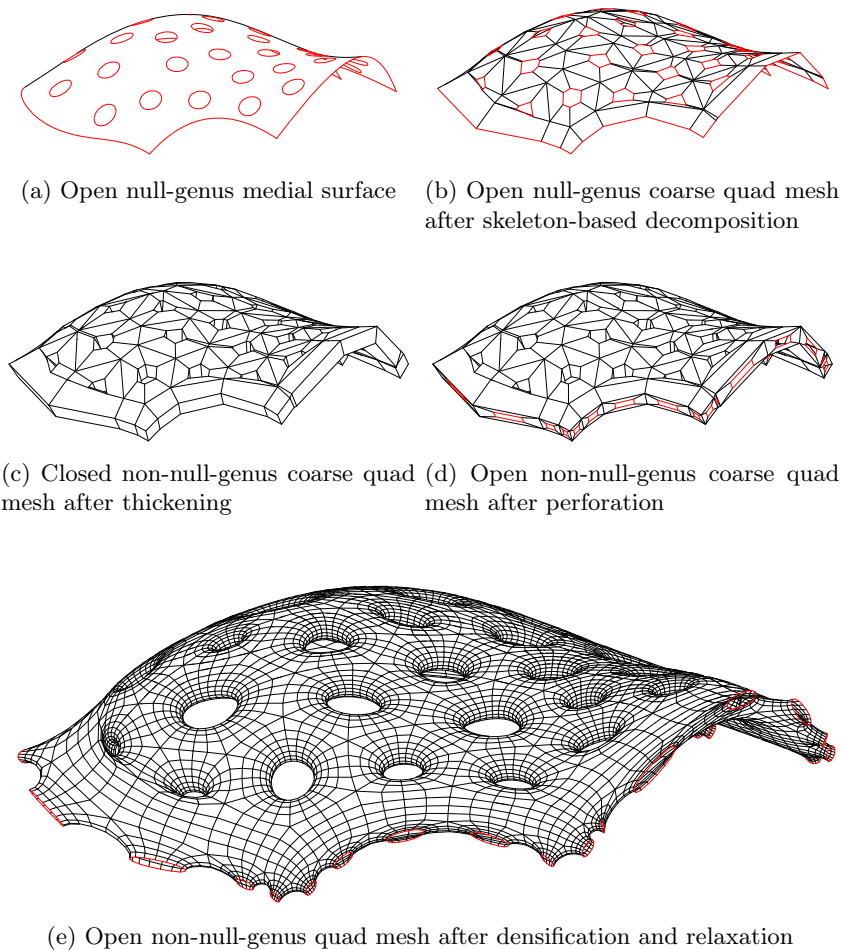
Figure 4.12 – The generation of a high-genus pattern aligned with boundaries and handles is performed thanks to skeleton-based decomposition of a medial surface. The design is inspired by the ICD/ITKE Research Pavilion of 2015/16 [Alvarez et al., 2018].
