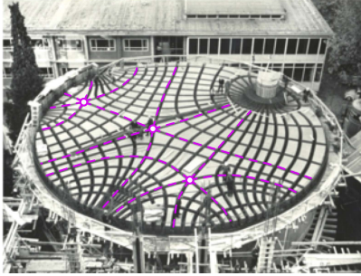
(c) The statics-integrated quad-mesh pattern of the zoology lecture hall at the University of Freiburg, Germany [Antony et al., 2014]
