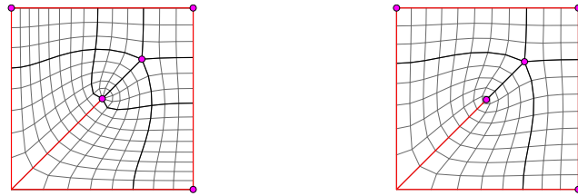
(a) A pole thanks to the missed-concavity operation (b) A two-valent singularity thanks to the unwanted-triangle operation
