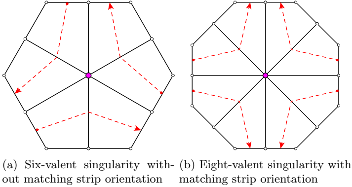
Figure 7.43 – 2k -valent singularities are adjacent to odd number of strips per colour, which does not provide the symmetry for matching directions, represented by the red arrows, between the strips of the same colour, opposed to 4k -valent singularities, which are adjacent to even number of strips per colour.
