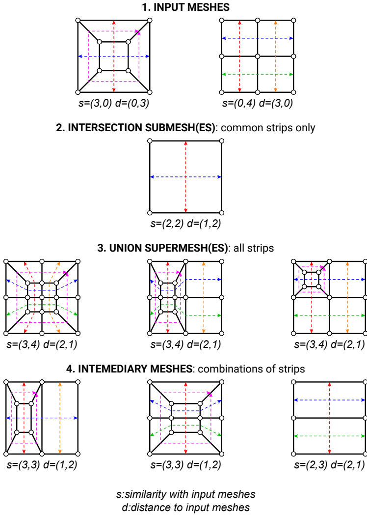
Figure 6.14 – Approach to generate hybrid quad meshes with different degrees of topological similarity with input quad meshes. The colours correspond to similar strips, supporting the values on the similarity and dissimilarity with the input meshes.
