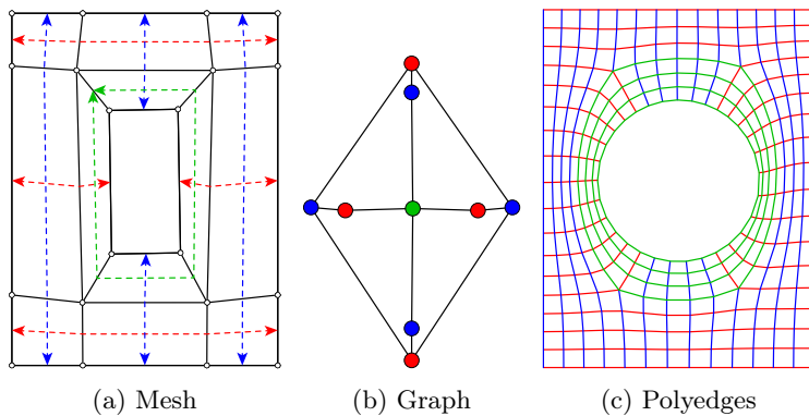
Figure 7.17 – Quad mesh without two-coloured polyedges evidenced by the three-coloured strip graph of its coarse quad mesh.
