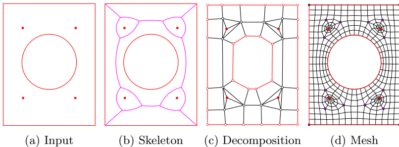
Figure 4.13 – Skeleton-based decomposition of a surface in a coarse quad mesh to yield a pattern aligned with the boundary and point features off the boundary.
