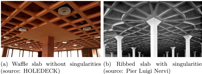
Figure 1.7 – Slab systems with different geometrical and topological regularities due to singularities in the patterns.
