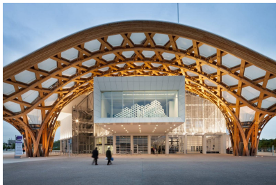
(c) Timber gridshell with a semi-regular, Kagome pattern of the Centre Pompidou in Metz, France (Source: damienguillou.fr)
