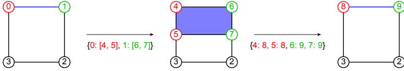
Figure 6.15 – Maps for vertex relabelling, in red and green, after strip addition and strip deletion rules, in blue.
