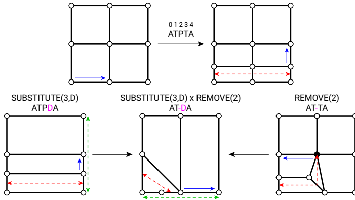
Figure 8.16 – Combining modifications: \text{substitute}(3,D) and \text{remove}(2) are applied on ATPTA to obtain ATDA. The results of the mutations are highlighted in pink.
