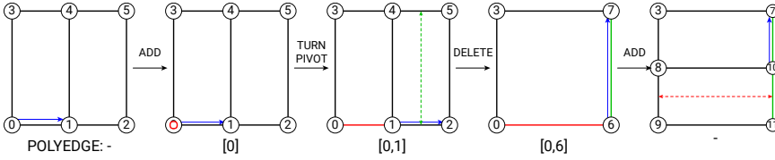
Figure 8.11 – The collected polyedge for strip addition, in red, updates when strip deletion applies, in green, by replacing the old vertices by the new ones.
