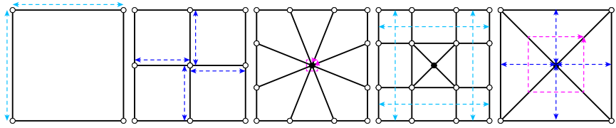
(a) Temporarily adding the strips in cyan to add the the strips in blue and pink to obtain a quad-mesh topology with a pole at the centre, to provide many load paths to the point load.
