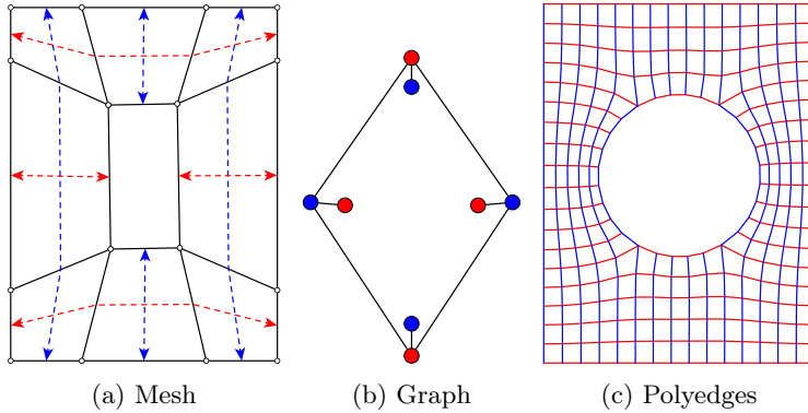
Figure 7.18 – Quad mesh with two-coloured polyedges after deletion of the third-colour strips, evidenced by new two-coloured strip graph of its coarse quad mesh.
