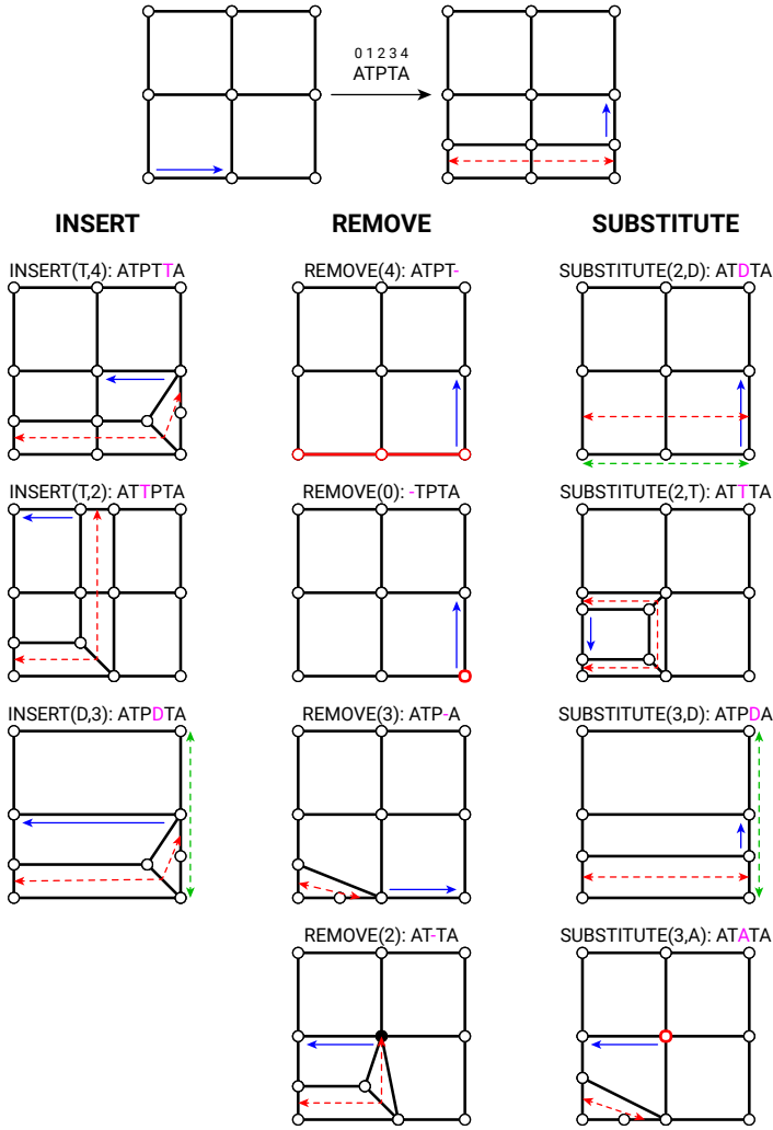
Figure 8.15 – Examples of application of the three types of letter modifications: insert, remove and substitute. The modifications in the initial string ATPTA are highlighted in pink. A dash marks the removed letters in the string. The added strip and collected polyedge are highlighted in red and the deleted strips in green.
