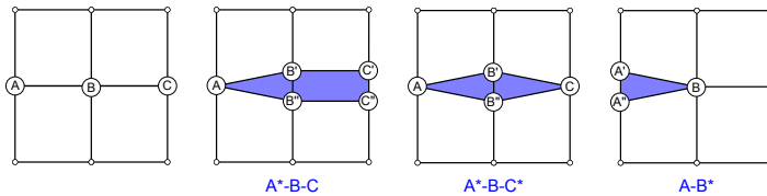
Figure 5.15 – Add strips with poles.
