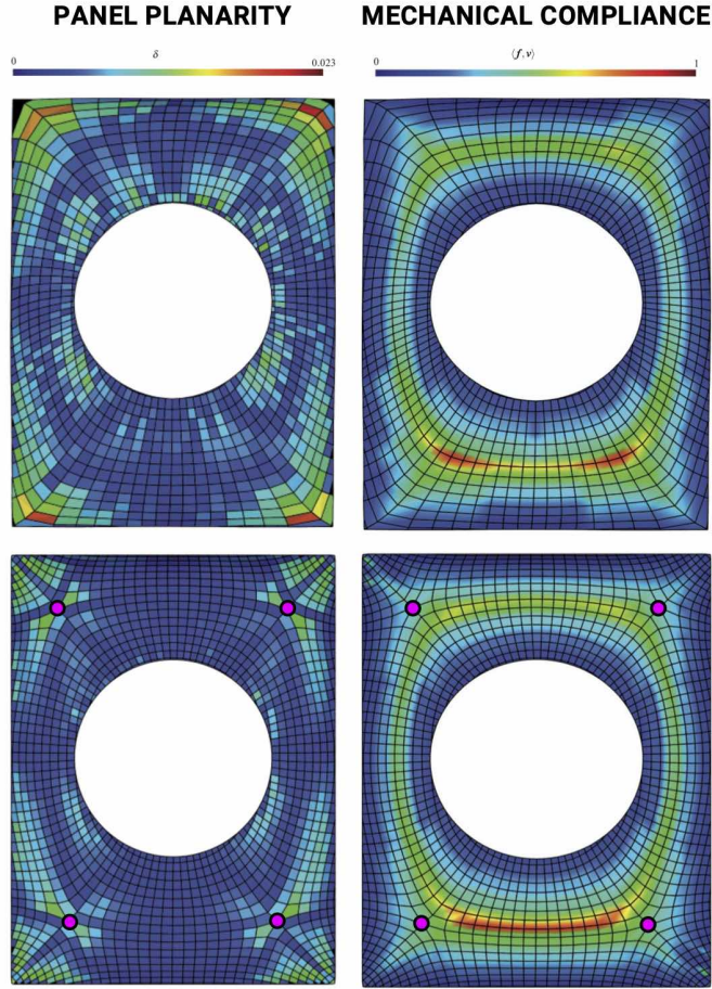
Figure 2.2 – Two pattern designs revisiting the British Museum roof. The topology at the top performs the best regarding the requirement on the right on minimising mechanical compliance. The topology at the bottom performs the best regarding the requirement on the left on minimising panel planarity [Schiftner and Balzer, 2010]. The singularities in a quad mesh, highlighted in pink, influence its efficiency and affordability, highlighting the importance of their design for the challenge of meeting trade-offs in multi-objective structural design.
