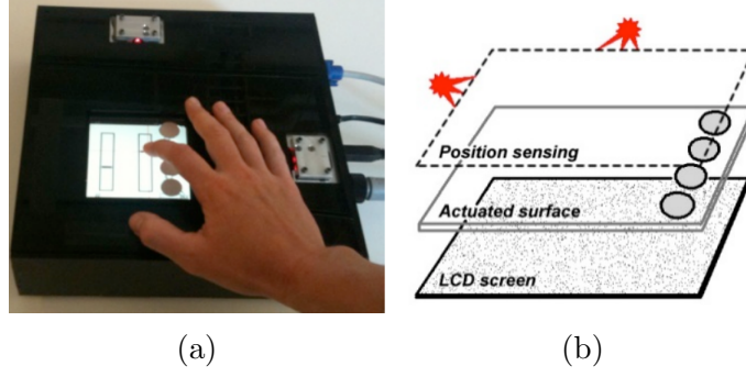
Figure 2.23: a) Picture and b) structure of the variable friction device, from [60].
