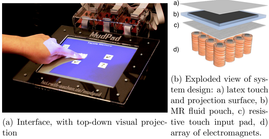
Figure 2.7: MudPad interface, from [44].
