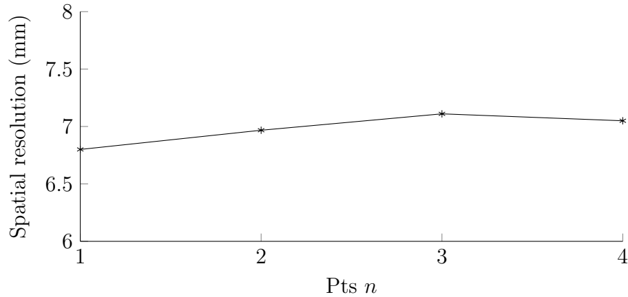
Figure 4.34: Spatial resolution of each focus point.
