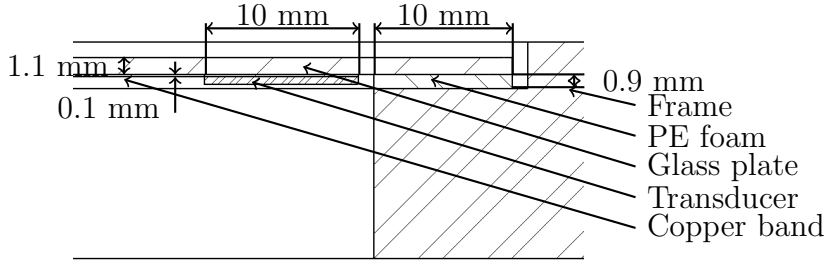
Figure 4.2: Section of the haptic display.
