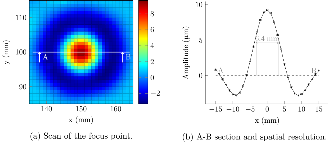
Figure 4.20: Spatial characteristics of the focus point for 1b signals with filtering
