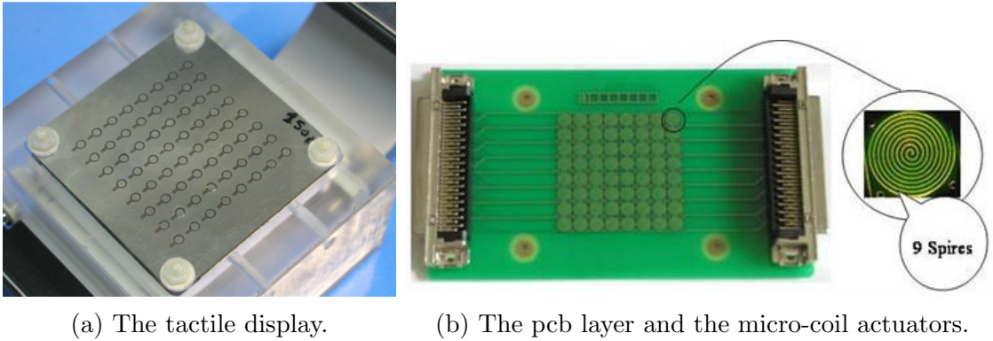
Figure 2.16: VITAL, an 8 by 8 vibrotactile display with an integrated laser-cut flexible membrane, from [4].
