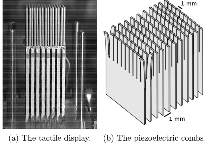
Figure 2.17: STReSS device with piezoelectric benders, from [66].
