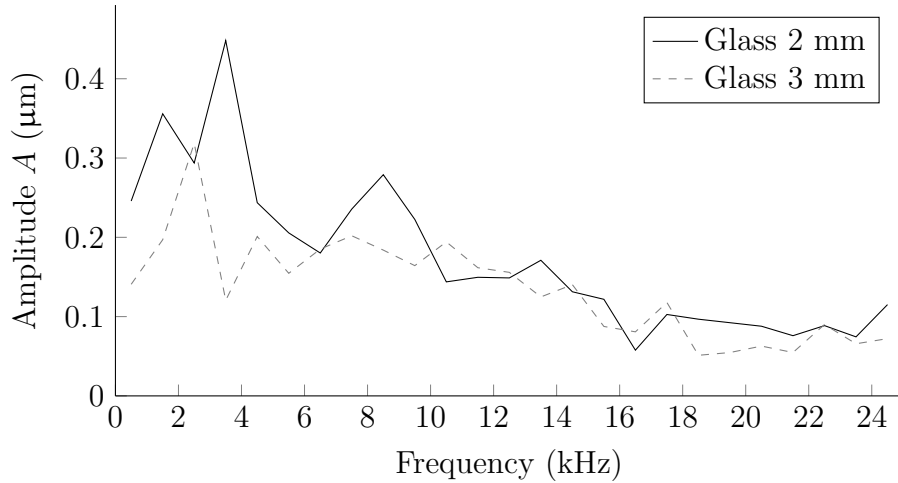
Figure 3.11: Displacement amplitude A of focus point for the ø12 mm transducers.
