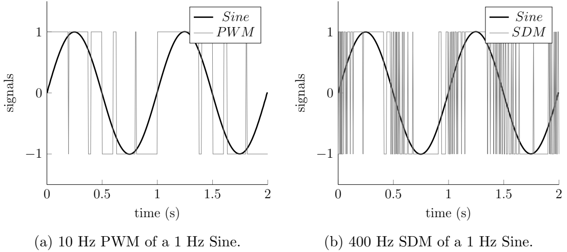
Figure 4.6: Comparison between PWM and SDM modulation methods.
