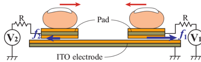
(a) Pads with different voltages stimulate fingers independently.
