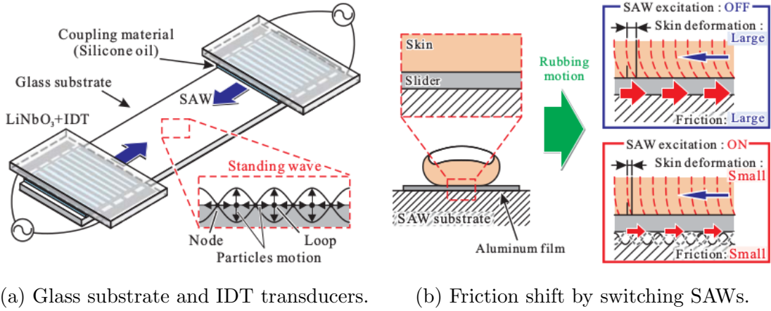
Figure 2.20: Variable friction interface with SAWs, from [56].
