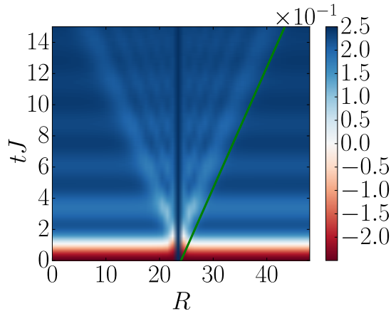
Figure 5.24: Spreading of the spin correlations along the z axis \langle \hat{S}_R^z(t) \hat{S}_{N_s/2}^z(t) \rangle for a sudden local quench in the local regime of the z polarized phase (lin-lin scale). The space-time spin correlations have been computed using the t-MPS + TDVP technique for J/h = 2 \times 10^{-2} and \alpha = 2.1 > 2 for a locally perturbed initial state |\Psi_0\rangle \simeq |\uparrow \dots \uparrow \downarrow \uparrow \dots \uparrow\rangle . The solid green line represents a ballistic fit to the motion of the CE (correlation edge). The associated slope V_{\text{CE}}^{\text{num}} has been found to be in excellent agreement both with the numerical spin edge velocity V_{\text{SE}}^{\text{num}} and the theoretical maximal group velocity V_g^* (see Fig. 5.22(b) for the values of V_{\text{SE}}^{\text{num}} and V_g^* ). Note that contrary to the local magnetization the spin correlations display another time-dependent term irrelevant for our study, see Fig. 5.22(a).
