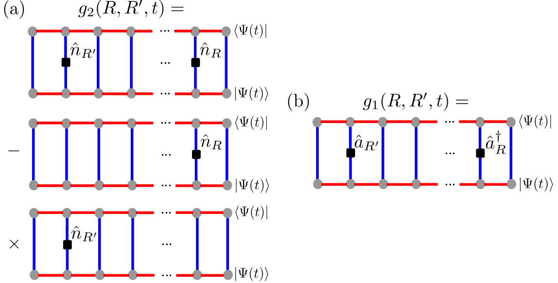
Figure 4.8: Graphical representation of correlators using tensor networks. (a) The equal-time correlation function g_2(R, R', t) = \langle \hat{n}_R(t)\hat{n}_{R'}(t) \rangle - \langle \hat{n}_R(t) \rangle \langle \hat{n}_{R'}(t) \rangle allowing to characterize the connected density-density correlation function G_2(R, t) = g_2(R, t) - g_2(R, 0) (for R' fixed to 0) in order to investigate the density fluctuations of a 1D particle lattice model. (b) The equal-time correlation function g_1(R, R', t) = \langle \hat{a}_R^\dagger(t)\hat{a}_{R'}(t) \rangle to characterize the connected one-body correlation function G_1(R, t) = g_1(R, t) - g_1(R, 0) (for R' fixed to 0) in order to investigate the phase fluctuations of a 1D particle lattice model.
