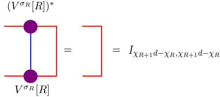
Figure 5.11: Graphical representation using tensor networks of the second condition fulfilled by the projector V[R] in order to find that the matrix X[R] corresponds to the single effective parameter of the tensor B[R] . The latter allows to explore the MPS tangent plane \mathcal{T}_{|\Psi(\{A\})\rangle} of the reference state |\Psi(\{A\})\rangle . The second condition on V[R] is the right normalization defined as \sum_{\sigma_R} V^{\sigma_R}[R] (V^{\sigma_R}[R])^\dagger = I_{\chi_{R+1}d - \chi_R, \chi_{R+1}d - \chi_R} .
