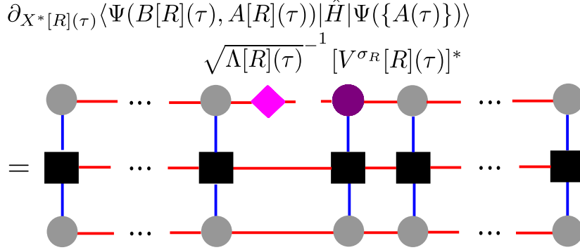
Figure 5.14: Graphical representation using tensor networks of the first term on the left-hand side of Eq. (5.41). Since the isometric gauge is considered, one should add to this graph the left and right gauge-fixing conditions of the isometric gauge provided at Fig. 5.6.
