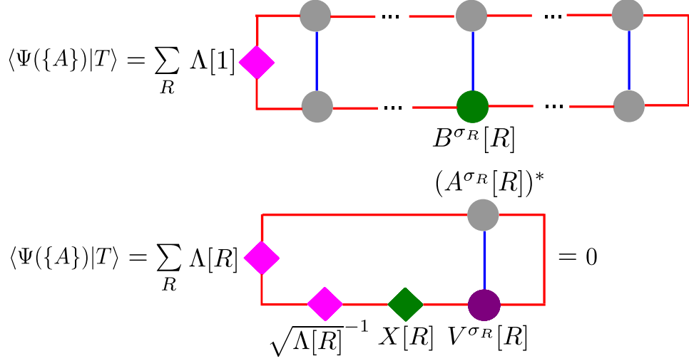
Figure 5.10: Demonstration using tensor network language of the orthogonality between a reference quantum state |\Psi(\{A\})\rangle and a tangent vector |T\rangle by computing the overlap \langle \Psi(\{A\}) | T \rangle . To demonstrate that \langle \Psi(\{A\}) | T \rangle = 0 , one has to use the following condition \sum_{\sigma_R} V^{\sigma_R}[R] (A^{\sigma_R}[R])^\dagger = 0_{\chi_{R+1}d - \chi_R, \chi_R} fulfilled by the projector V[R] .
