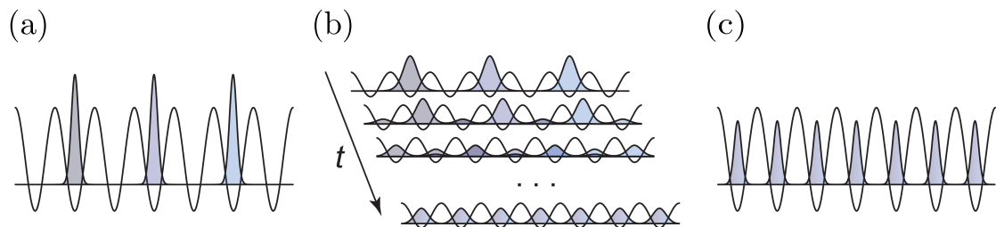
Figure 2.1: Quench and measurement protocols for the experimental investigation of the far-from-equilibrium dynamics of a density wave for an isolated one-dimensional Bose gas. (a) Preparation: the quantum system is initially prepared in a density wave |\Psi_0\rangle , see Eq. (2.10), requiring a large lattice depth to maximize the energy ratio U/J . (b) Evolution: a global quench is applied to the lattice model at t = 0^+ by reducing suddenly the lattice depth (or equivalently the ratio U/J ) permitting a tunneling process for bosons on nearest lattice sites. (c) Readout: the properties of the time-evolved quantum state |\Psi(t)\rangle are read out by freezing the time evolution of the quantum system by suppressing the tunneling process. Figure extracted and adapted from Ref. [21].
