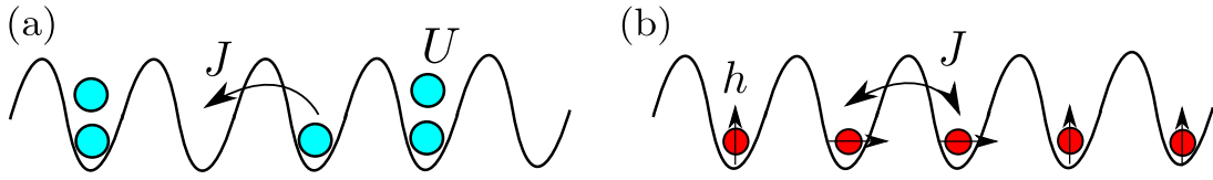
Figure 3.1: Short-range interacting lattice models. (a) Sketch of the 1D short-range Bose-Hubbard model representing interacting bosonic particles in an optical lattice. (b) Sketch of the 1D short-range interacting transverse Ising model corresponding to spins s = 1/2 interacting via an antiferromagnetic interaction J > 0 while an uniform and constant transverse magnetic field h > 0 is applied along the z axis favorizing the spins to align along this direction.
