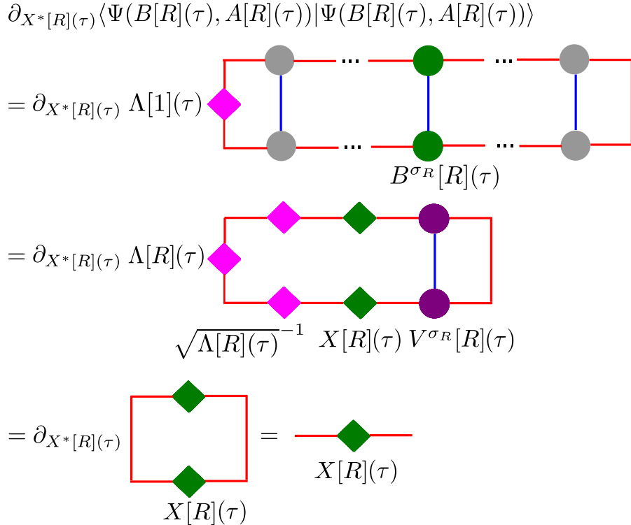
Figure 5.15: Graphical representation using tensor networks of the second term on the left-hand side of Eq. (5.41).
