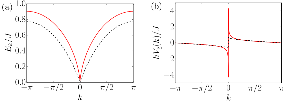
Figure 3.11: Excitation spectrum properties of the 1D LRXY model in the x polarized phase. (a) Excitation spectrum rescaled by the spin exchange coupling E_k/J as a function of the quasimomentum k in the first Brillouin zone \mathcal{B} = [-\pi, \pi] in the quasi-local regime for \alpha = 2.3 (red solid line) and in the local regime for \alpha = 3.3 (black dashed line). (b) Dimensionless quantity \hbar V_g(k)/J , where V_g denotes the group velocity, as a function of the quasimomentum k for the same power-law exponents \alpha . For \alpha = 2.3 (red solid line), V_g diverges at k \rightarrow 0 whereas for \alpha = 3.3 (black dashed line), it is finite over the first Brillouin zone.
