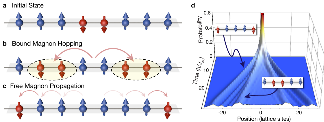
Figure 2.11: Spreading of magnonic excitations in the 1D short-range Heisenberg model. (a) Initial many-body quantum state where both central 'up' spins are flipped, ie. |\Psi(0)\rangle = |\uparrow \dots \uparrow \downarrow \downarrow \uparrow \dots \uparrow\rangle , and its decomposition into bound (b) and free (c) magnons propagating through the lattice chain. (d) Numerical result obtained from exact diagonalization showing the probability to find a flipped ('down') spin at a given lattice site following the initial state preparation. Note that on panel (d), two different wavefronts corresponding to bound and free magnons can be identified (see insets). The maximum probability ( P_{\max} = 1 at t = 0 \times (\hbar/J_{\text{ex}}) for both central lattice sites) was clipped in the graph for clarity. Figure extracted from Ref. [110].
