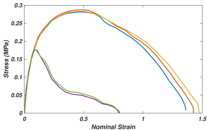
FIGURE 2.16: Probe tack test result repeatability
