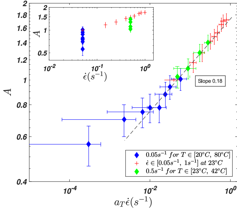
FIGURE 3.20: The two graphs represent the evolution of the shift factor \mathcal{A} . The small graph regards its evolution with respect to \dot{\epsilon} and T . On the main graph, \mathcal{A} is plotted with respect to the normalized strain rates a_T \cdot \dot{\epsilon} .
