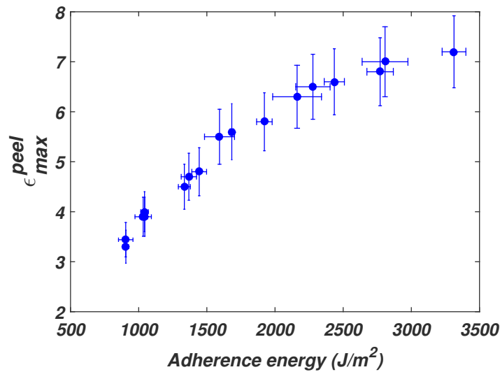
FIGURE 3.17: Maximal extension of equivalent fibrils measured in peeling at 90^\circ
