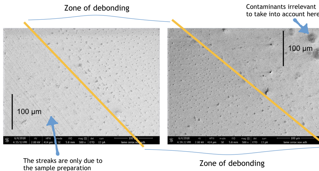
FIGURE 4.18: SEM observation of the substrate surface after debonding. The zone of debonding corresponds to the area where the foam PSA was peeled off.
