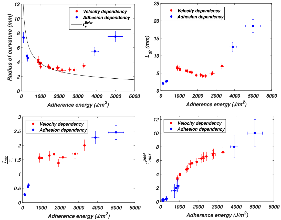
FIGURE 4.13: Radius of curvature r_c , debonding region length L_{dr} , ratio \frac{L_{dr}}{r_c} , maximal extension \epsilon_{max}^{peel} evolutions with respect to the adherence energy. Peelings at 90^\circ in triggering the peeling velocity (in red) and substrate surface chemistry (in blue).
