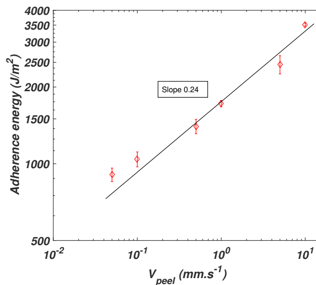
FIGURE 3.6: Evolution of the adherence energy with respect to the peeling velocity. Samples are peeled on glass substrates (see 2.3 for substrate preparation)
