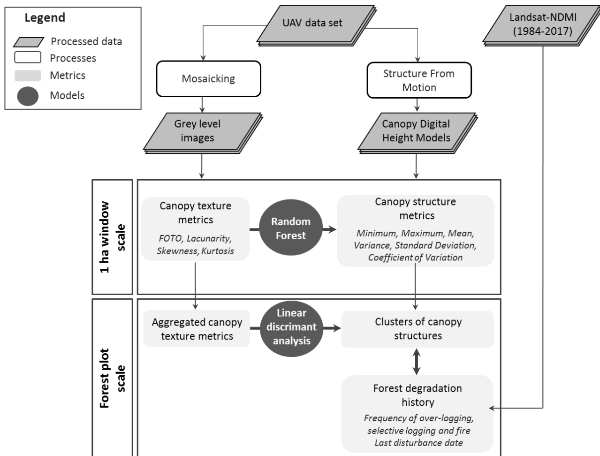
Figure 3.3 Workflow of the method used to evaluate the potential of canopy texture metrics to retrieve the canopy structure along the gradient of forest degradation and their relation with forest degradation history.
