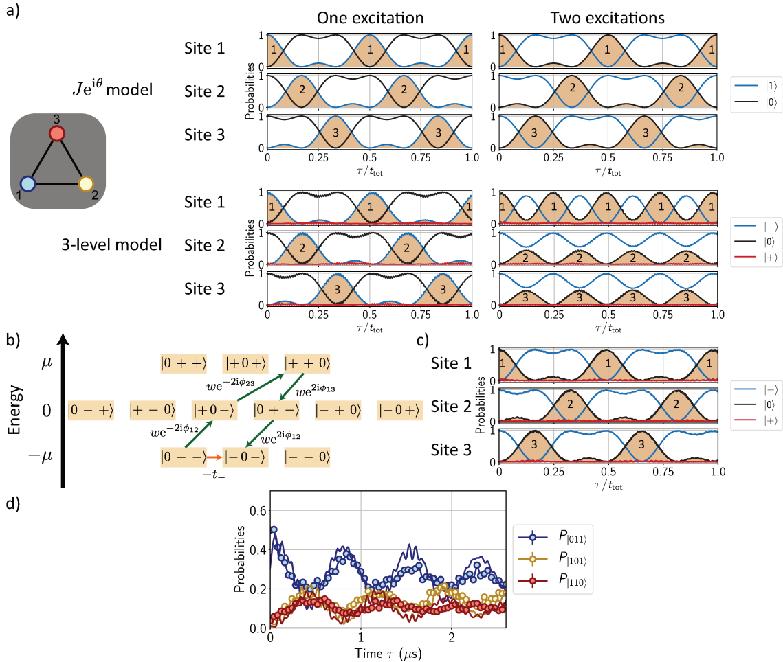
Figure 6.12: Two-excitation case. (a) Comparison of the one- and two-excitation cases, for the J e^{i\theta} model or Hamiltonian (6.3). We plot as a function of time the site-dependent probabilities to be in the particle state ( |1\rangle or distinguishing between the spin states |-\rangle and |+\rangle for the three-level model) or the vacuum state |0\rangle . The total duration t_{\text{tot}} was set in order to have in the one-excitation case two cycles of the periodic motion. (b) Perturbative approach in the two-excitation case, revealing a fourth-order off-resonant process. (c) Same as (a) for Hamiltonian (6.3), but increasing both w and \mu by a factor 210 to obtain again two cycles of the periodic motion of a hole. (d) Measured probabilities to be in the different two-excitation states as a function of time, after having prepared |0--\rangle , for the parameters corresponding to the circular motion in the single-excitation case.
