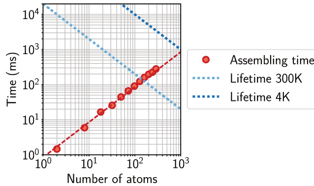
Figure 7.3: Towards larger systems. Comparison between the assembling time and the vacuum-limited lifetime of a configuration, as a function of the number of atoms.
