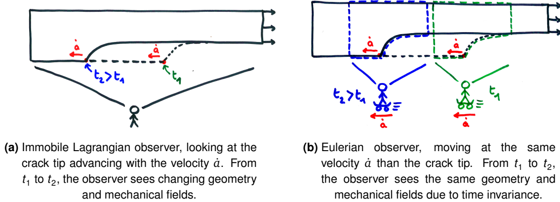
Figure VI.5 Illustration of the Lagrangian vs. Eulerian frameworks in a steady-state regime.
