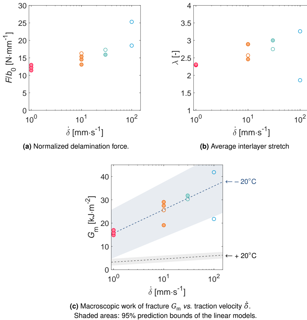
Figure V.10 TCTT values for increased MTES-treated glass, at -20^\circ\text{C} . Filled symbols: steady-state delamination. Open symbols: rupture of the interlayer.
