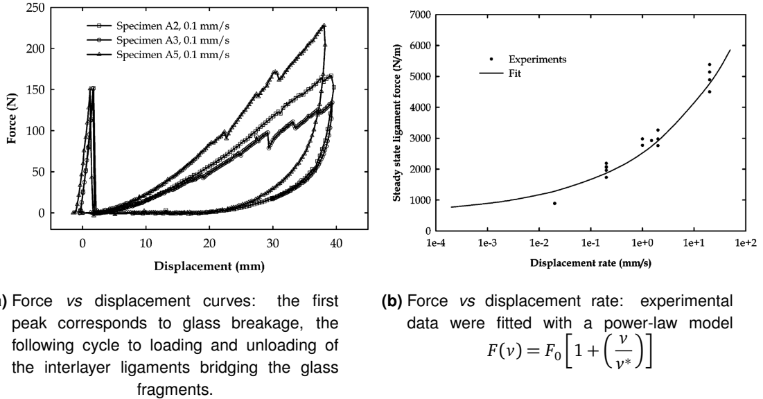
Figure I.6 Flexural and indentation test on laminated glass, from Seshadri et al. [26]
