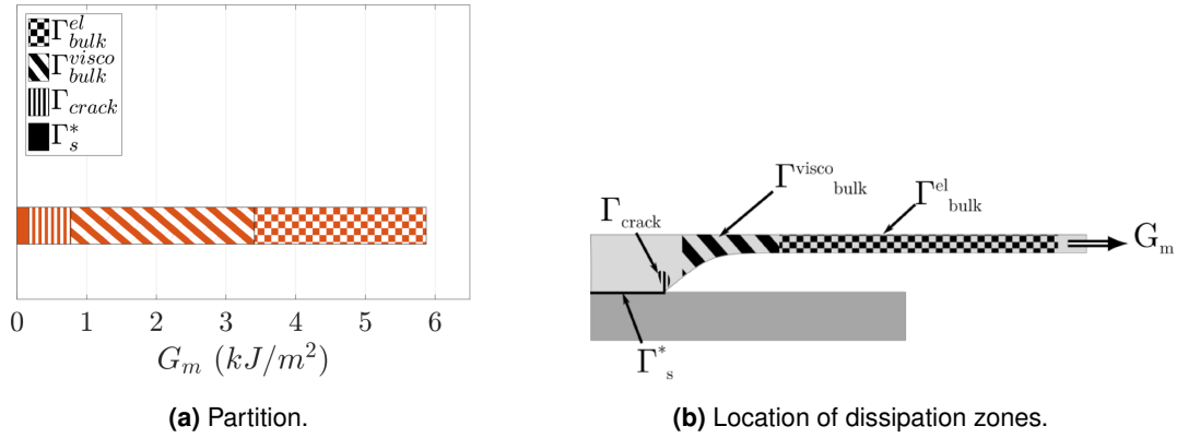
Figure VI.1 Macroscopic work of fracture, from Elziere.
