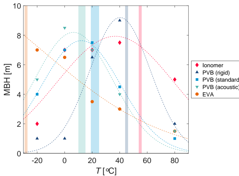
Figure I.4 Mean Break Height of laminates made of different interlayers, measured at temperatures from -20°C to 80°C. Dashed lines are gaussian fits made to highlight the optimum of performance. Shaded bars indicate the glass transition temperature of each polymer. Data from Novotny & Poot (2016) [12]
