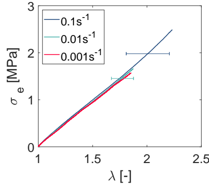
Figure IV.9 Tensile test to rupture for EVA at 80°C. The errorbars indicate the standard deviation of the strain at break (3 samples).
