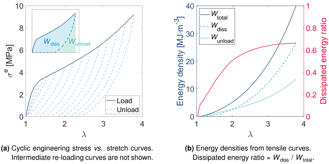
Figure IV.10 Cyclic tensile tests on EVA at 20°C.
