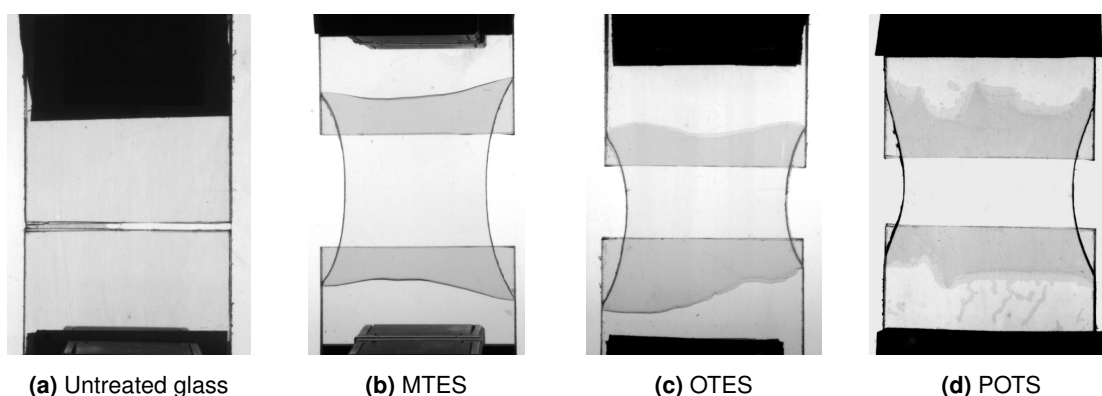
Figure V.4 Through Crack Tensile Test of EVA for various surface chemistries. ( T = 20^\circ\text{C} , \dot{\delta} = 10 \text{ mm}\cdot\text{s}^{-1} )
