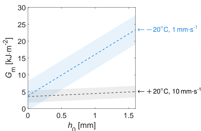
Figure VII.4 TCTT with EVA laminates: macroscopic work of fracture vs. interlayer thickness, at ambient temperature and close to the glass transition.
