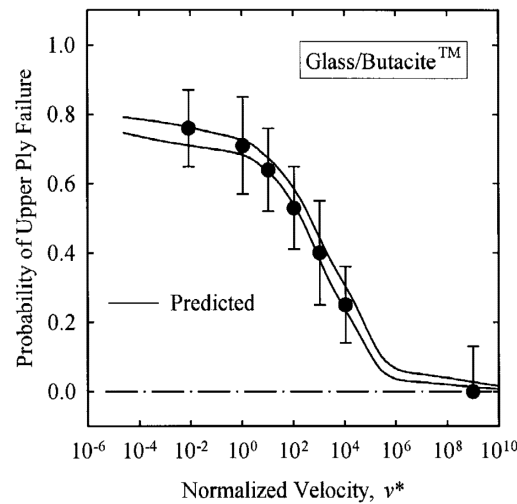
Figure I.5 Probability of upper glass ply failure vs velocity in biaxial flexure, from Bennison et al. [19]
