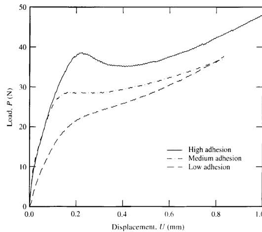
Figure I.10 TCTT force-displacement curves for high, medium and low adhesion PVB laminates at low strain rate ( \dot{\delta} = 8.5 \cdot 10^{-6} \text{ m} \cdot \text{s}^{-1} ) [35]
