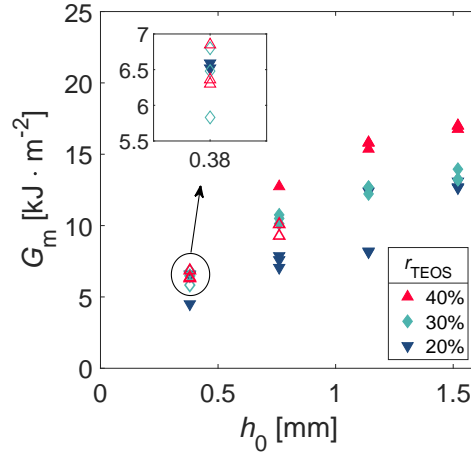
Figure III.10 Experimental macroscopic work of fracture. Filled symbols: steady-state delamination. Hollow symbols: interlayer rupture after partial delamination.
