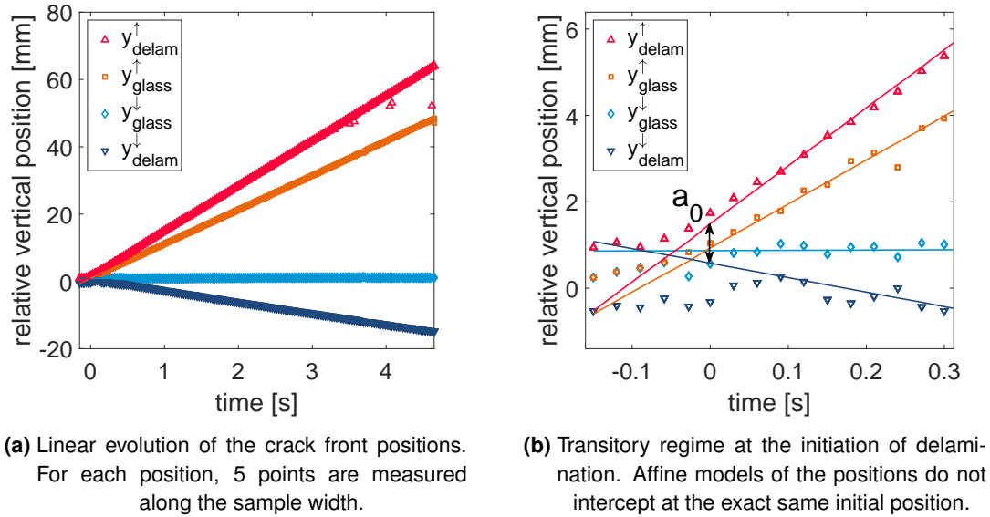
Figure II.11 Positions of delamination fronts and glass cracks over time in the TCTT.
