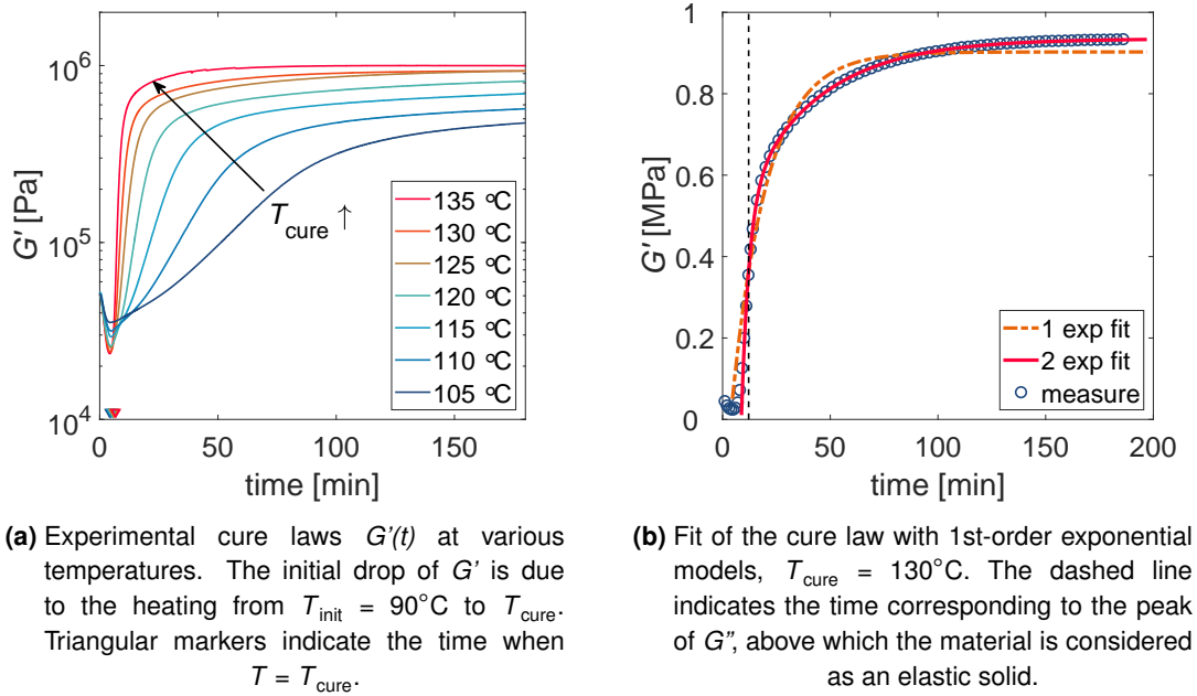
Figure IV.4 Curing behavior of EVA: time evolution of the storage shear modulus G' increases at constant temperature T_{\text{cure}} .
