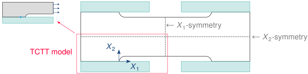
Figure VI.4 Steady-state model of the TCTT: the X_1 -axis and X_2 -axis symmetries allow to model only one quarter of the model.
