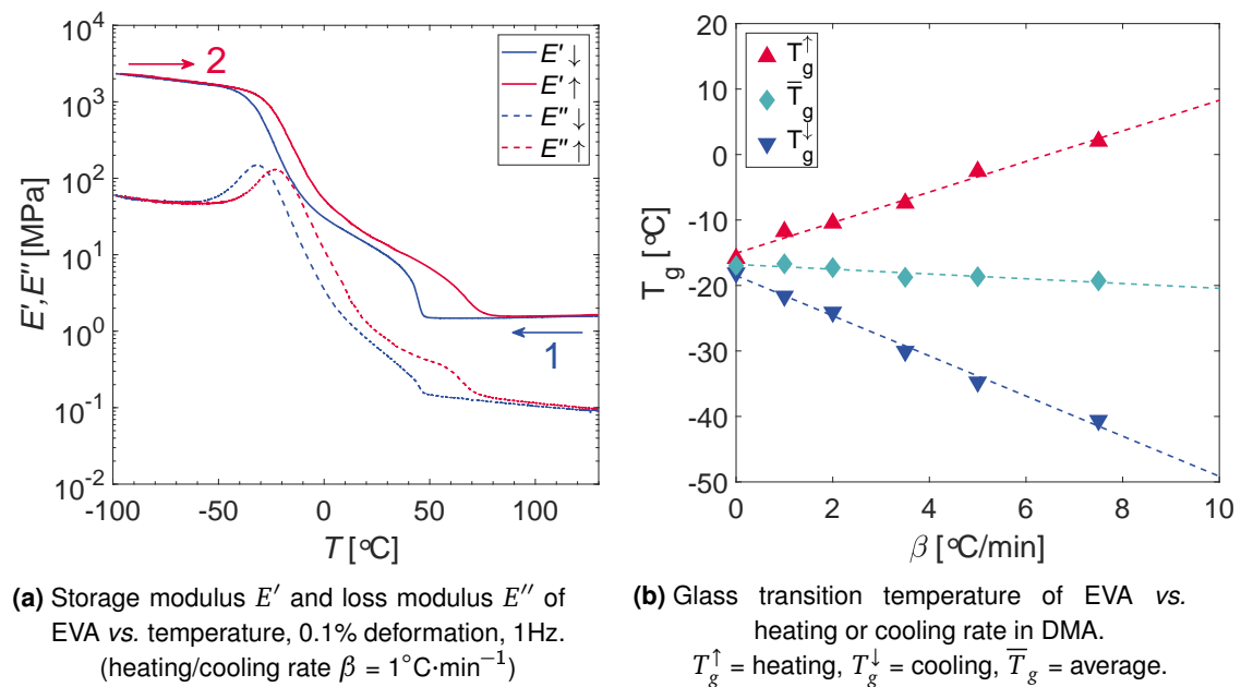
Figure IV.6 DMTA of EVA. Glass transition occurs around -20^\circ\text{C} and crystallization/fusion around 50^\circ\text{C} to 80^\circ\text{C} (frequency = 1Hz, deformation = 0.1%).
