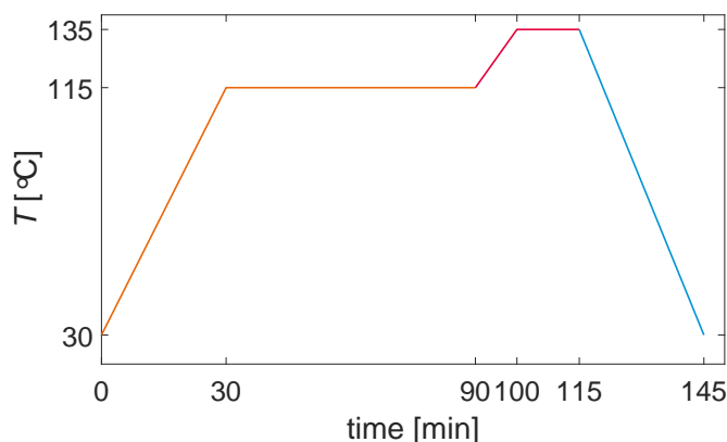
Figure IV.1 Thermal cycle for EVA lamination
