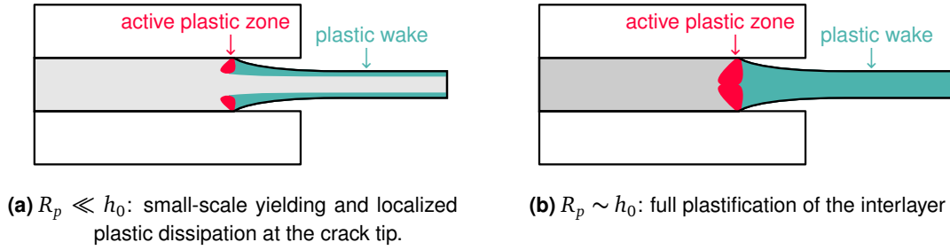
Figure V.7 Scenarii of plastic dissipation in the TCTT: (a) small-scale yielding vs. (b) development of the active plastic zone over the entire thickness of the interlayer.
