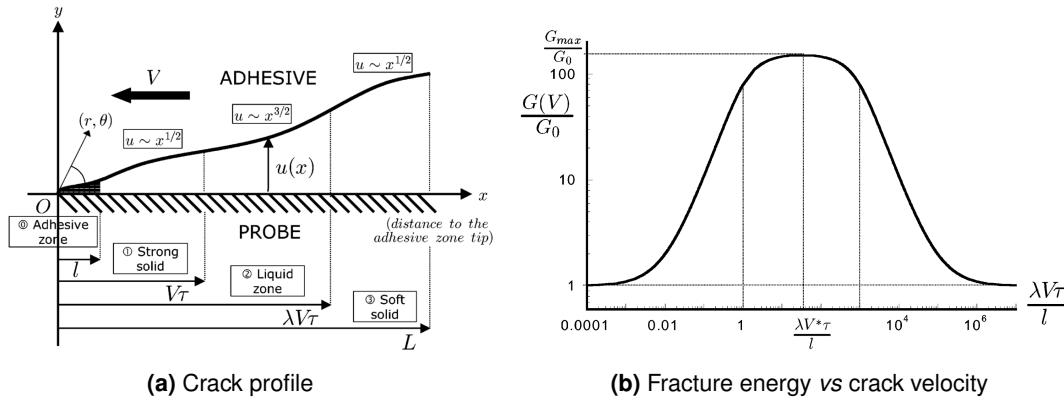
Figure I.12 De Gennes' “viscoelastic trumpet” model: the maximum value of G/G_0 is given by \lambda = \mu_0/\mu_\infty , the ratio of instantaneous modulus over relaxed modulus. From Saulnier et al. [51]
