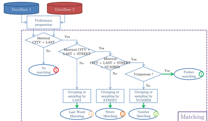
Fig. 2. Structure of the matching algorithm
