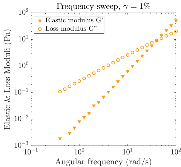
Figure 2.14 Frequency sweep tests on alginate solution ( M_w = 250 kg/mol, [alginate] = 13.1 g/L): elastic ( G' ) and loss ( G'' ) moduli against angular frequency \omega .
