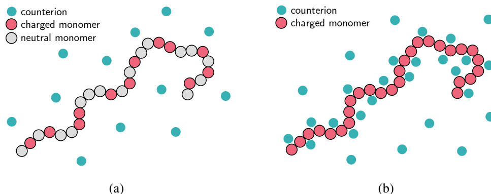
Figure 2.2 Schematic representation of a polyelectrolyte solution: Manning-Oosawa counterion condensation. (a) Weakly charged polyelectrolyte. (b) Strongly charged polyelectrolyte and condensation phenomenon.
