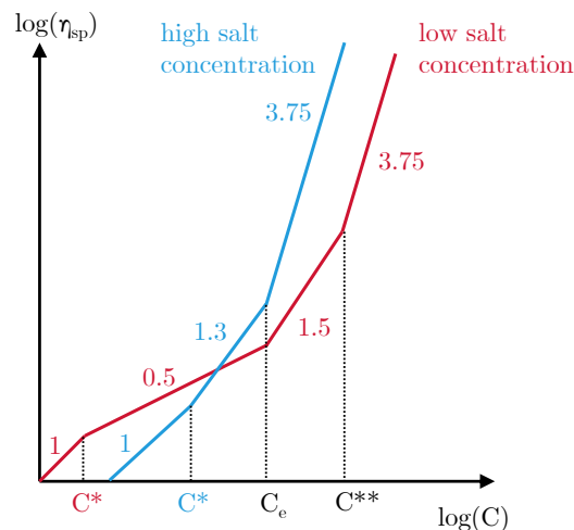
Figure 2.4 Predicted power laws from scaling theory showing the concentration dependence of specific viscosity for polyelectrolyte solutions at low salt concentration (in red) and high salt concentration (in blue). Adapted from [11] and [13].
