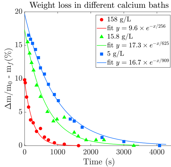
Figure 5.7 Weight loss measurements on 3 mm beads in baths of concentration [\text{Ca}^{2+}] = (158 \text{ g/L}, 15.8 \text{ g/L}, 5 \text{ g/L}) . In order to fit the data points with an exponential law, we shift all the data up to positive values. To do so, we plot the relative weight loss \frac{m-m_0}{m_0} - m_f , where m_0 and m_f are the initial and final bead weight respectively.
