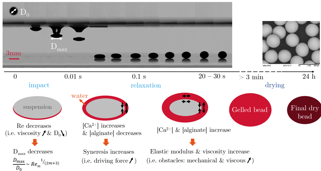
Figure 6.1 Summary of the key parameters at each step of the drip-casting process.
