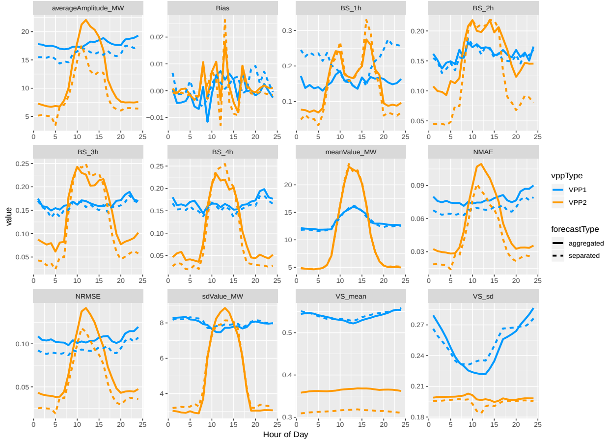
Figure 2.29: Properties and scores of scenarios generated with Gaussian Copula, directly aggregated from the DG method ("aggregated", solid line) and indirectly aggregated by separate production forecast from the IG method ("separated", dashed-line). Starting at top-left: average Amplitude of the scenario set, in MW; average bias of scenarios, scaled by installed capacity; Brier Score for ramps on several intervals, from 1 hour to 4 hours; mean value of scenarios, in MW; Normalized Mean Average Error of scenarios (NMAE), scaled by installed capacity; Normalized Root Mean Square Error of scenarios (NMRSE), scaled by installed capacity; standard deviation of the scenarios, in MW; mean value of the Variogram Score with moment = 0.5; standard deviation of the Variogram Score with moment = 0.5
