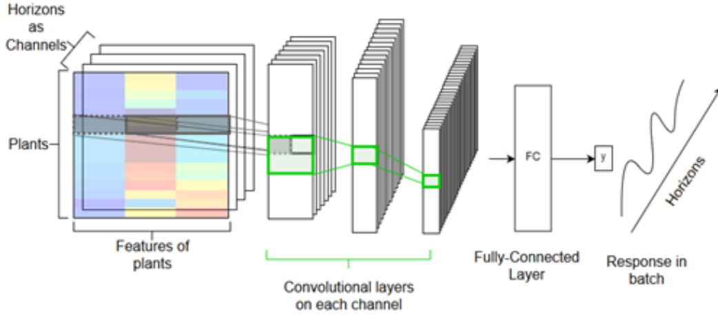
Figure 2.8: Overview of a CNN model for the multiple quantile regression of aggregated VRE production
