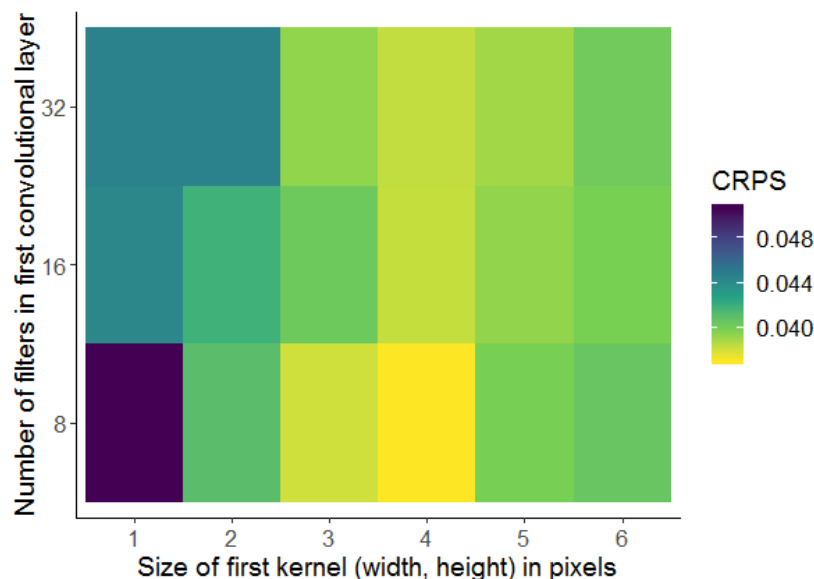
Figure 2.22: Grid search of CNN parameters: CRPS on wind aggregated production as a function of number of filters in first convolutional layer and size of first kernel. For reference, QRF has CRPS = 0.045
