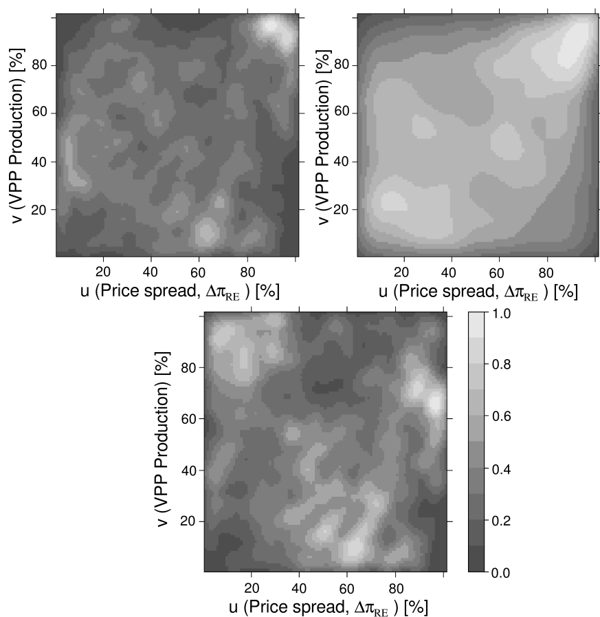
Figure 4.17: Copula modelling dependence between VPP production and price spread between aFRR and energy, (top left) 75% capacity from Wind, KDE Copula, (top right) 75% capacity from Wind, by Joe-Frank copula (1.39,0.95) (top right), (bottom) 75% capacity from PV, by KDE Copula
