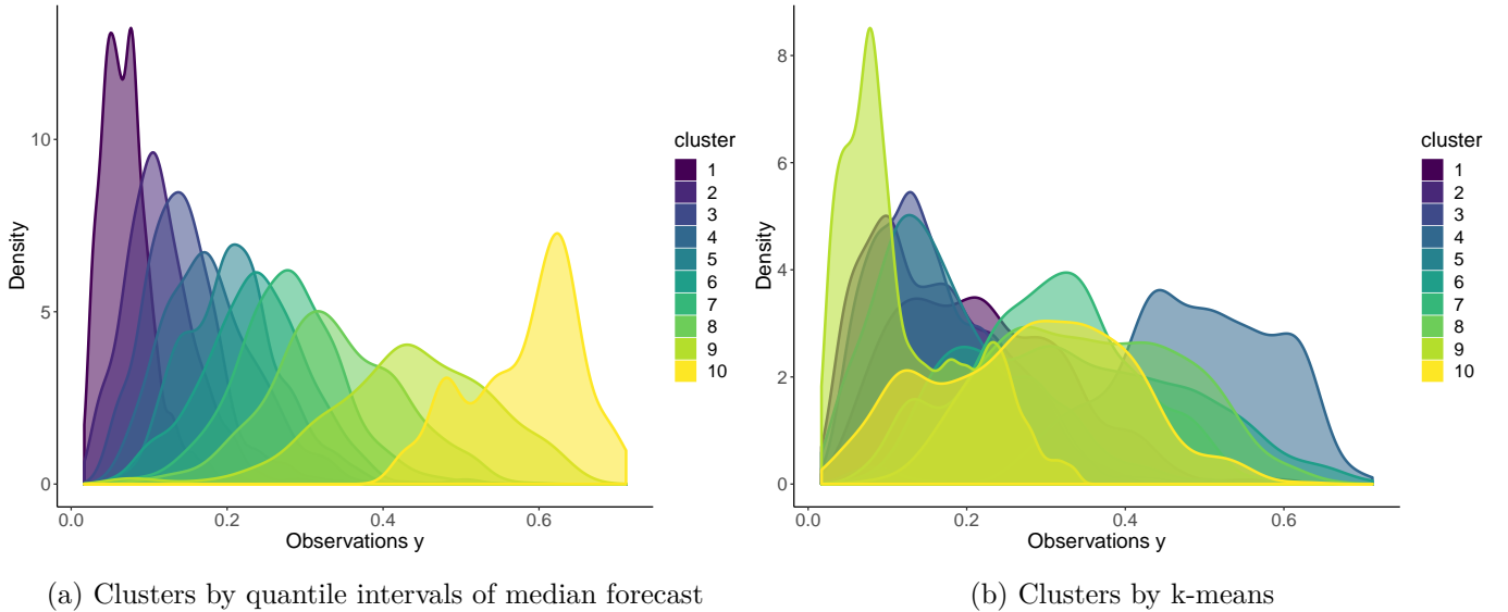
Figure 3.7: Distribution of clustered observations for two clusterization methods, for 10 clusters in each methods.
