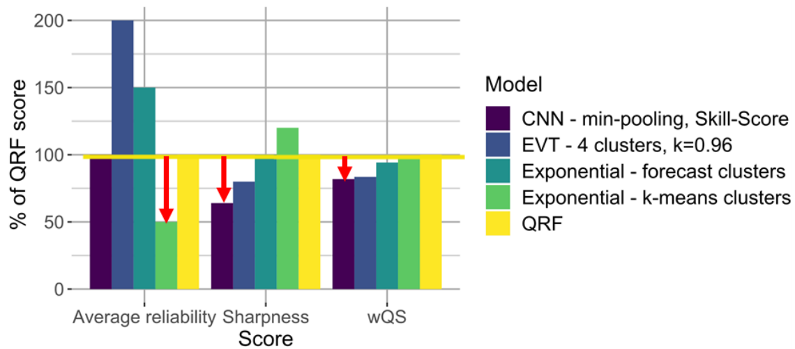
Figure 3.19: Summary of results for best models for forecasting extremes of aggregated VRE production, in terms of average reliability, sharpness on the [0.1\%-0.9\%] interval, and wQS. Scores are scaled with reference to the QRF. VPP1.
