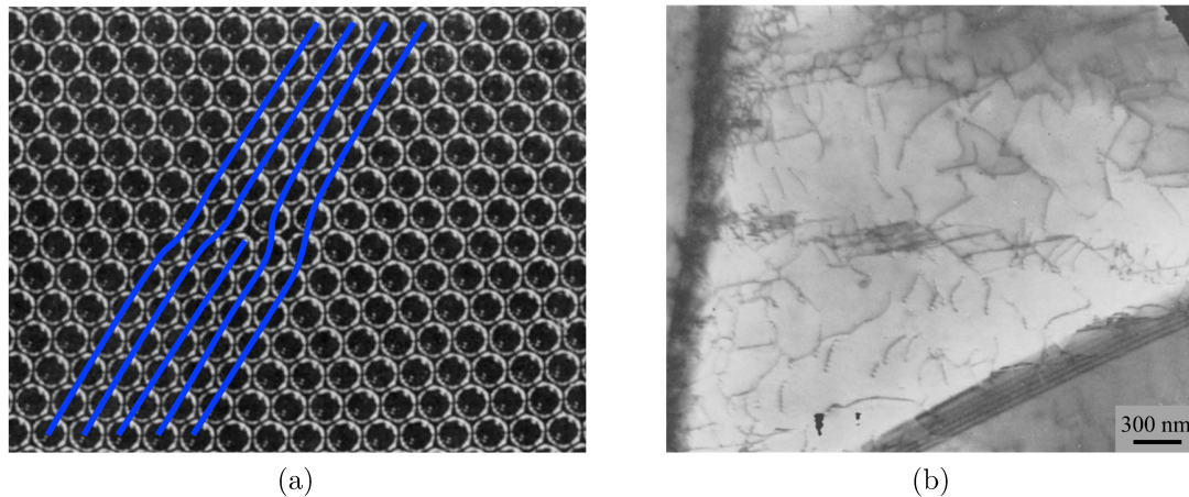
Figure 2.4 (a) Bubble raft illustration of the concept of dislocation. The bubbles diameter is 1.9 mm (Bragg and Nye, 1947). (b) Transmission electron micrograph of dislocations in a rolled stainless steel (Whelan et al., 1957).
