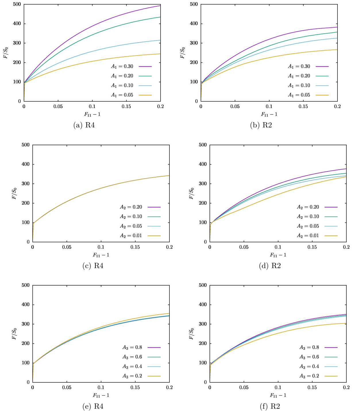
Figure D.1 Sensitivity analysis to the parameters A_1 , A_2 and A_3 for orientations R4 in (a,c,e) and R2 in (b,d,f) (The other simulation parameters were assigned the values given in Table 3.3 from Ling (2017))
