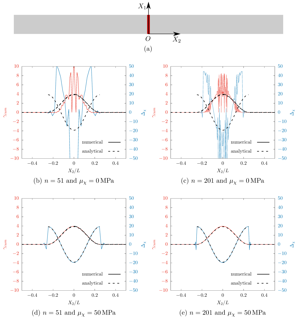
Figure 5.1 (a) Geometry of the periodic bar. (b-e) Analytical (dashed black lines) and numerical (solid blue and red lines) solutions of accumulated plastic slip \gamma_\chi (red) and Laplacian term \Delta_\chi (blue) along a periodic strip in simple shear for a linear softening behaviour (For interpretation of the references to color in this figure caption, the reader is referred to the web version of this paper).
