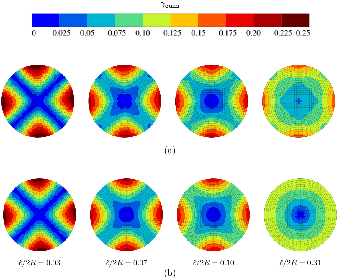
Figure 5.8 Cumulative plastic strain distribution in FCC single crystal for \langle 001 \rangle crystal orientation for different values of ratio l/2R_0 using (a) micromorphic (b) Lagrange multiplier models at surface strain of 0.08 (fields reported on the reference configuration).
