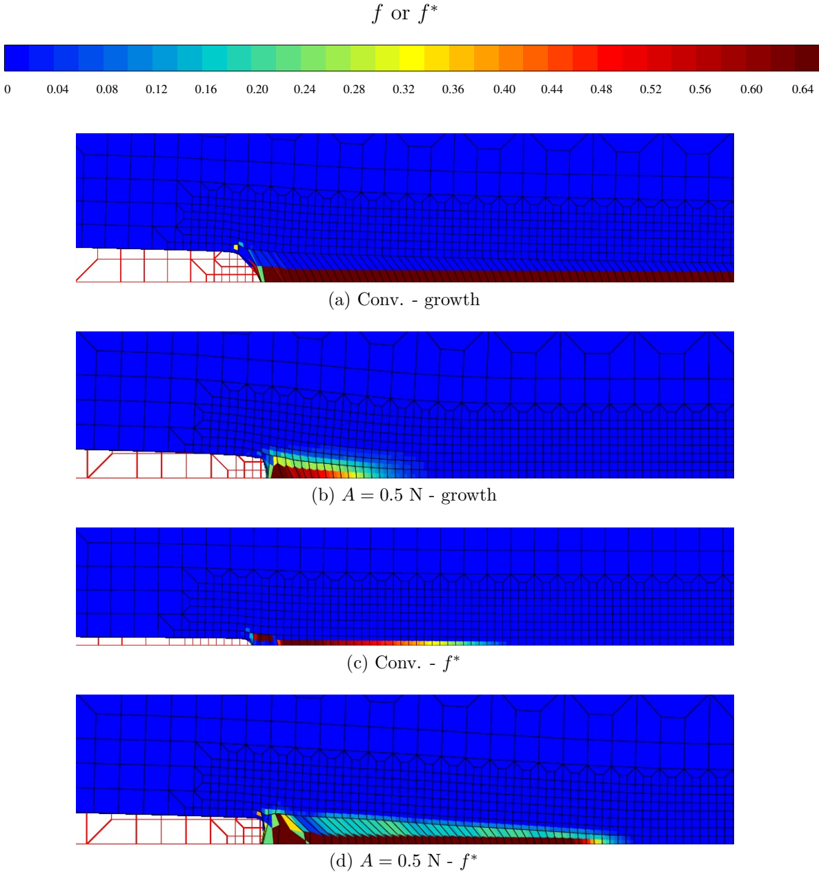
Figure 6.14 Porosity fields in the vicinity of the CT specimen notch front, i.e. close to X_1 = a_0 at CMOD=2mm in (a), (b) and (d). The last computed time step is used in (c). Initial (undeformed) mesh is displayed in solid red lines.
