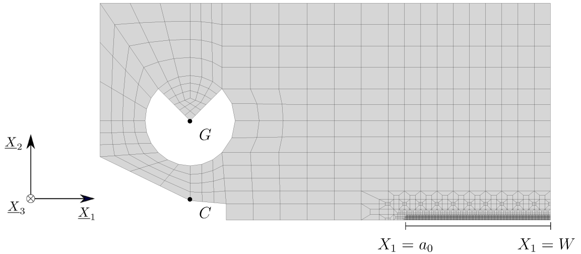
Figure 6.13 Finite element mesh of a half CT specimen geometry.
