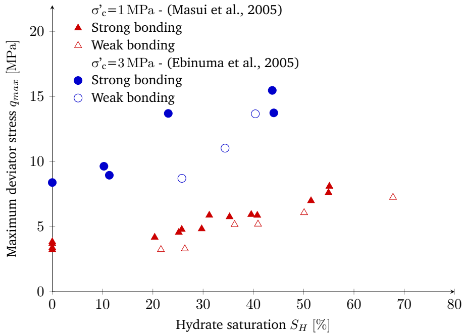
Fig. 2.18: Effect of the pore habit of methane hydrates, at fixed temperature ( 5^\circ\text{C} ), on the strength of Toyoura sand samples at 1 MPa (Masui et al., 2005) and 3 MPa (Ebinuma et al., 2005) of confining pressure (after Soga et al., 2006).
