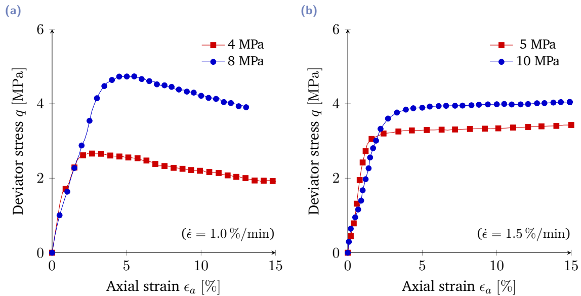
Fig. 2.4: Results of triaxial tests at -5 °C and different confining pressures on pure methane hydrate samples performed by (a) Hyodo et al. (2002) at a strain rate of 1.0 %/min and by Yu et al. (2011b) at 1.5 %/min.
