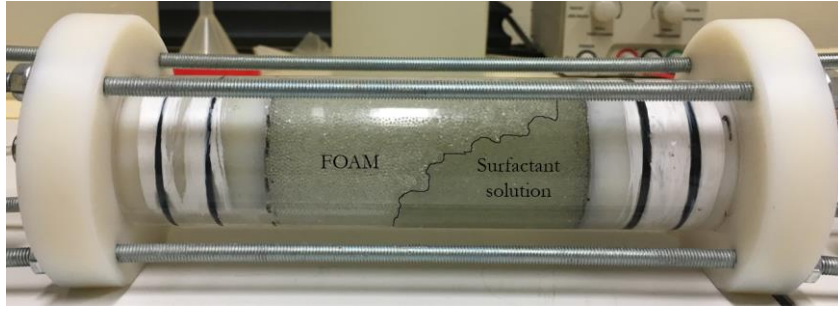
Fig. 2.6 In situ foam generation in foam generator column (after 0.6 PV injection):
