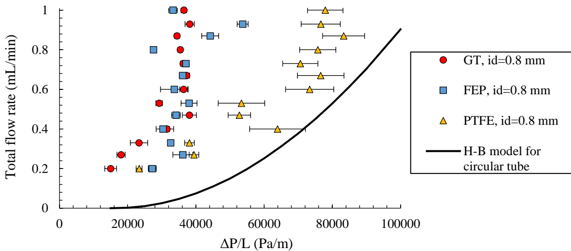
Fig. 4.15 Total flow rate as a function of the pressure loss per unit length for GT, FEP, PTFE tubes with the id of 0.8 mm and the analytical solution for the yield stress fluid ( f_g=85\% )
