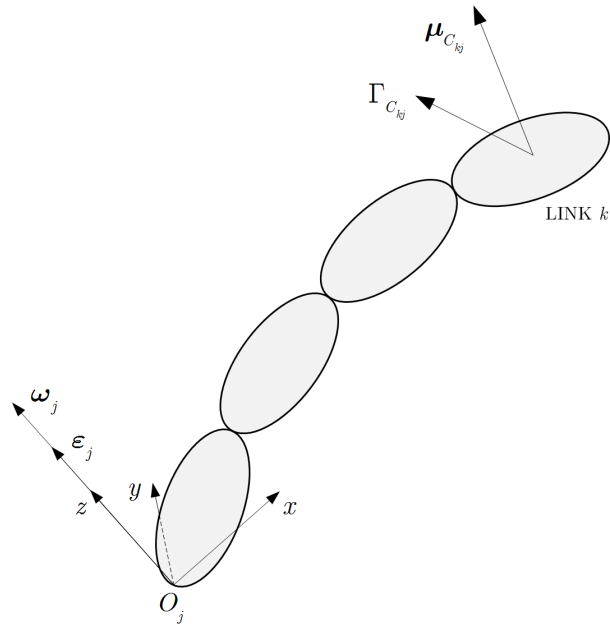
Figure 5.1: Inertial moment \boldsymbol{\mu}_{C_{kj}} and linear acceleration \boldsymbol{\Gamma}_{C_{kj}} of center of mass of link k transferred by frame. j
