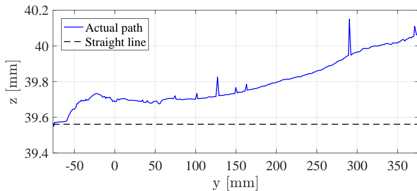
Figure 4.31: Actual path in zy plane.
