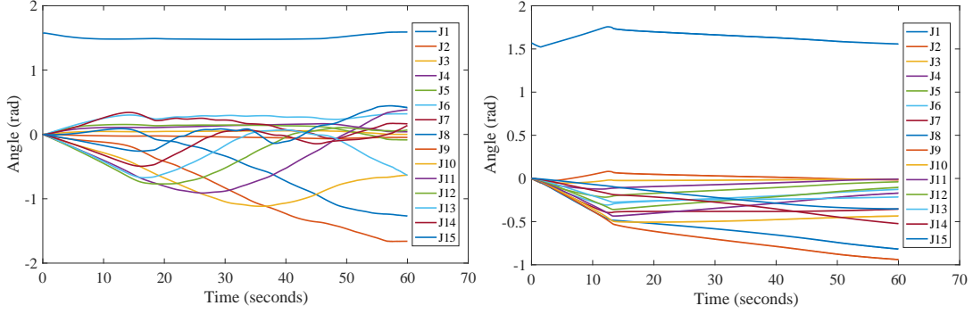
Figure 3.25: Test 1: joint angles, Newton method (left), gradient method (right).
