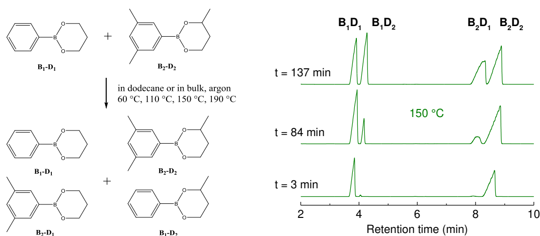
Figure 3.16. Left side: Metathesis of highly pure dioxaborinanes \text{B}_1\text{D}_1 and \text{B}_2\text{D}_2 at different temperatures under argon protective atmosphere. Right side: Gas chromatography traces of the reaction medium after 3 min (bottom), 84 min (middle) and 137 min (top) during the exchange at 150 °C.
