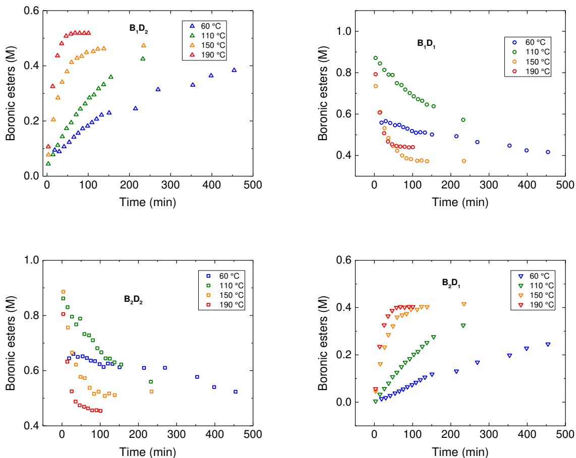
Figure 3.17. Kinetic plots of the exchange reaction between boronic esters B_1D_1 and B_2D_2 in dodecane at different temperatures and under argon protective atmosphere.
