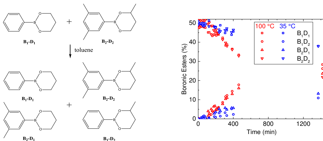
Figure 9. Exchange between \mathbf{B}_1\mathbf{D}_1 and \mathbf{B}_2\mathbf{D}_2 under air in toluene at 100 °C (red) and 35 °C (blue).
