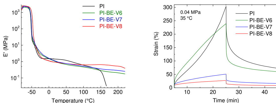
Figure 5.20. Left: Storage modulus of PI, PI-BE-V6 , PI-BE-V7 and PI-BE-V8 , measured by DMA between -75 ^{\circ}\text{C} and 220 ^{\circ}\text{C} . Right: Creep experiment at 35 ^{\circ}\text{C} and 40 000 Pa for PI, PI-BE-V6 , PI-BE-V7 and PI-BE-V8 .
