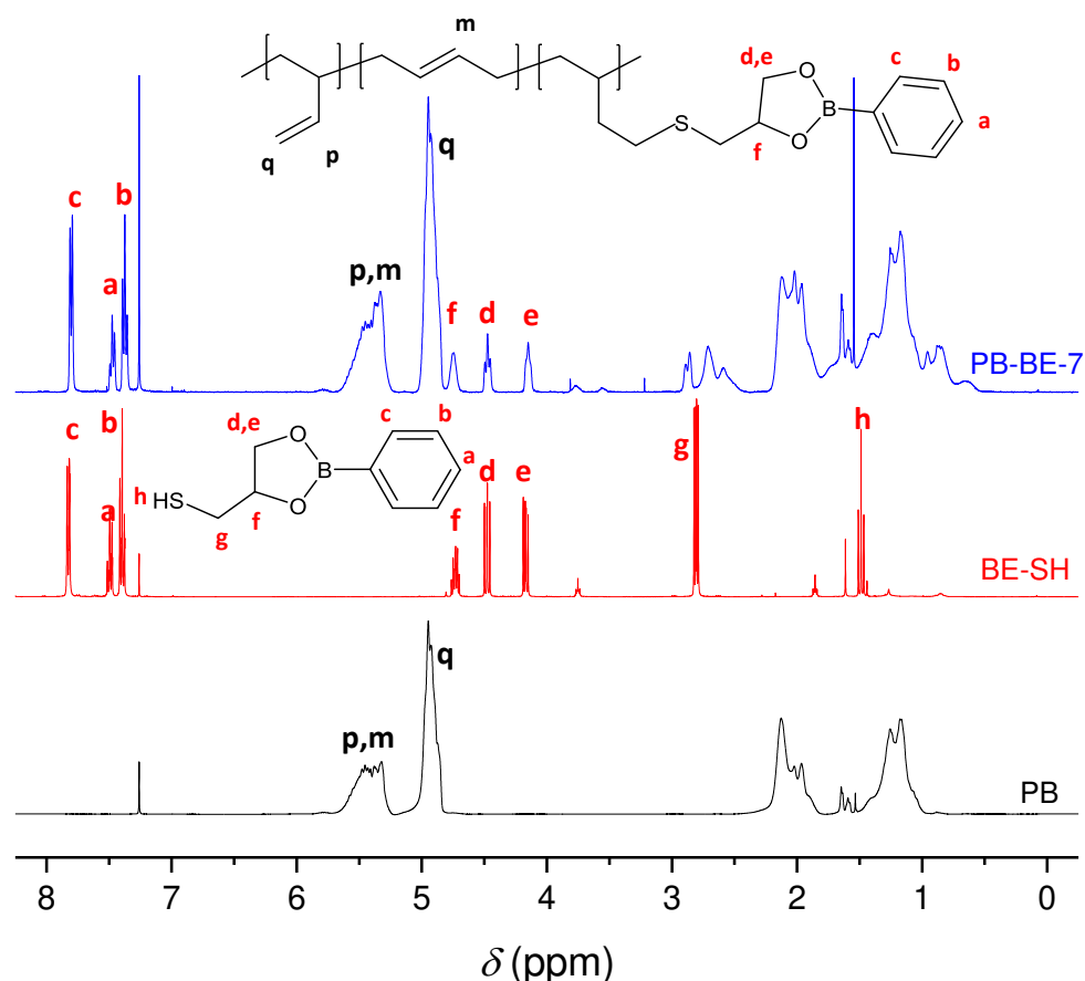
Figure 2.2. ^1\text{H-NMR} spectra in \text{CDCl}_3 of PB-BE-7 after purification by precipitation into anhydrous methanol (grafting yield = 89%, f = 9\% ) (top, blue), BE-SH (middle, red), and the starting neat PB (bottom, black).
