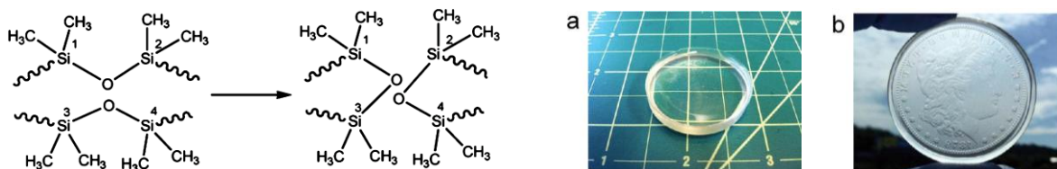
Figure 1.14. Left: Siloxane exchange. Right: (a) Disc-shape sample and (b) remolded with a silver dollar. 109
