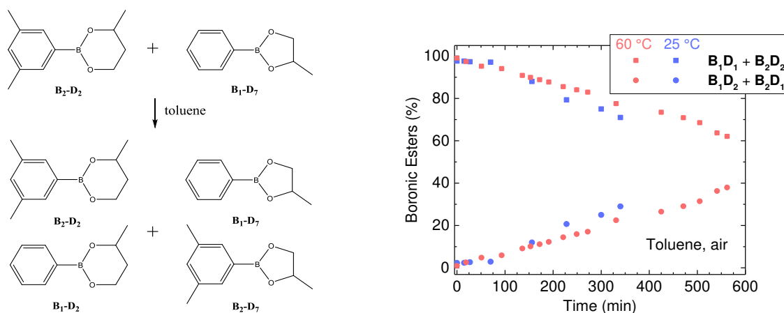
Figure 3.10. Exchange between dioxaborolane B_1D_7 and dioxaborinane B_2D_2 under air in toluene at 60 °C (red) and 25 °C (blue).
