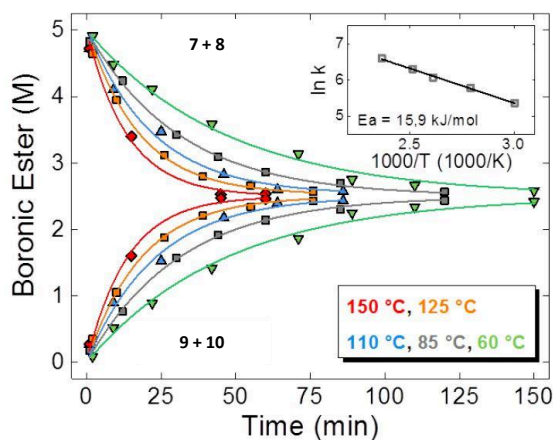
Figure 3.1. Kinetic data of the metathesis of dioxaborolanes 7 and 8 in bulk under argon protective atmosphere (adapted from reference 89 ).
