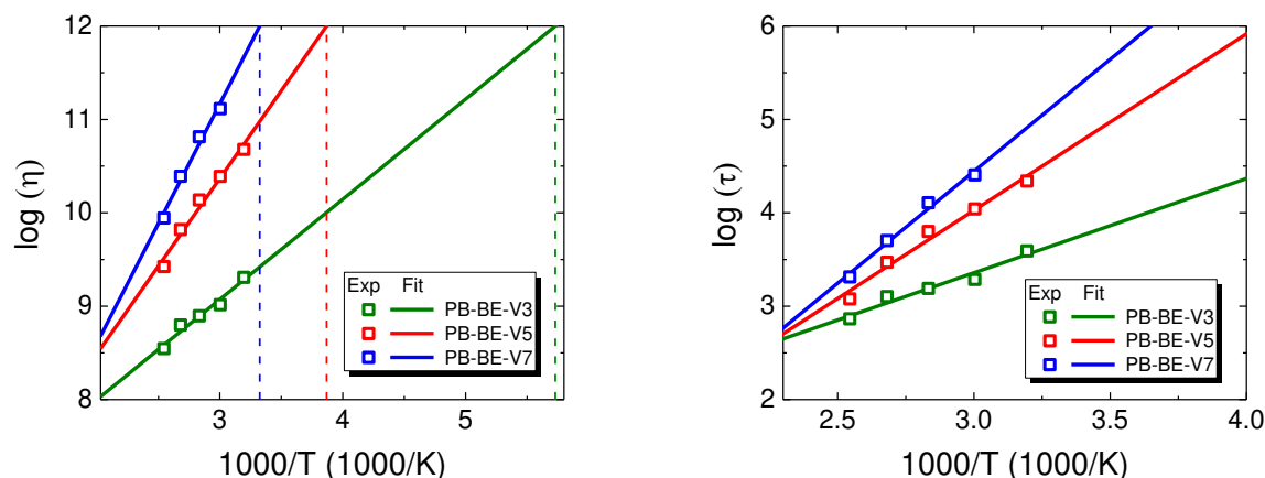
Figure 2.15. Plots of \log(\eta) (left) and \log(\tau) (right) versus 1000/T for PB-BE-V3 (green), PB-BE-V5 (red) and PB-BE-V7 (blue) experimental points (squares) and linear fits (solid lines) to extract the activation energy from the slope and T_v from the abscissa at which \log(\eta) = 12 (dashed lines). Viscosities were extracted from stress step-stress creep data with Equation 2.1 . Relaxation times were extracted from step-stress creep data with Equation 2.2 .
