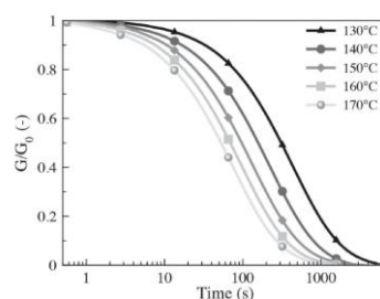
Figure 1.21. Left: Exchange reaction of model compounds for kinetic studies. Right: Normalized stress relaxation at different temperatures. 127
