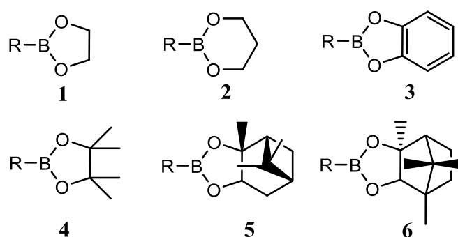
Scheme 3.5. Some common boronic esters.
