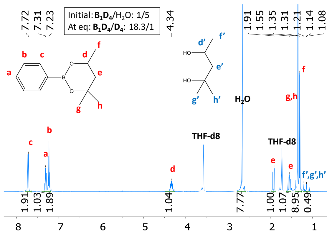
Figure 3.6. ^1\text{H} -NMR in THF- \text{d}_8 of \text{B}_1\text{D}_4 and \text{D}_4 after hydrolysis reaction with an initial ratio \text{B}_1\text{D}_4/\text{H}_2\text{O} : 1/5.
