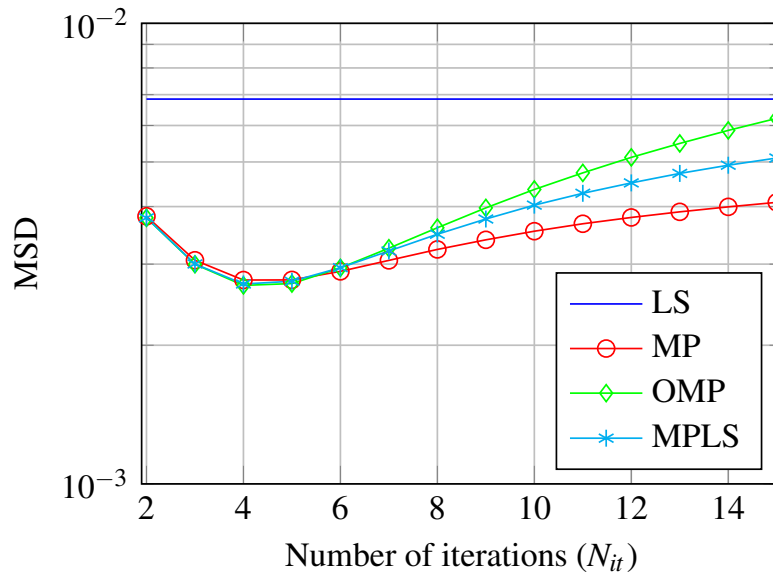
Figure 5.7 – MSD vs N_{it} for M = 40 and wideband HF Channel B.
