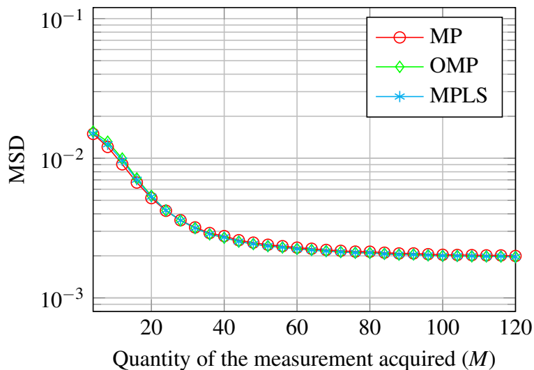
Figure 5.8 – MSD vs M for S = 4 and Wideband HF Channel B.
