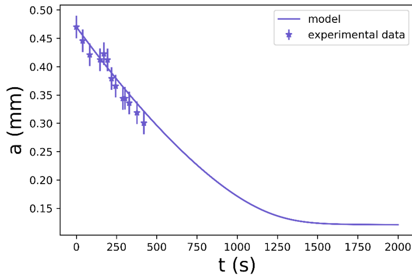
Figure 4.4: Numerical and experimental results of a bubble, which was immersed in an R-1.0 glass melt, to demonstrate the studied region for \sim 10 min.
