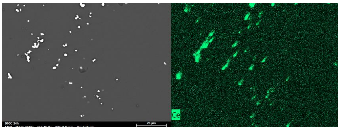
Figure 5.10: Scanning electron microscopic (SEM) image showing an example of region with non-incorporated cerium-IV oxide ( \text{CeO}_2 ) for the sample 900 °C 24h.
