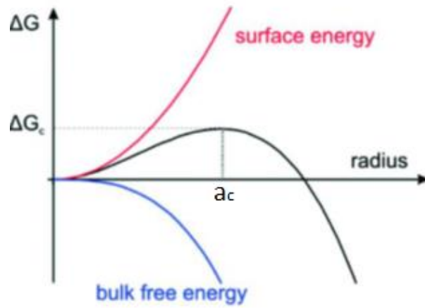
Figure 2.4: Energy balance versus radius development for nucleation.
