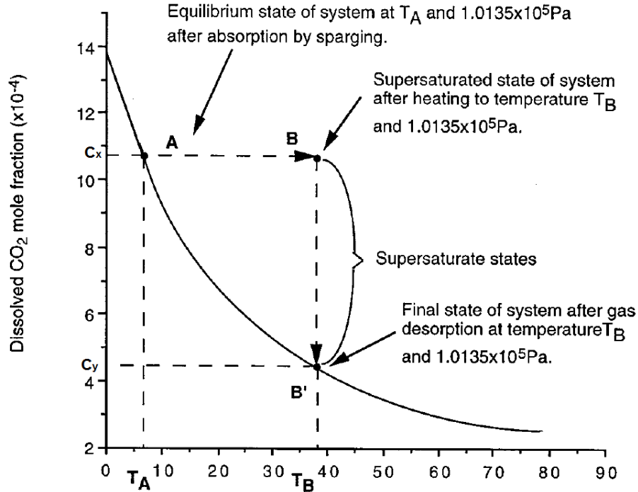
Figure 2.2: \text{CO}_2 solubility in water as function of the temperature at 1.013 \times 10^5 \text{ Pa} . 36
