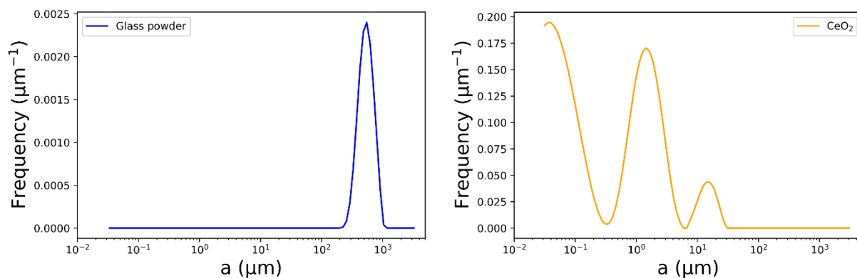
Figure 3.1: PSD for borosilicate glass and \text{CeO}_2 powders obtained by laser granulometry.
