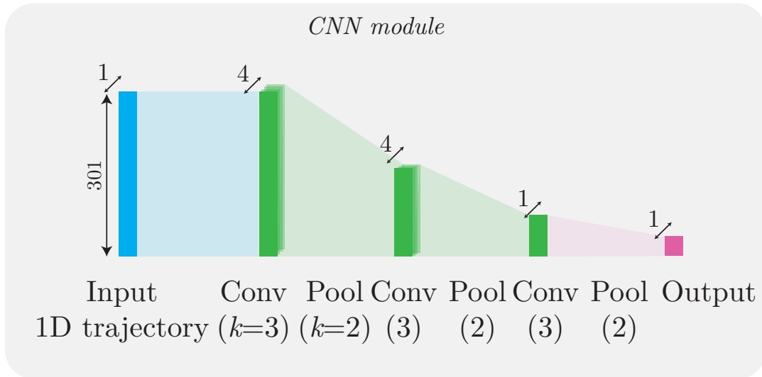
Figure 3.4 – Vehicle Control: CNN Module
