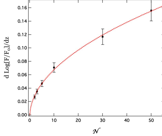
Figure 4.2 – Rate of the exponential increase of the resistive force d \log(F)/dz againsts the chain's length \mathcal{N} . The red dashed curve corresponds to the best power law fit \sim \mathcal{N}^{0.46} .
