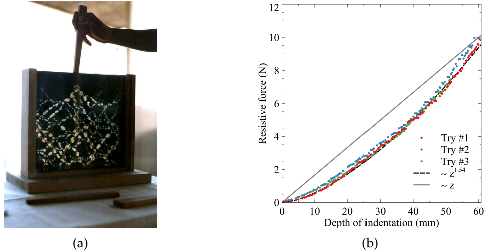
Figure 2.5 – (a) Force chains are visible thanks to the photoelasticity of the grain material [3]. (b) Measured resistive force against depth of indentation for unconnected beads.
