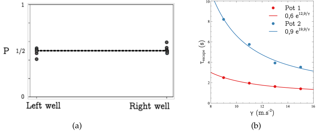
Figure 6.8 – (a) Probability for the bead to be located in the right or the left well. The black dashed line corresponds to the probability 1/2 . (b) Mean escape time from a well. The solid lines are best fits to a \cdot \exp(b/\gamma) .
