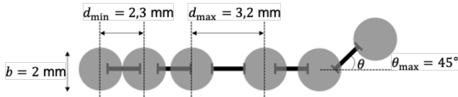
Figure 2.2 – Modelisation of the granular chain.
