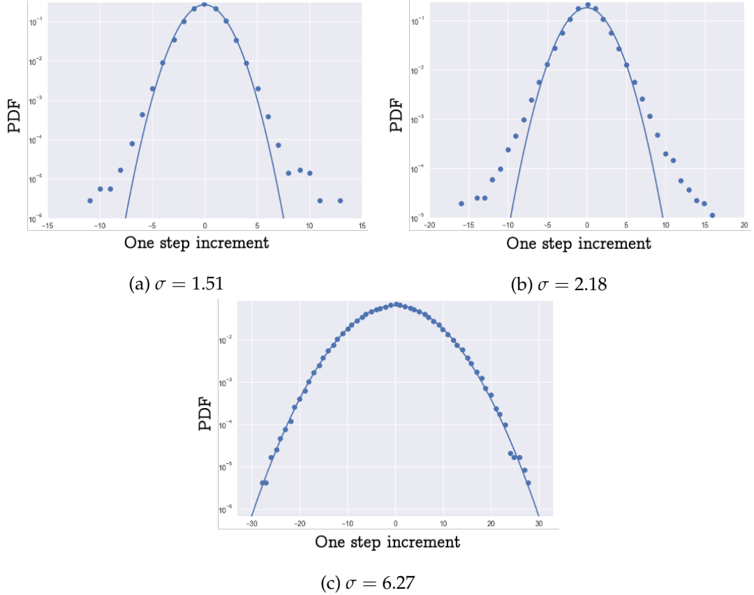
Figure 5.7 – Probability density function (PDF) of the one step increment \Delta x for different solvent bath (a) small plastic beads (b) dimers (c) glued beads. The solid blue lines represent a Gaussian fit with \sigma as the standard deviation of the distribution.
